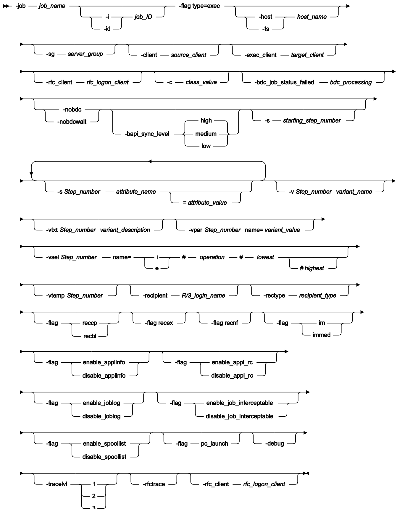
Figure 21. Job definition syntax
