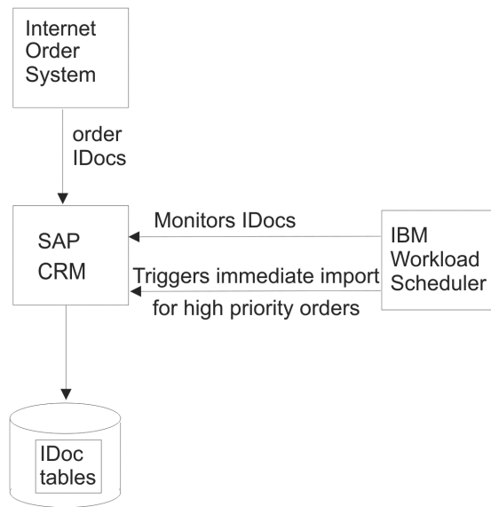
Figure 29. Managing high priority IDocs overview
