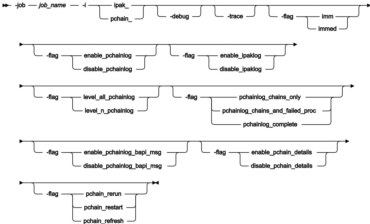
Figure 24. Job definition syntax
