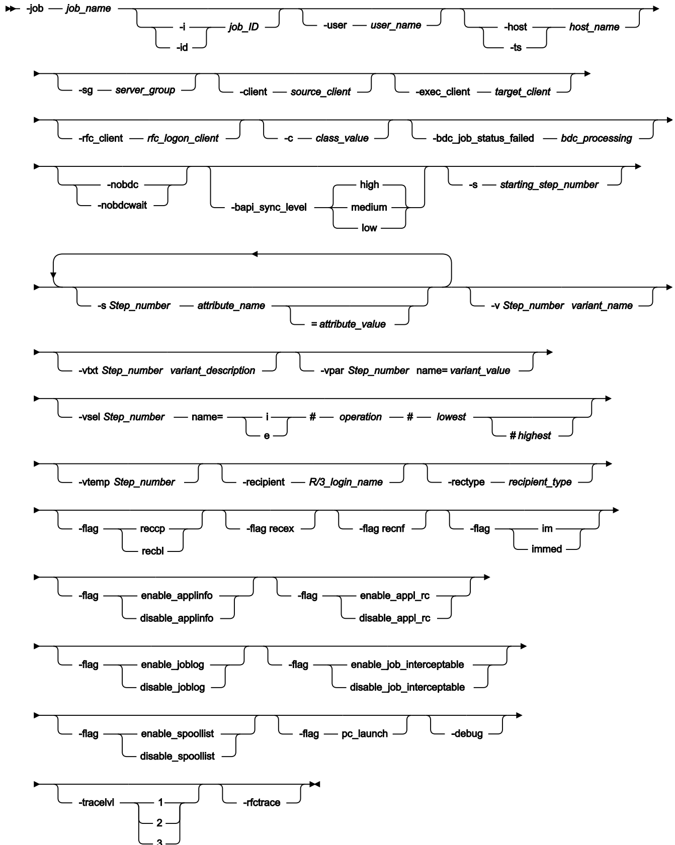
Figure 19. Job definition syntax
