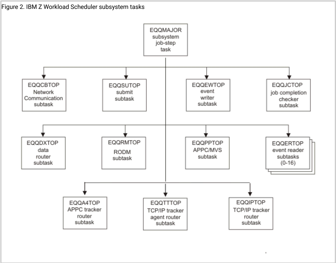
Figure 2: IBM Z Workload Scheduler subsystem tasks on page 56 shows the tasks that can be started as subtasks by the job-step task when IBM Z Workload Scheduler is installed.
