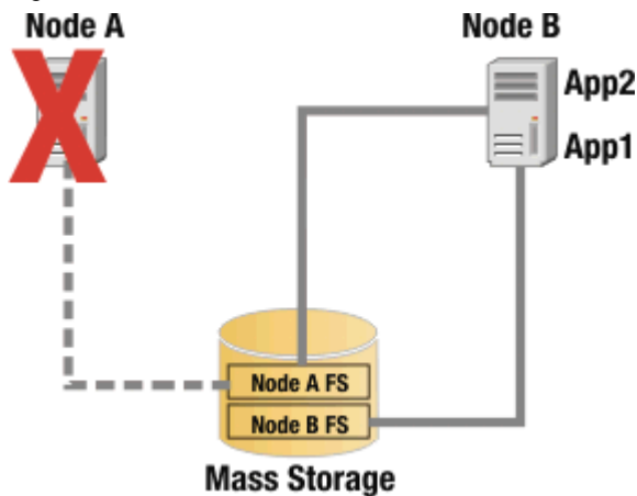
Figure 11. Failover scenario
