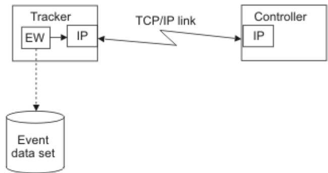
Figure 1. A z/OS system with a TCP/IP connection
