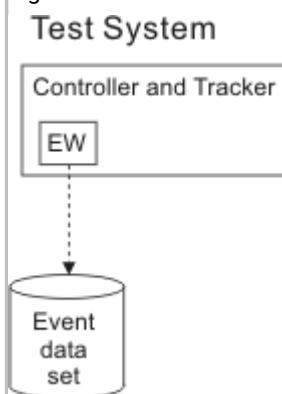
Figure 4. A tracker and controller configured in a single address space
