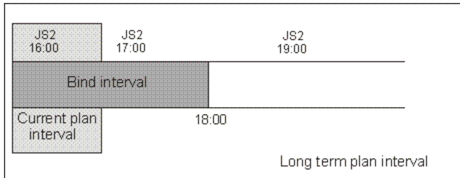
Figure 67. The instance to be bound exists but it is not yet included in the CP
