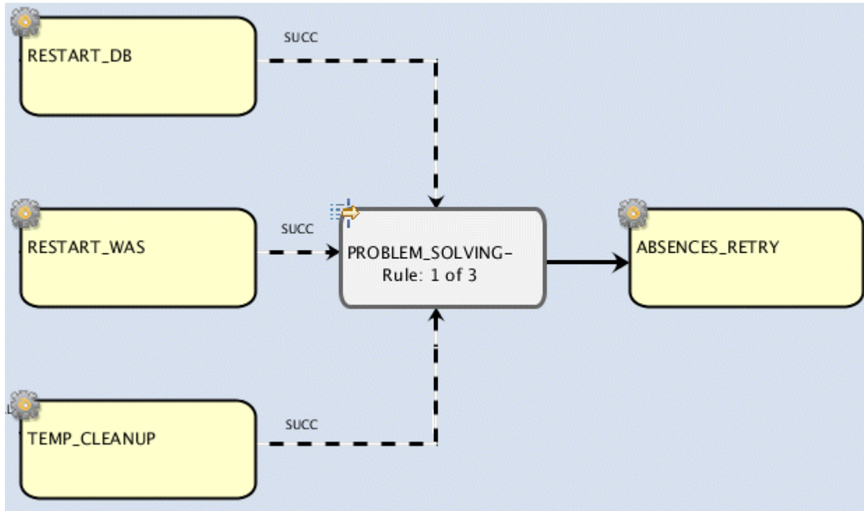
Figure 56. A join dependency containing three dependencies on SUCC status
