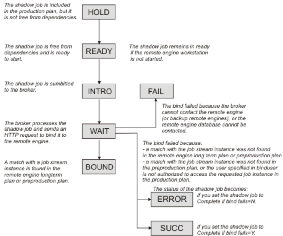
Figure 63. Shadow job status transition until the bind is established
