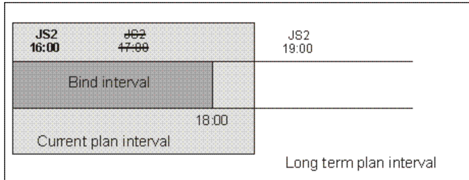
Figure 65: Instance to be bound if the instance that most closely precedes the shadow job scheduled time exists in the LTP but was canceled from the CP on page 1288 shows, highlighted in bold, the JS2 instance that is selected for the bind, because the occurrence that better matched was deleted.
