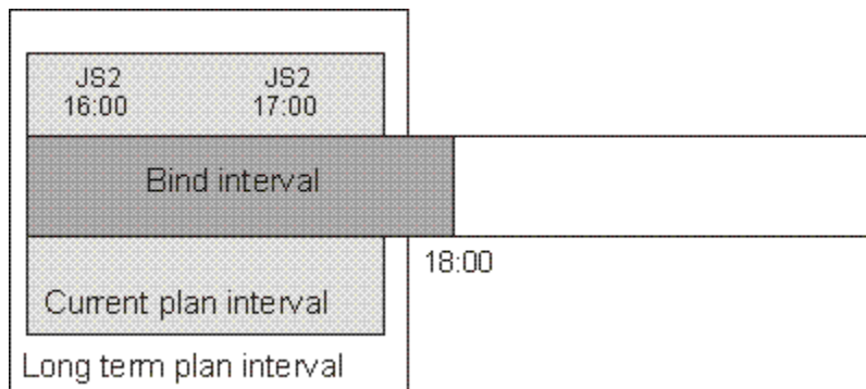
Figure 68. The LTP interval still does not contain the shadow job scheduled time
