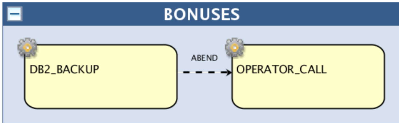
Figure 58. ABEND status conditional dependency
