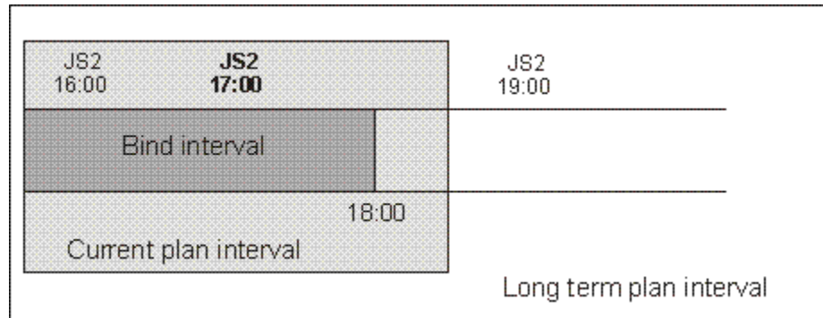
Figure 64. Instance to be bound if the shadow job scheduled time is included in the CP interval
