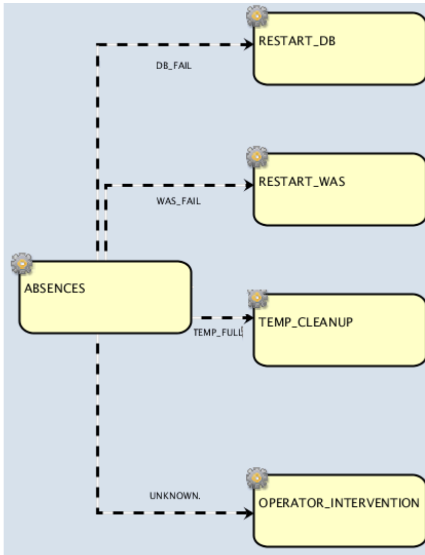
Figure 55. Conditional dependencies on output conditions on the ABSENCES job
