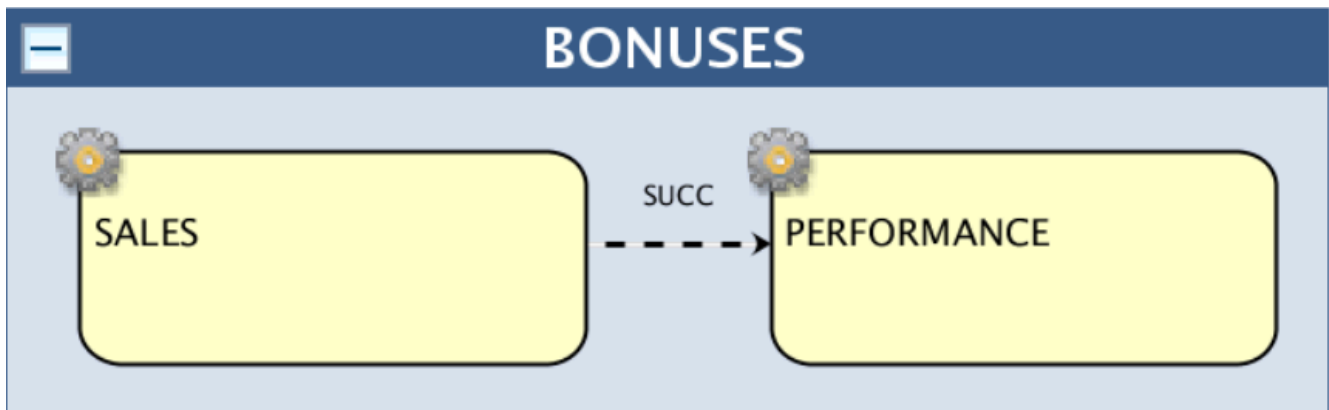
Figure 57. Status conditional dependency on a job with recovery stop setting
