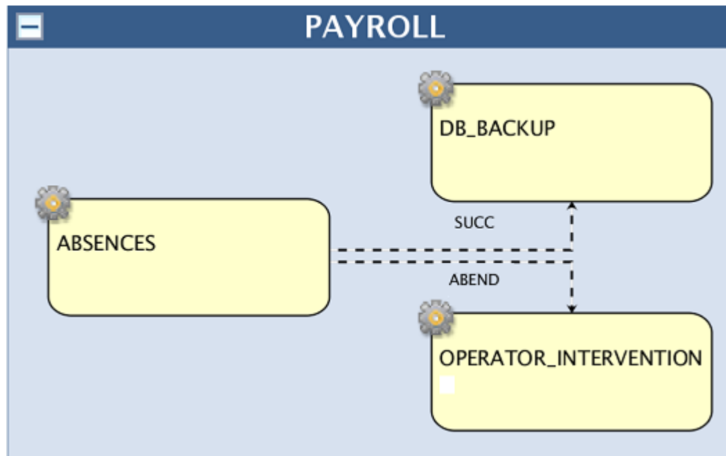
Figure 54. Two different conditional dependencies on SUCC and ABEND statuses on the ABSENCES job
