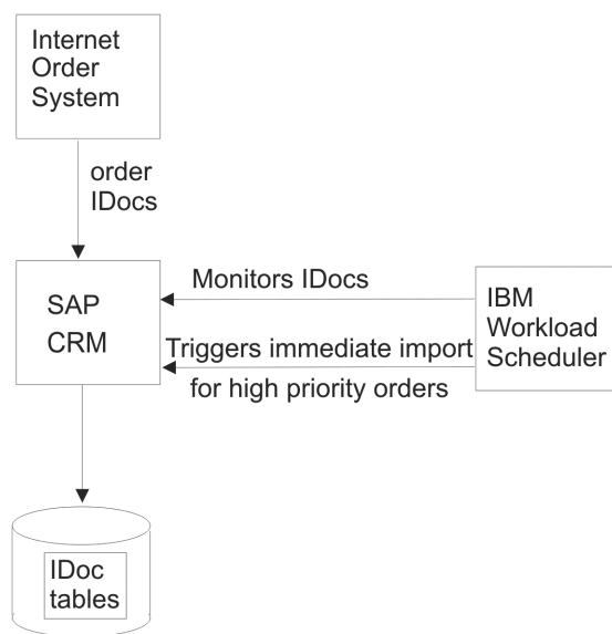
Figure 47. Managing high priority IDocs overview
