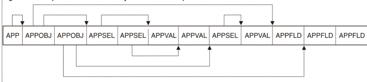
Figure 5. Example of a send buffer layout for a GET request
