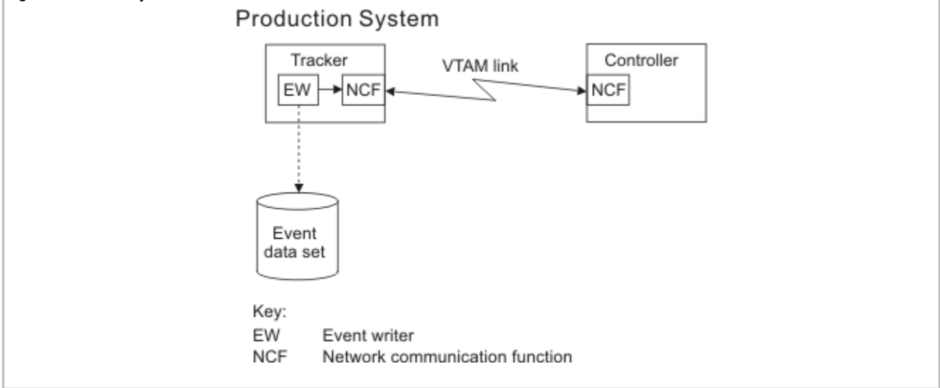
Figure 3. A z/OS system with a VTAM® connection
