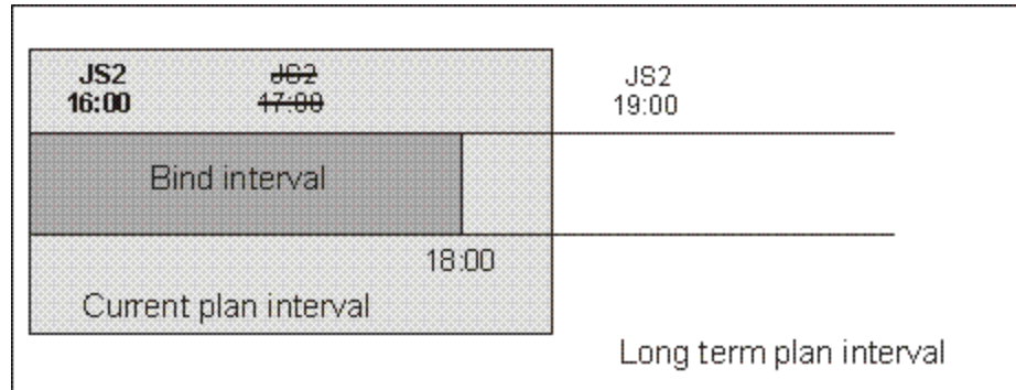
Figure 45: Instance to be bound if the instance that most closely precedes the shadow job scheduled time exists in the LTP but was canceled from the CP on page 1083 shows, highlighted in bold, the JS2 instance that is selected for the bind, because the occurrence that better matched was deleted.
