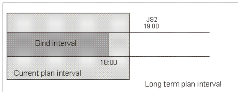
Figure 46: The scheduled time of the shadow job is included in the CP but no instance to bind exists on page 1083 shows that a JS2 instance that closely precedes the shadow job scheduled time does not exist.
