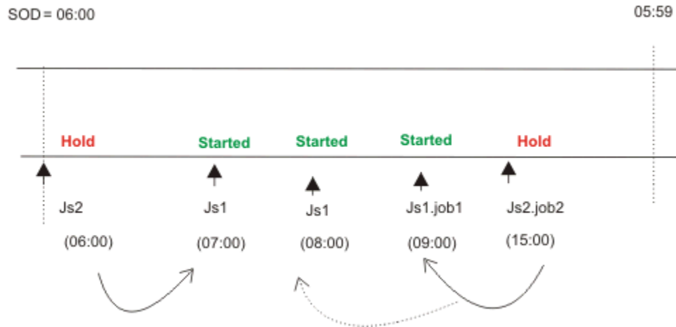
Figure 14. Sameday matching criteria - Step 2: at 9:00
