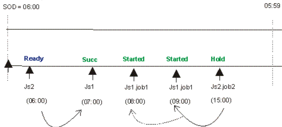
Figure 15. Sameday matching criteria - Step 3: at 15:00
