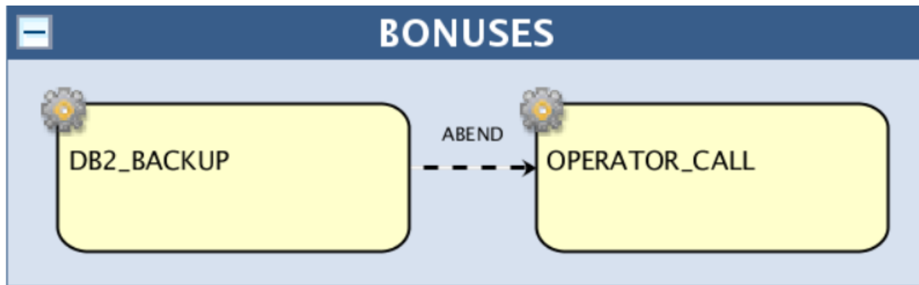
Figure 38. ABEND status conditional dependency
