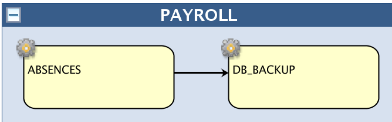
Figure 33. A follows dependency on the ABSENCES job
