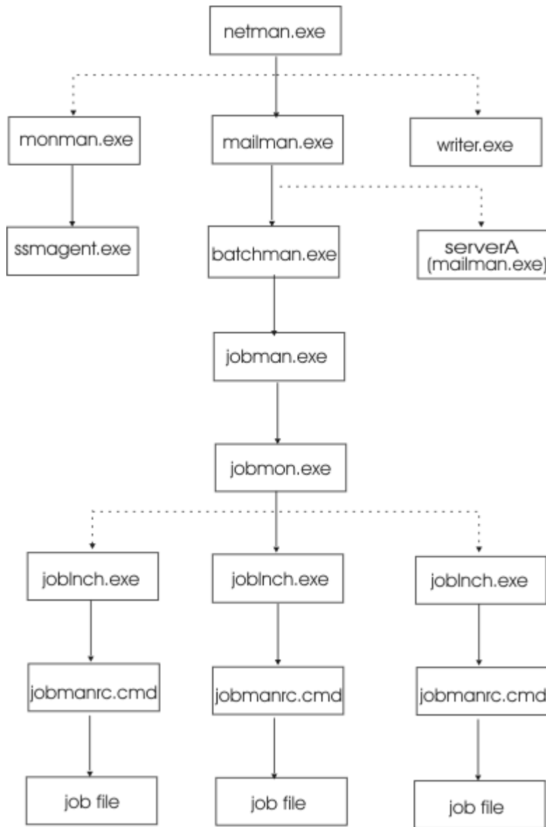
Figure 4. Process tree in Windows®
