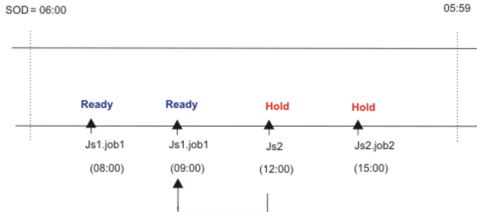
Figure 16. Closest preceding matching criteria - Step 1: before 08:00
