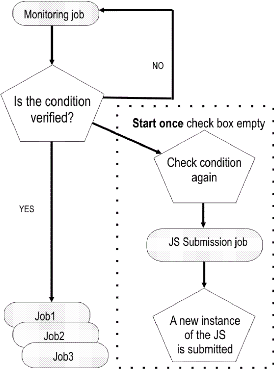
Figure 23. Condition-based workload automation
