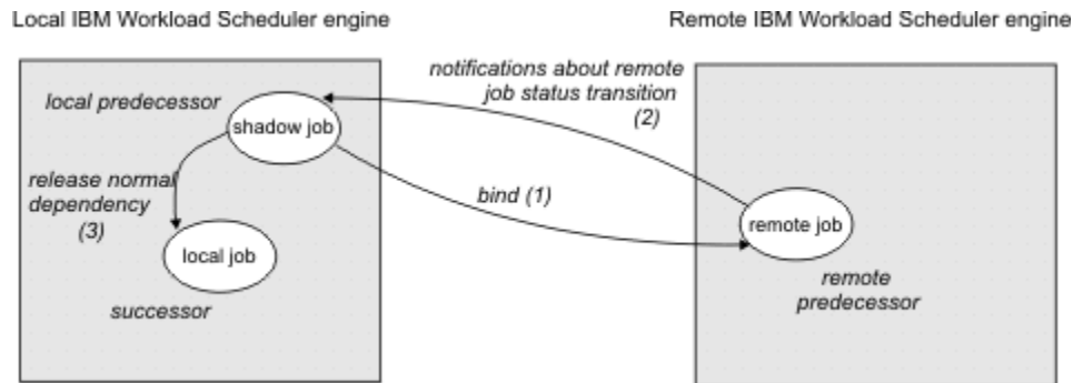
Figure 42. Cross dependency logic
