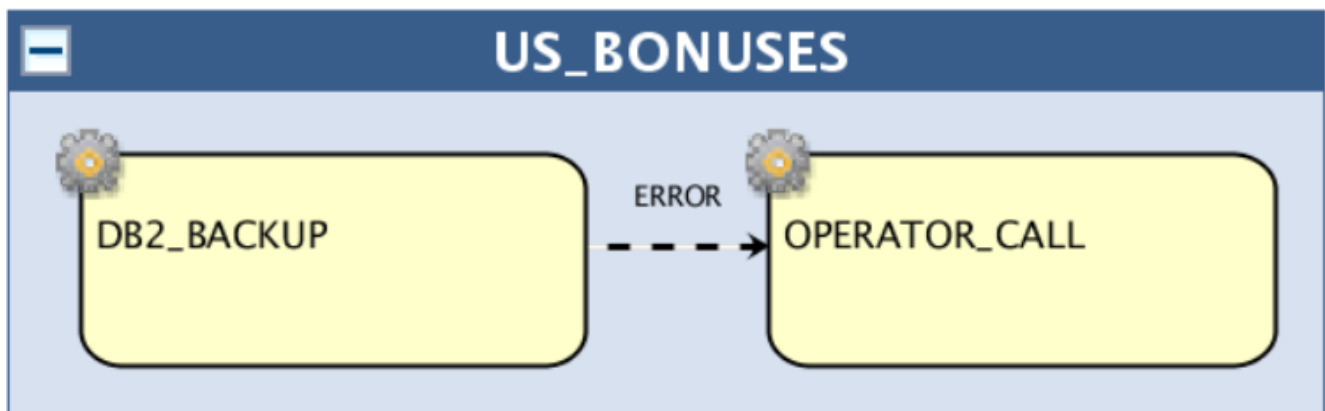
Figure 40. ERROR output condition
