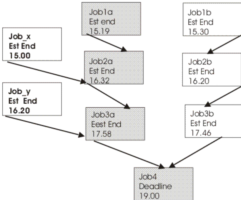
Figure 22. Critical path
