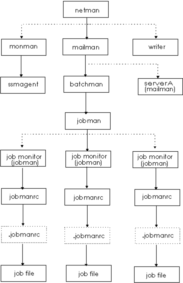
Figure 3. Process tree in UNIX®
