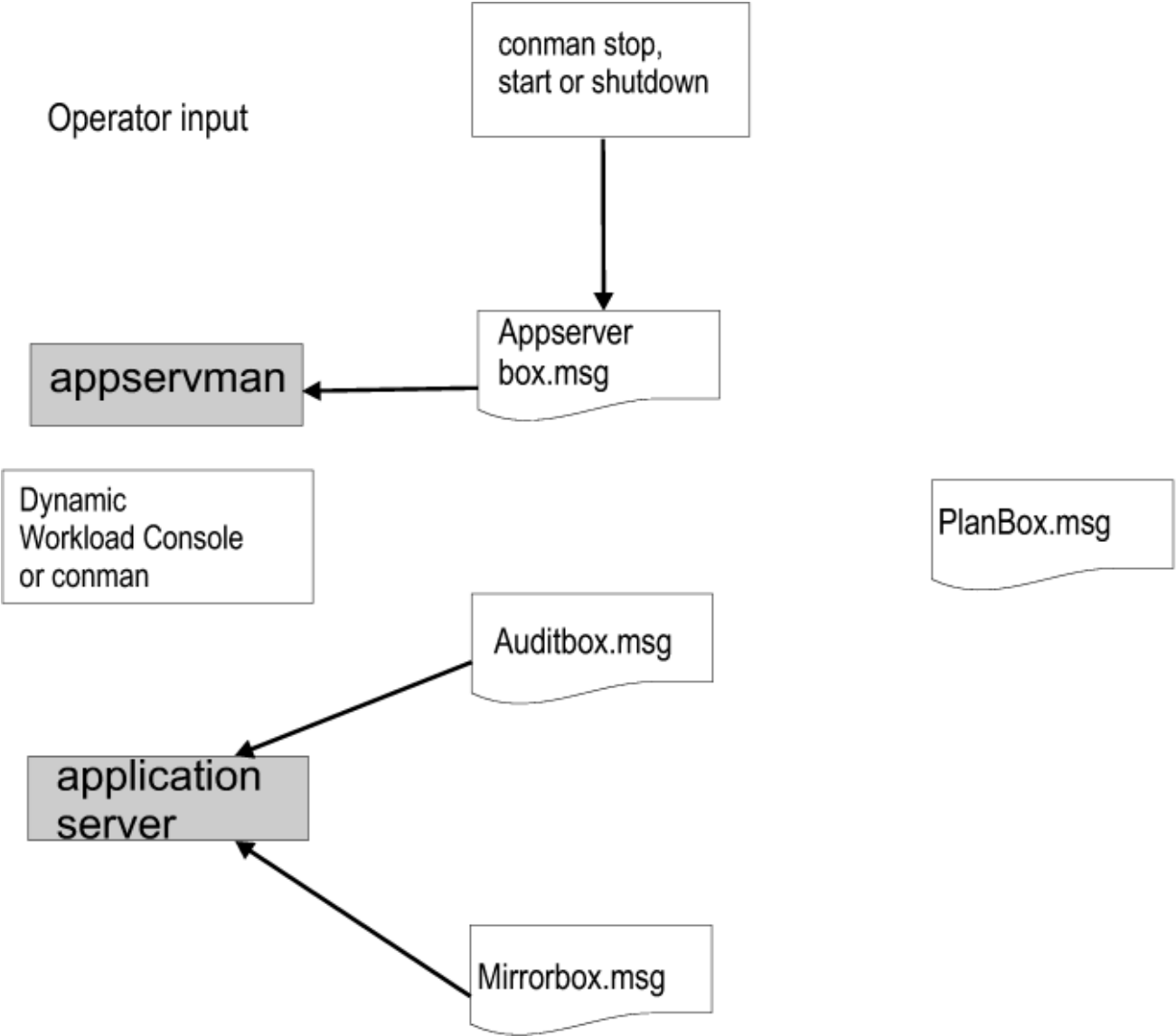
Figure 5. Inter-process communication on the master domain manager
