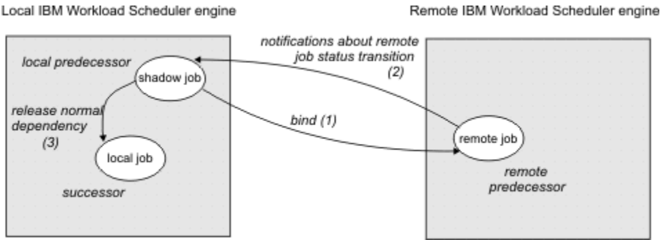
Figure 42. Cross dependency logic
