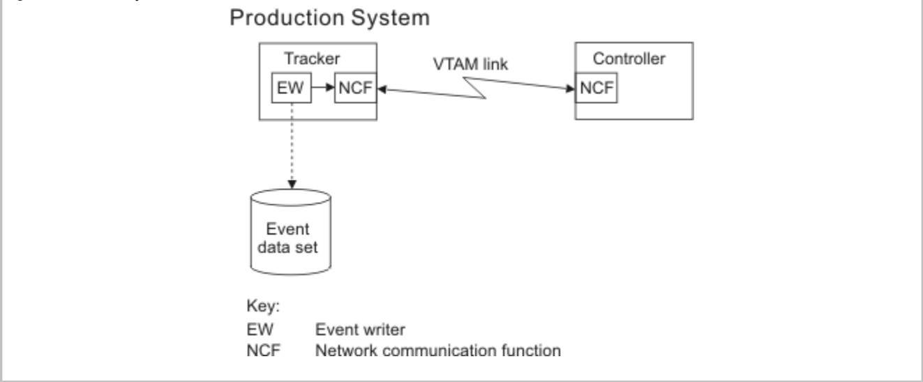
Figure 4. A z/OS system with a VTAM® connection
