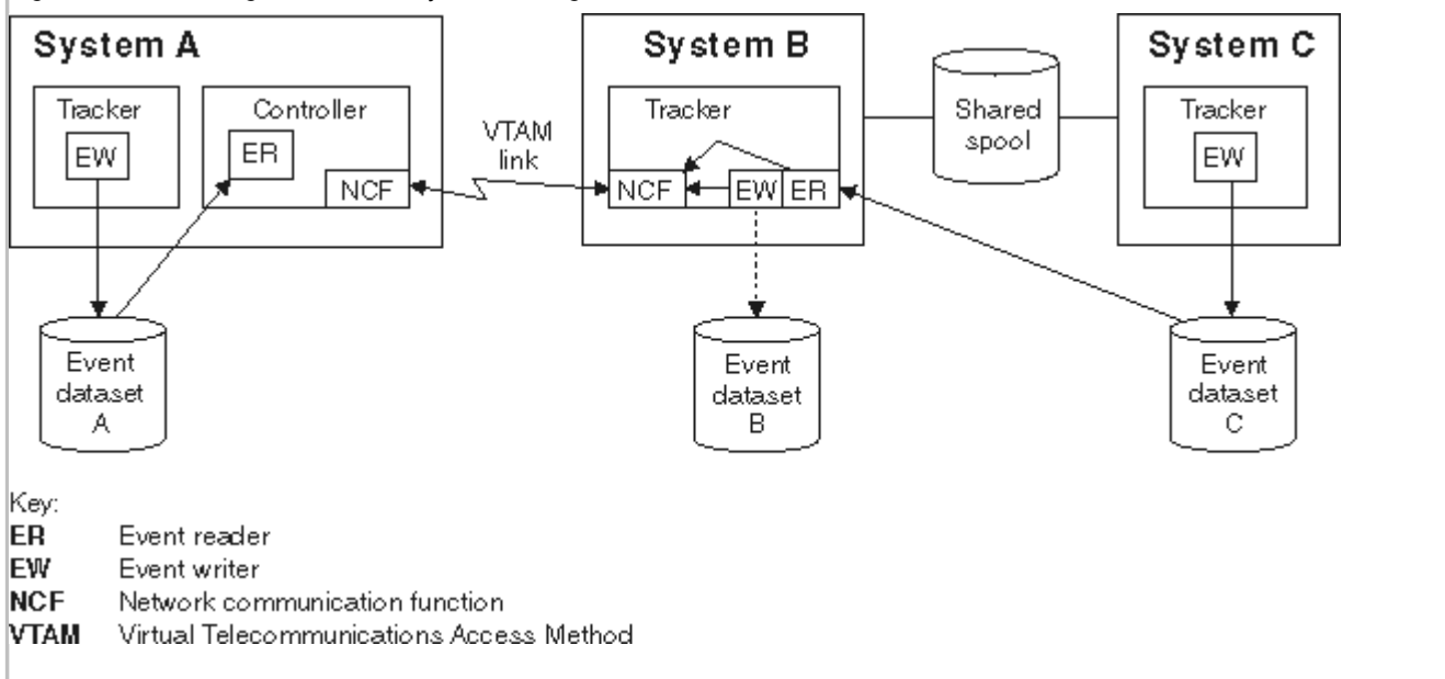
Figure 33. Controlling a JES2 MAS system through a VTAM® link
