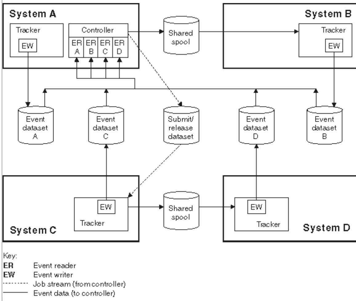
Figure 27. Two z/OS JES2 MAS complexes connected through shared DASD
