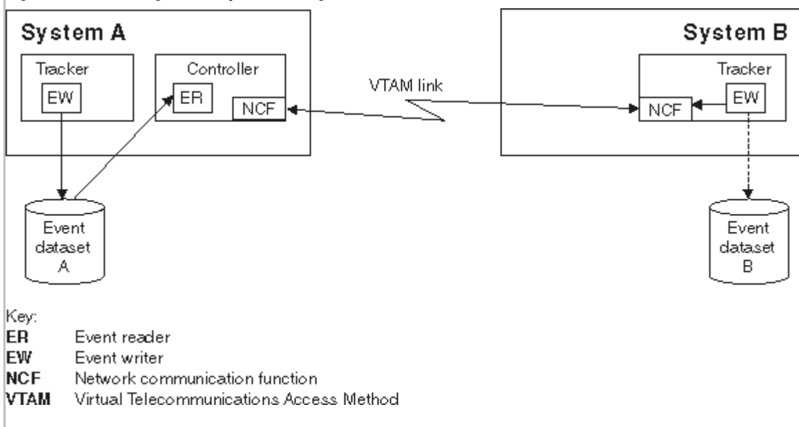
Figure 31. Controlling a z/OS system through a VTAM® link
