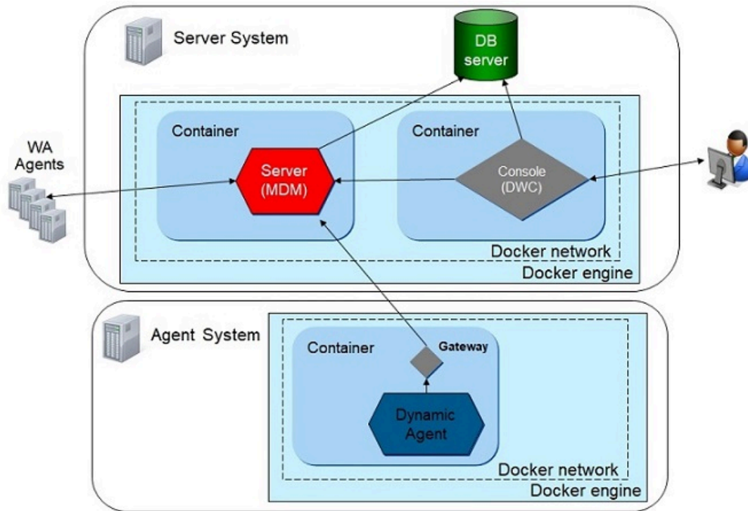
Figure 8. Dockerized environment configuration
