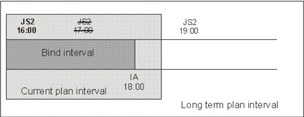
Figure 191. Instance to be bound if the instance that most closely precedes the shadow job input arrival exist in the LTP but it was canceled from the CP
