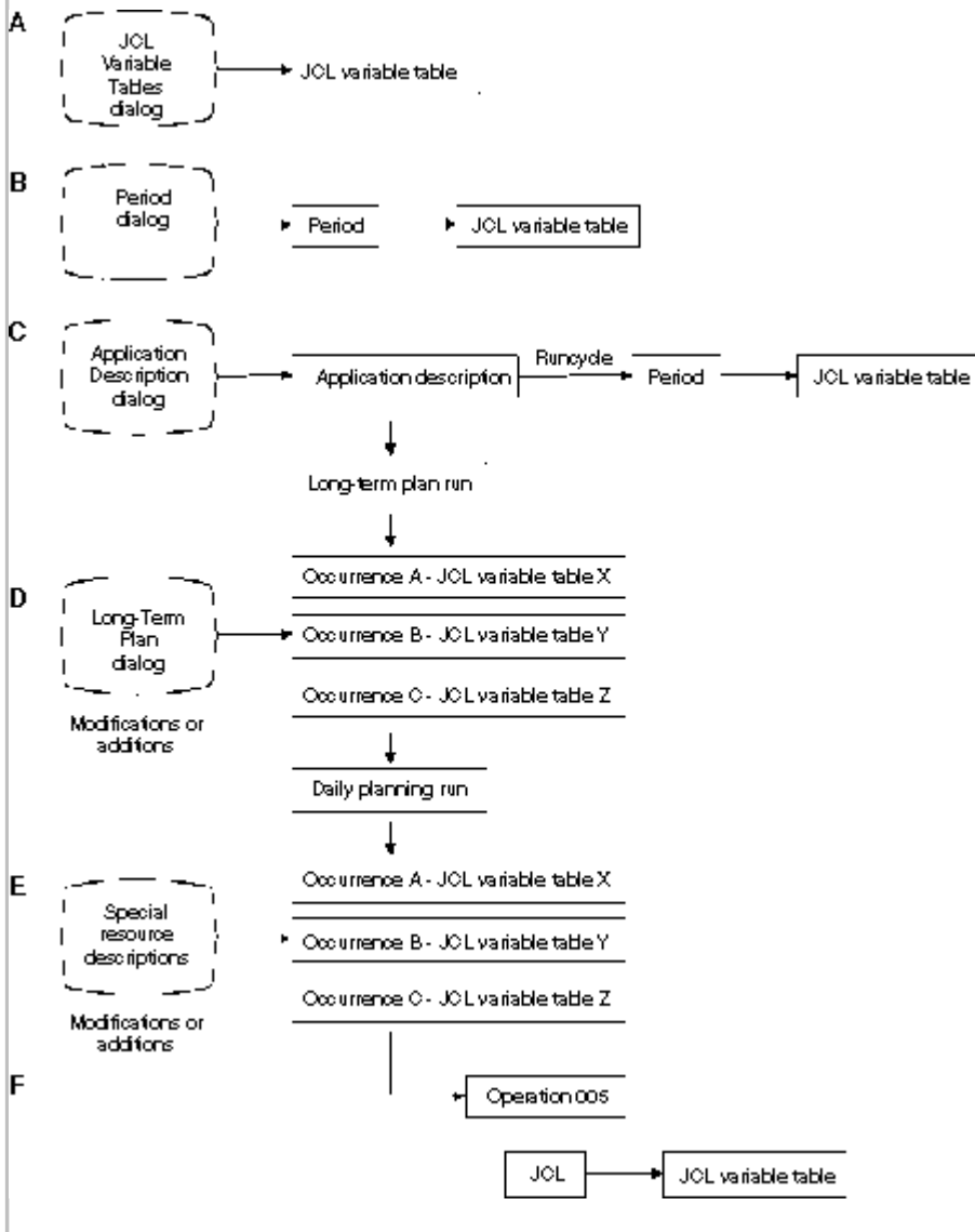
Figure 204. JCL variable handling
