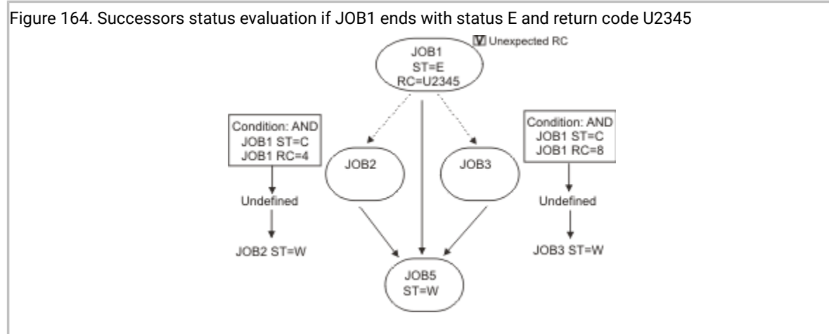
Figure 164: Successors status evaluation if JOB1 ends with status E and return code U2345 on page 490
