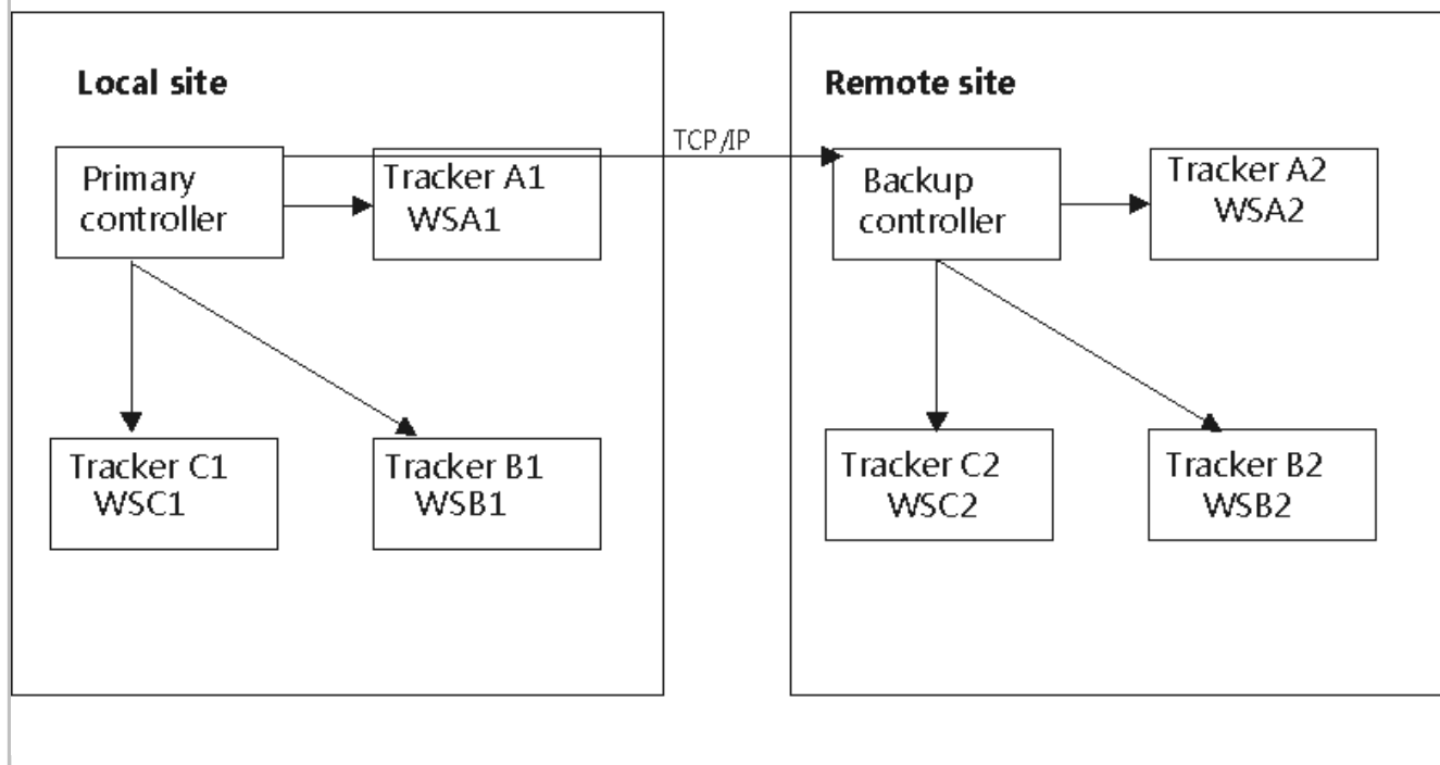
Figure 151. Configuring the local site and remote site in the same way
