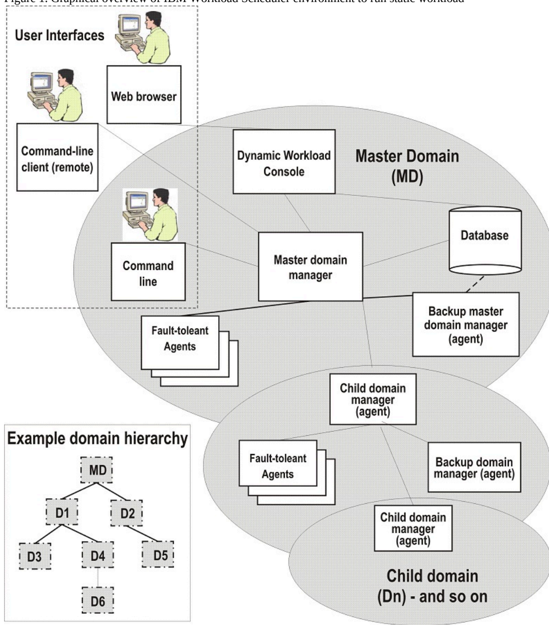
Figure 1. Graphical overview of IBM Workload Scheduler environment to run static workload
