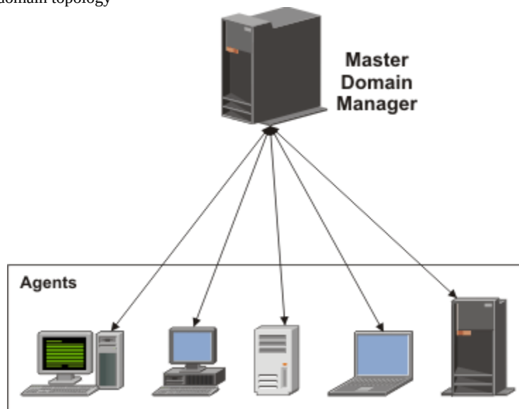
Figure 9. Single domain topology
