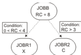
Figure 6. Example of recovery job with condition dependencies
