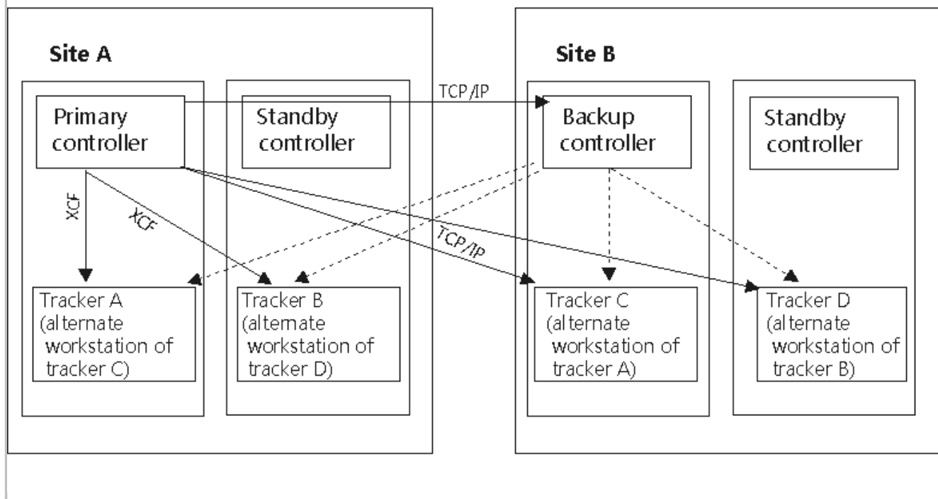
Figure 150. Configuring trackers, primary controller, and backup controller
