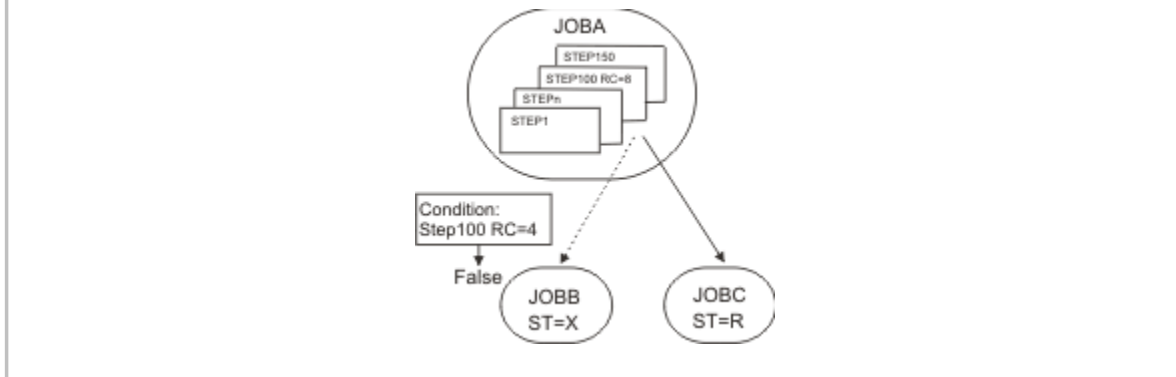
Figure 170. Step dependency status evaluation if Step100 ends with return code 8 and JOBA ends successfully
