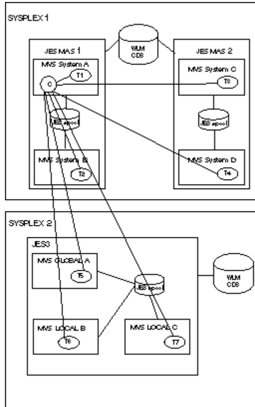
Figure 217. Multi-sysplex configuration: multiple JESplex
