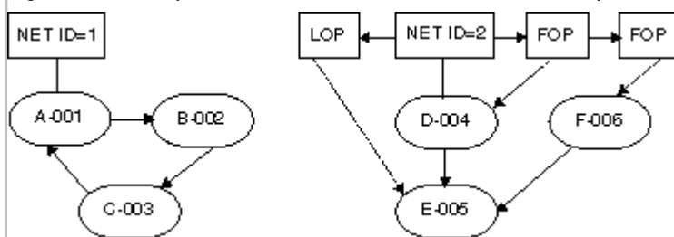
Figure 219. Example of a NO ENTRY AND/OR EXIT POINT loop condition
