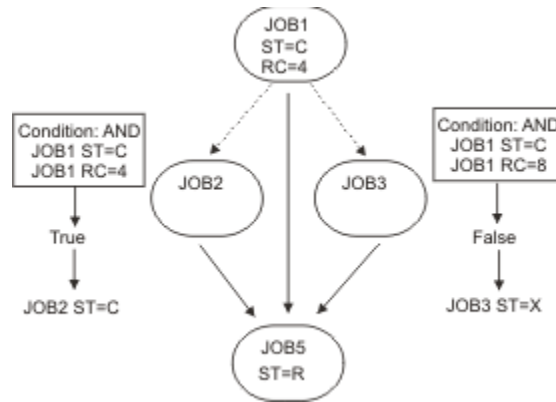
Figure 162. Successors status evaluation if JOB1 ends with status C and return code 4 and JOB2 runs successfully
