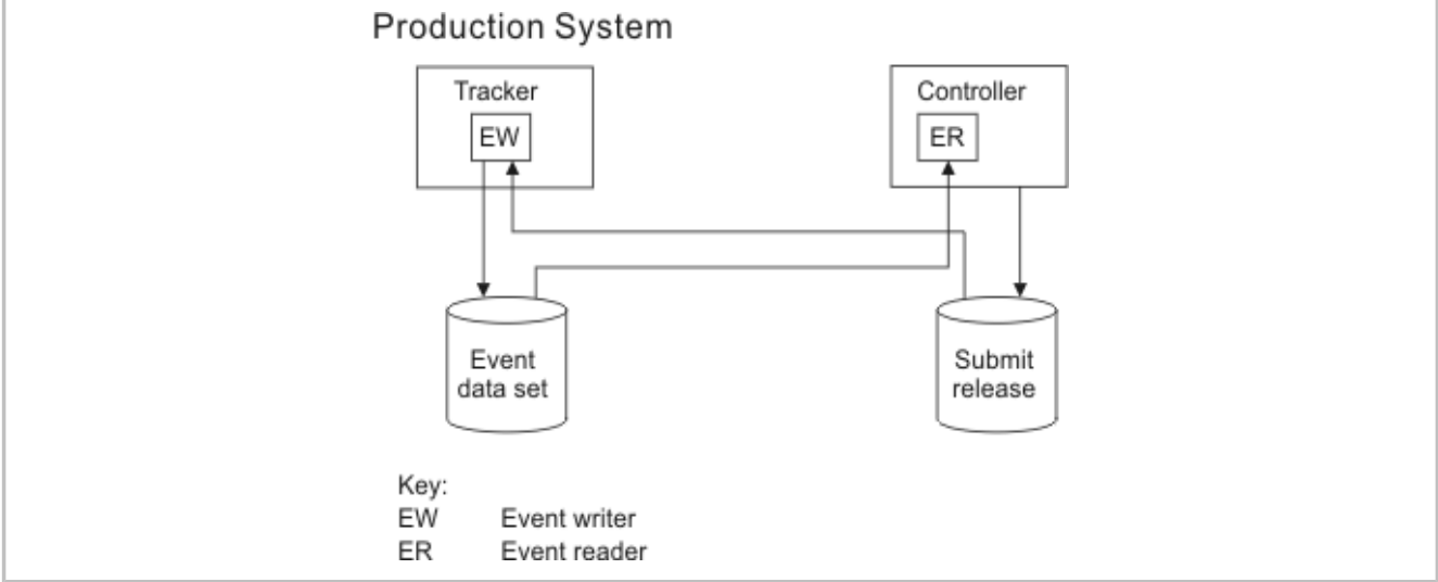
Figure 5. A z/OS system connected through shared DASD
