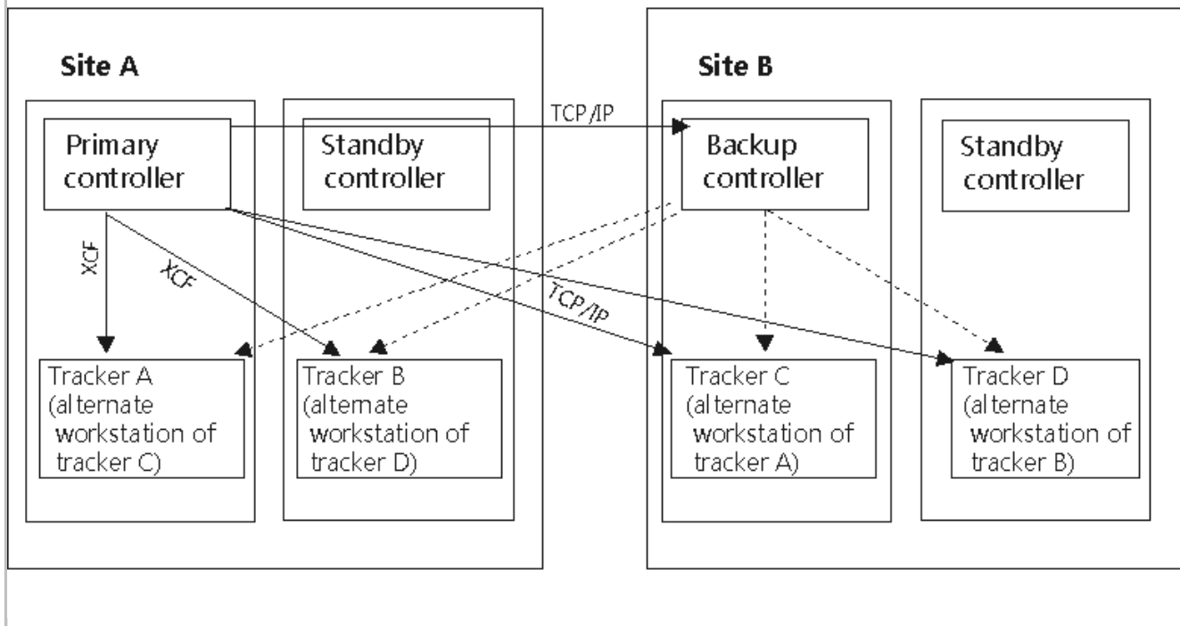
Figure 12. Configuring trackers, primary controller, and backup controller
