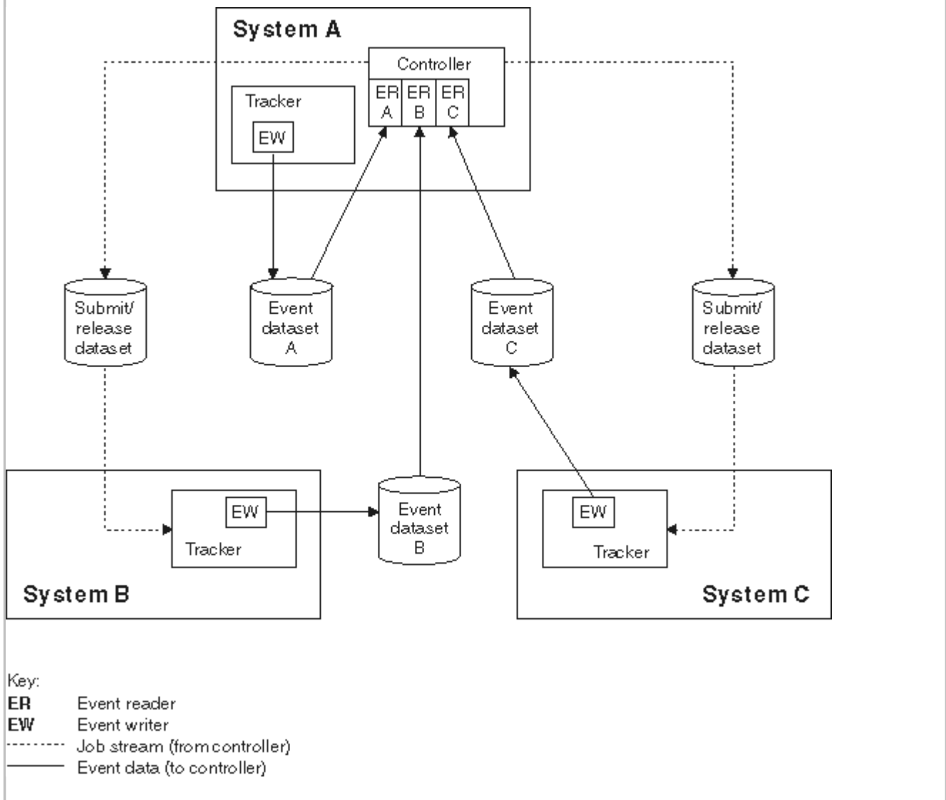
Figure 28. Individual systems connected through shared DASD
