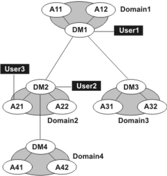
Figure 25. Network links
