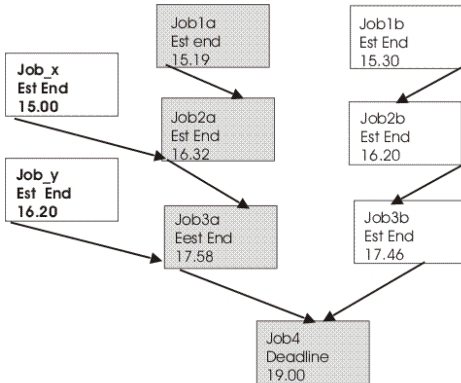
Figure 22. Critical path
