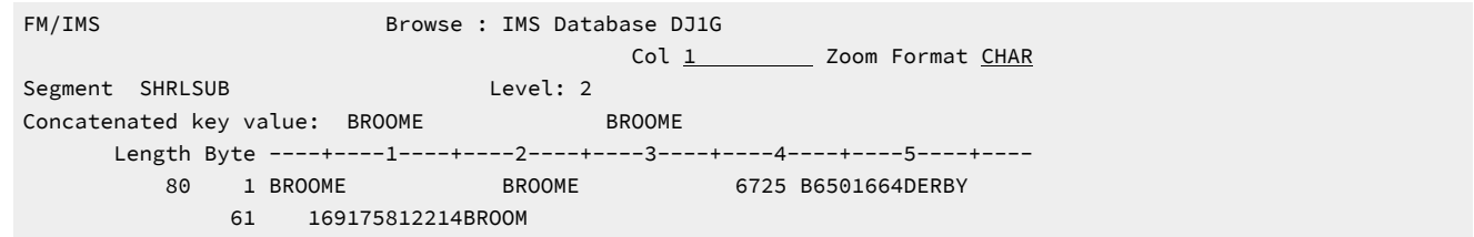
Figure 13. Zooming in on one segment (CHAR display format)
