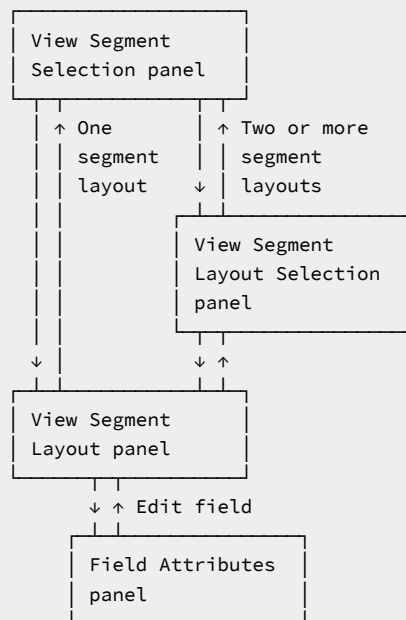
Figure 18. Editing a view
