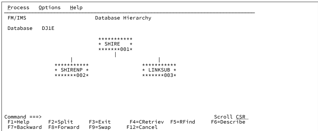
Figure 39. Database Hierarchy panel
