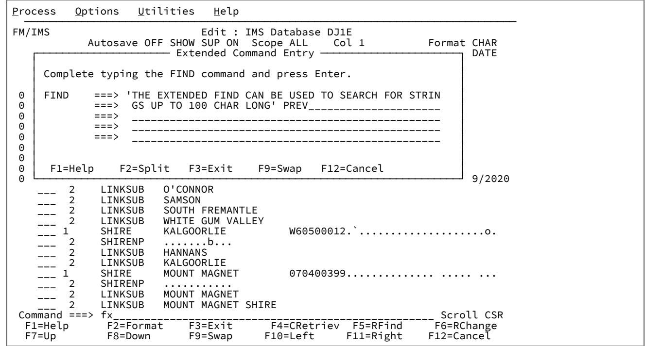
Figure 124. Extended Command Entry pop-up panel for the FIND command showing contiguous nature of entry lines
