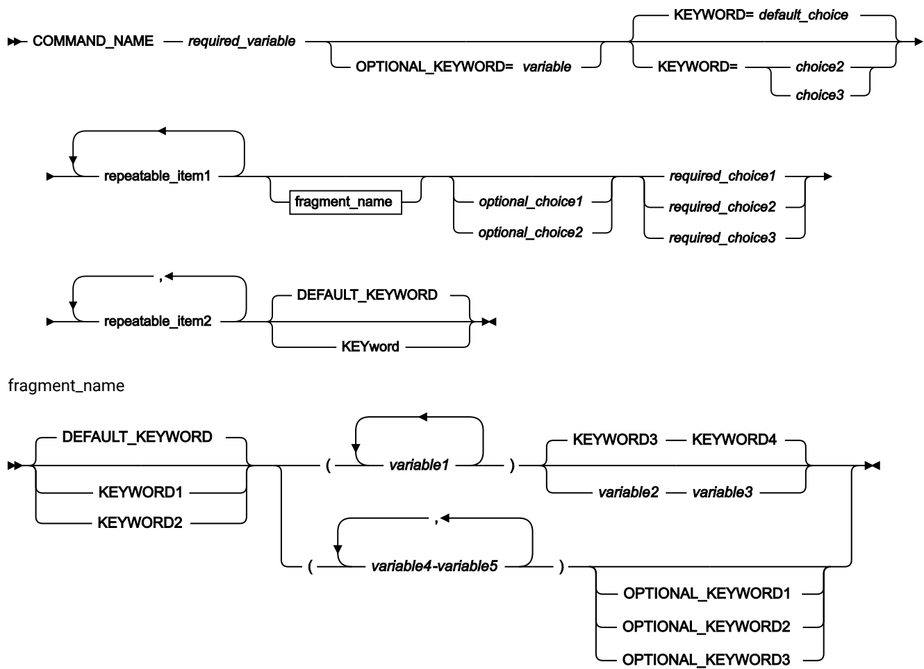
Figure 1. Syntax
