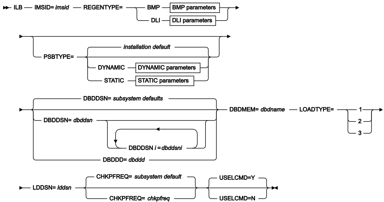
Figure 145. Syntax
