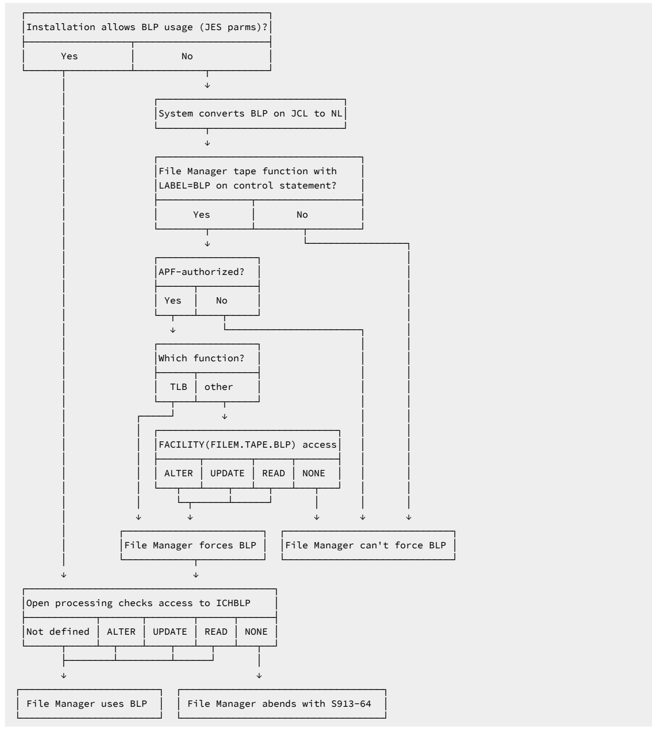
Figure 13. BLP processing by File Manager
