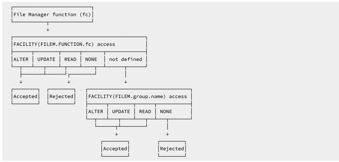
Figure 10. Access to File Manager functions
