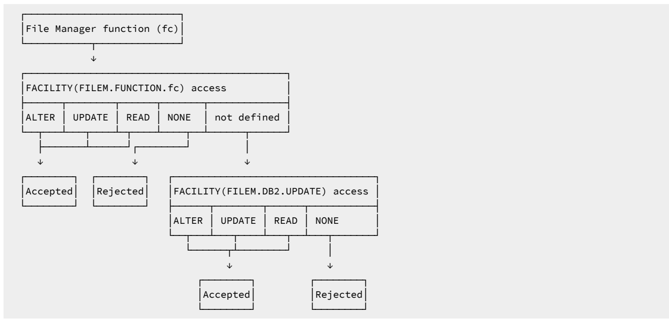
Figure 15. Security system validation for update functions
