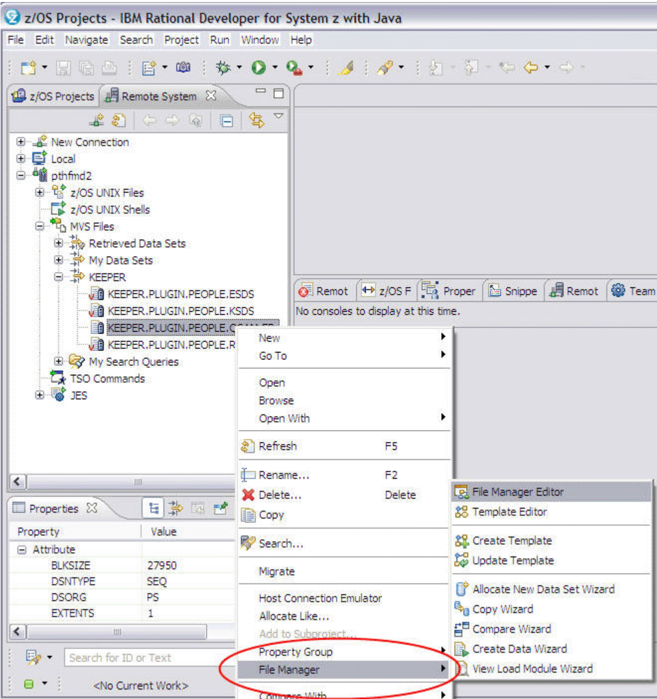
Figure 71. Screenshot of IBM® File Manager plug-in for Eclipse
