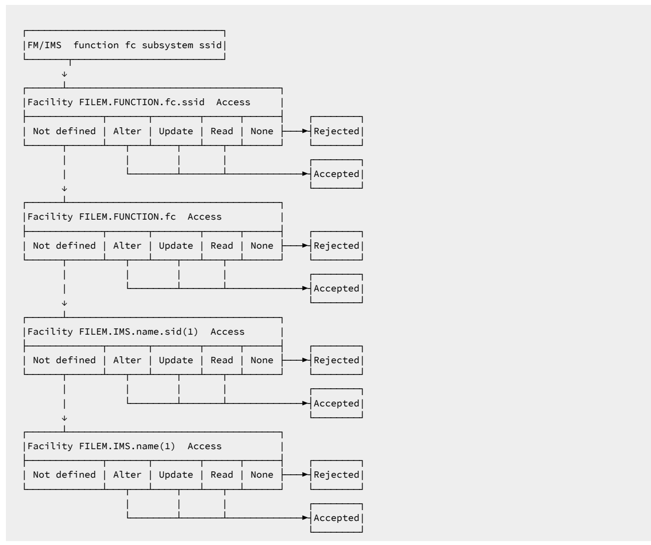
Figure 55. Security checking for FM/IMS functions
