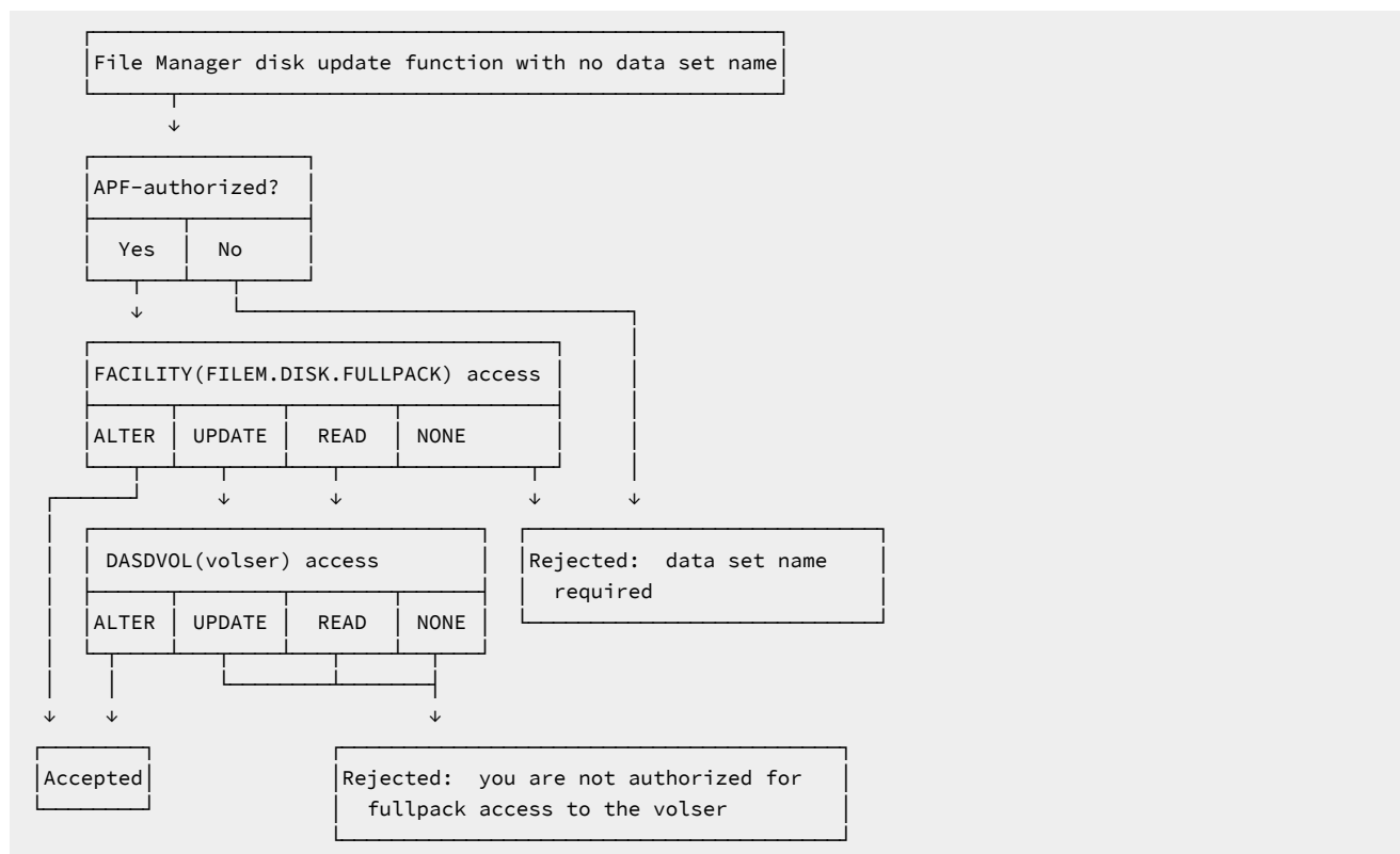
Figure 12. Fullpack processing for disk update functions
