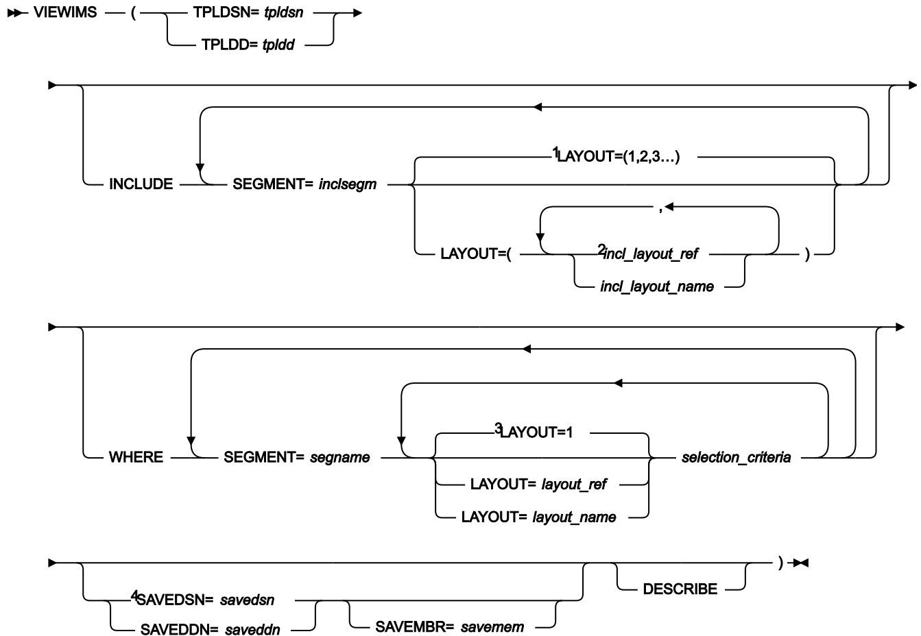
図 167. Syntax (to create a new view from an existing template)
