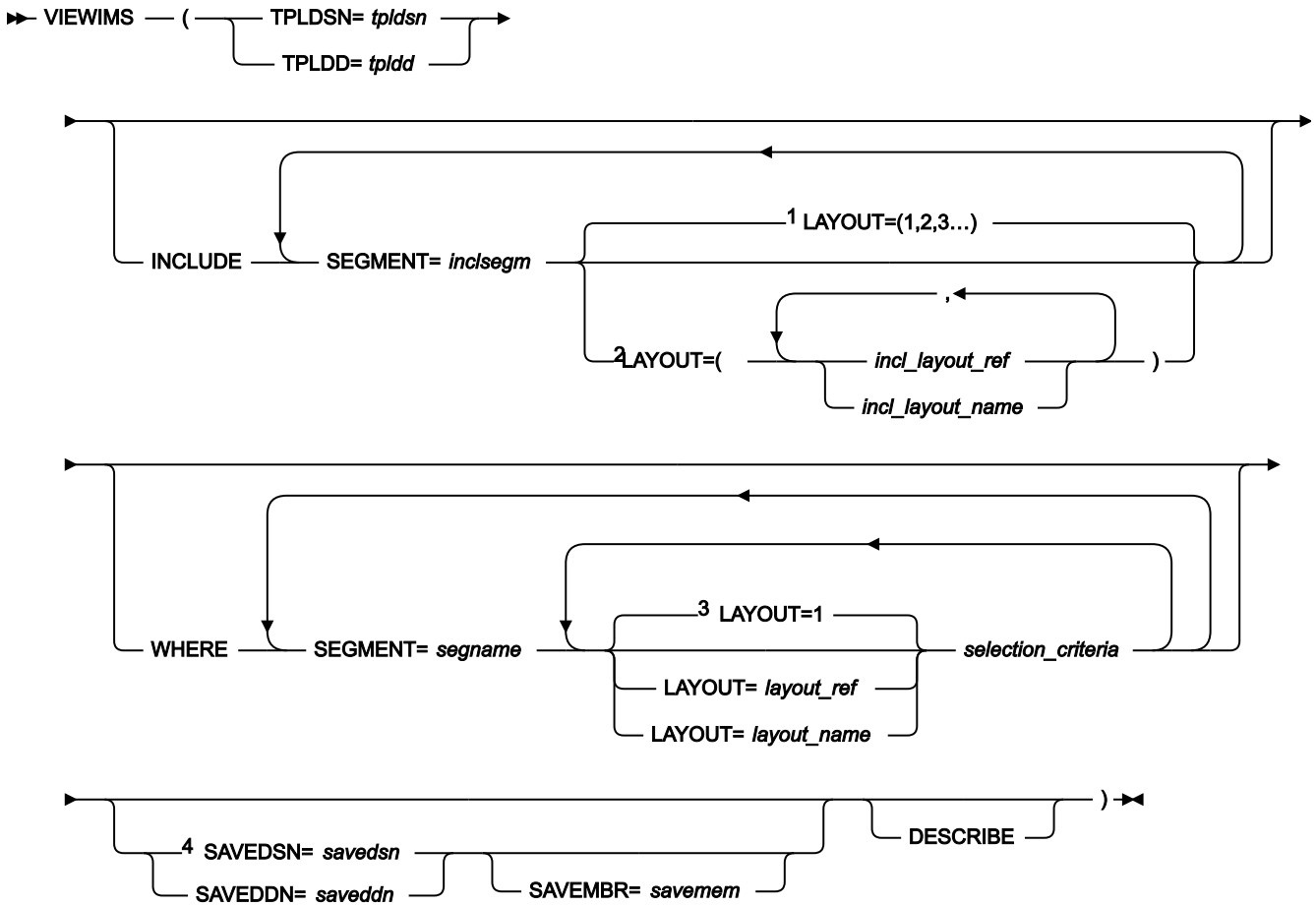
図 158. Syntax (to create a new view from an existing template)
