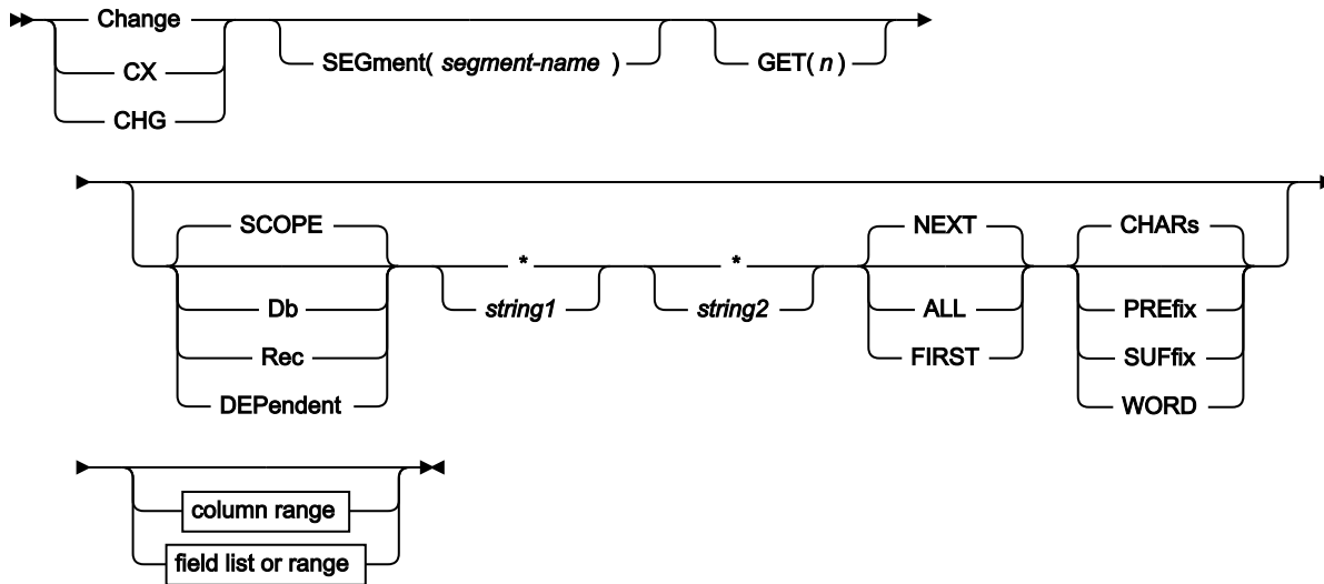
図 122. CHANGE syntax in edit
