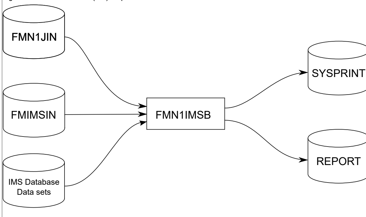
Figure 149. Flows for Print (IPR) step
