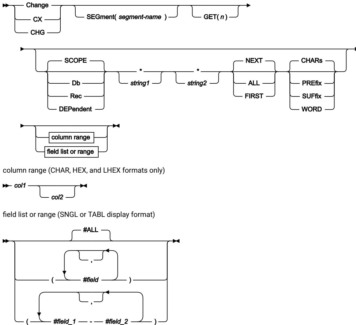
Figure 122. CHANGE syntax in edit
