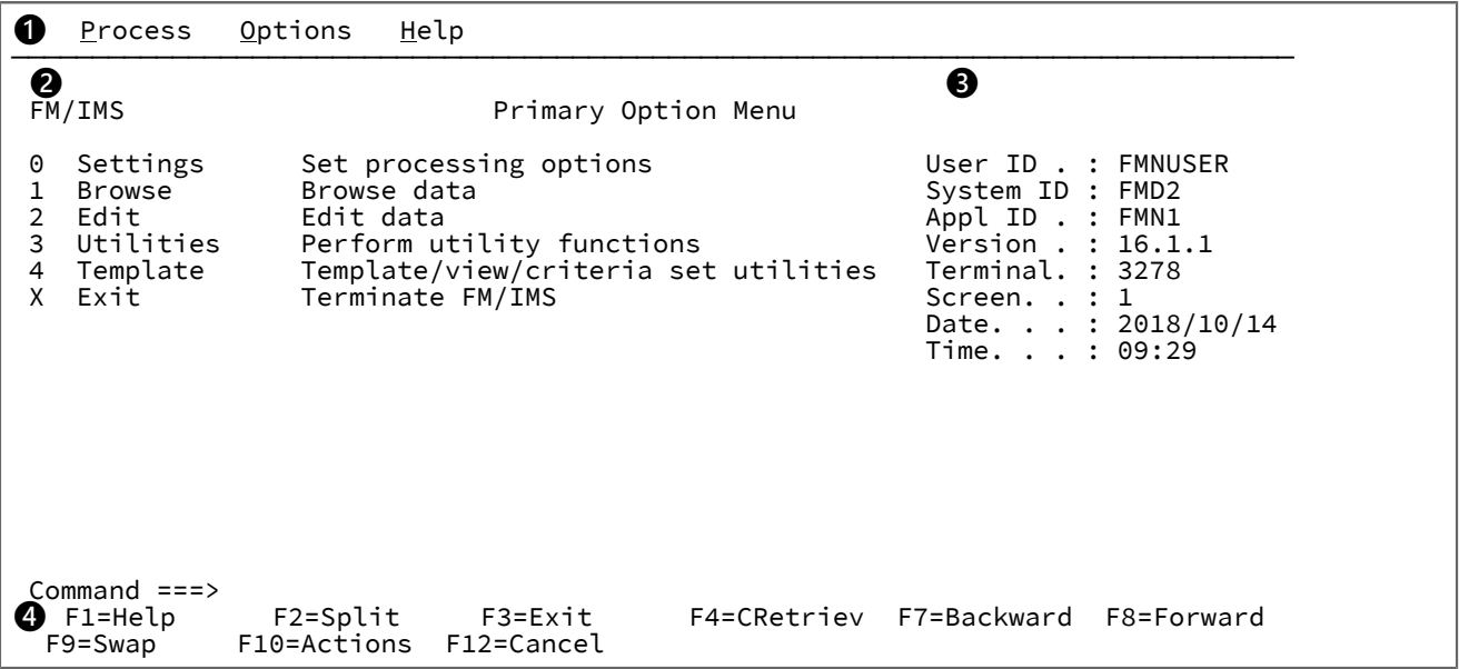
Figure 81. Primary Option menu
