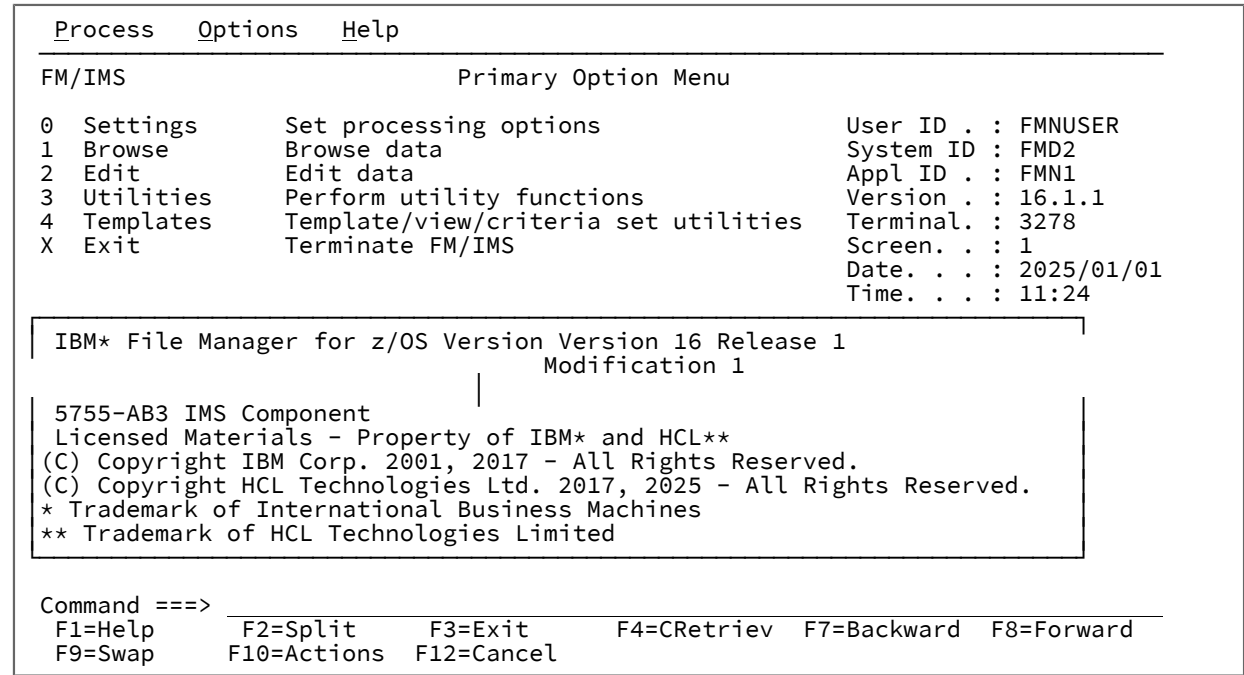
Figure 8. Primary Option menu with version information
