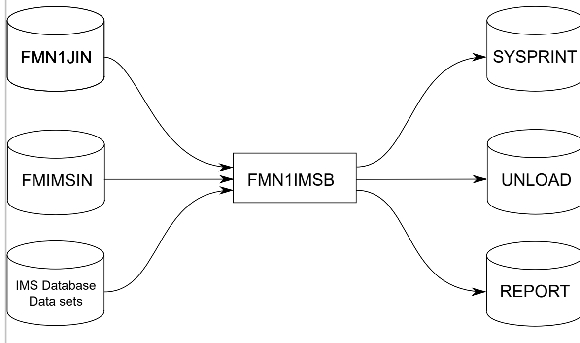
Figure 140. Flows for Extract (IXB) step
