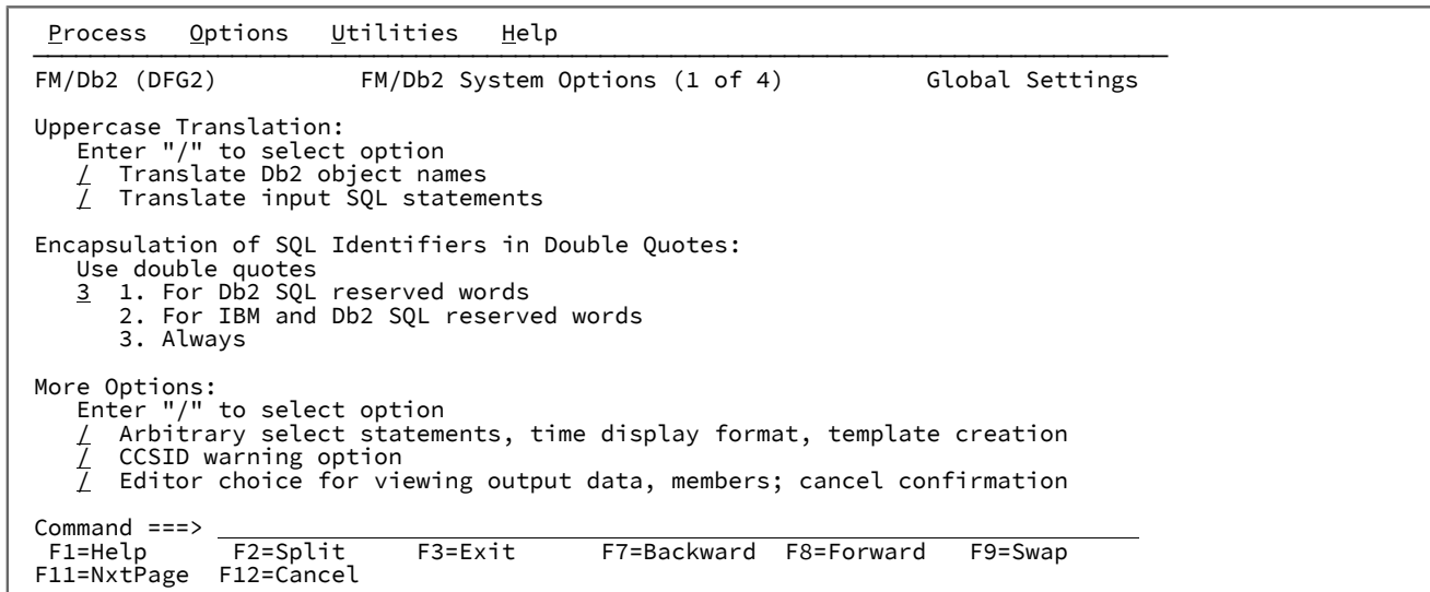
Figure 138. FM/Db2 System Options (1 of 4) panel
