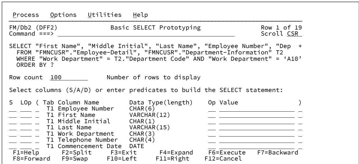
Figure 35. Basic SELECT Prototyping panel (6)
