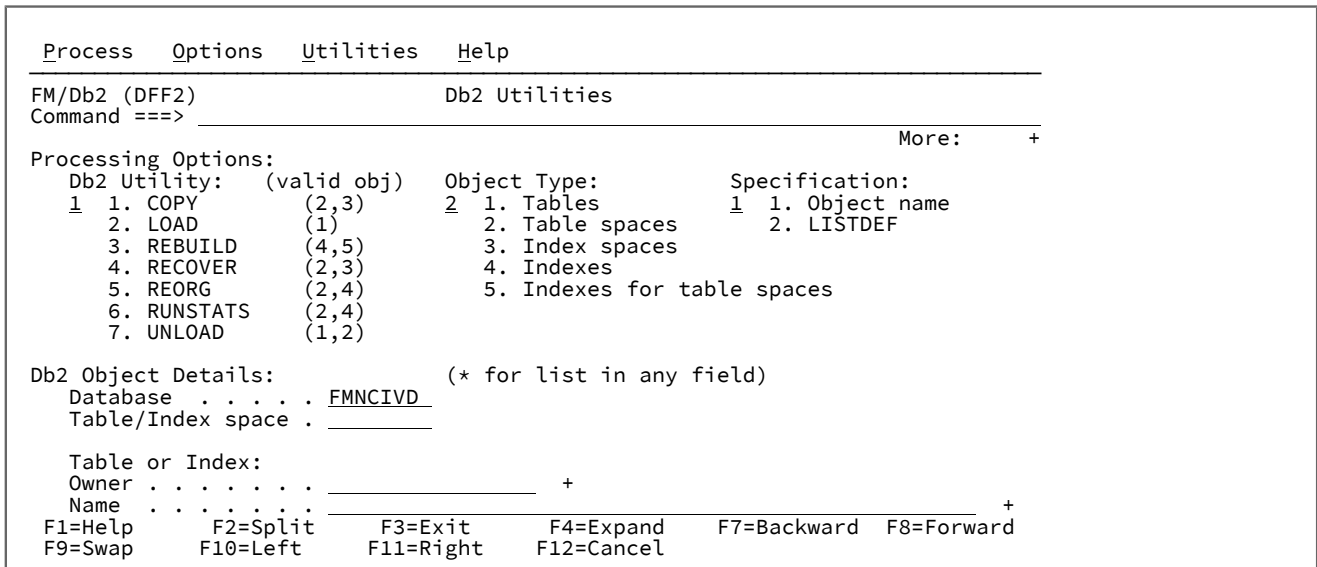
Figure 20. Db2® Utilities panel
