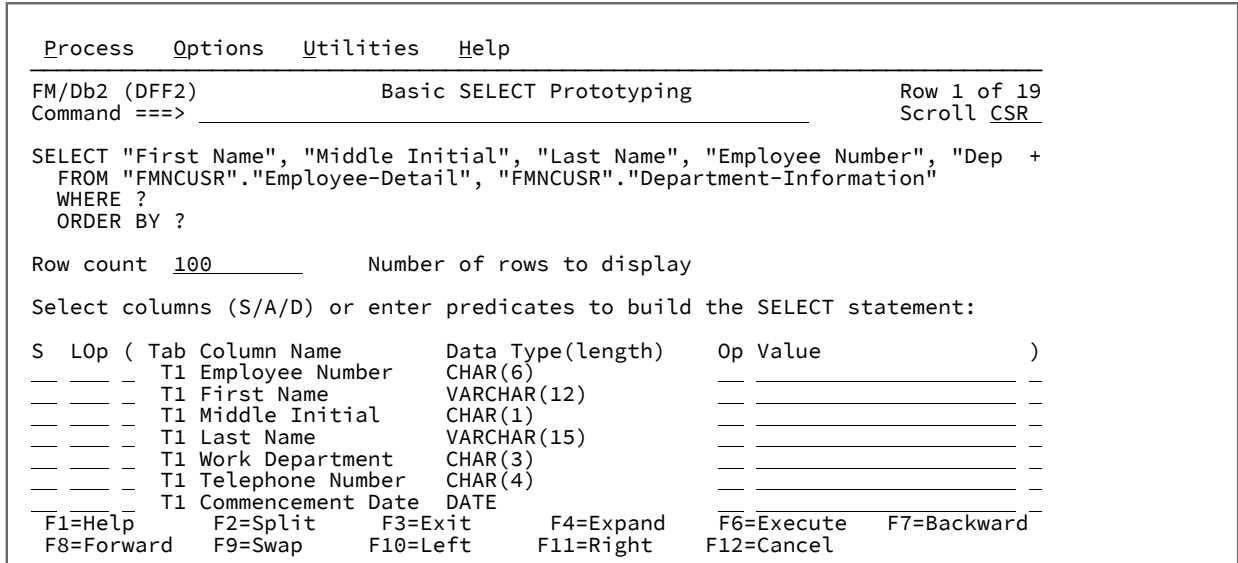
Figure 32. Basic SELECT Prototyping panel (3)
