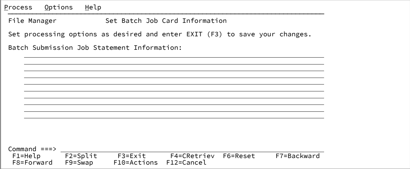
Figure 310. Set Batch Job Card Information
