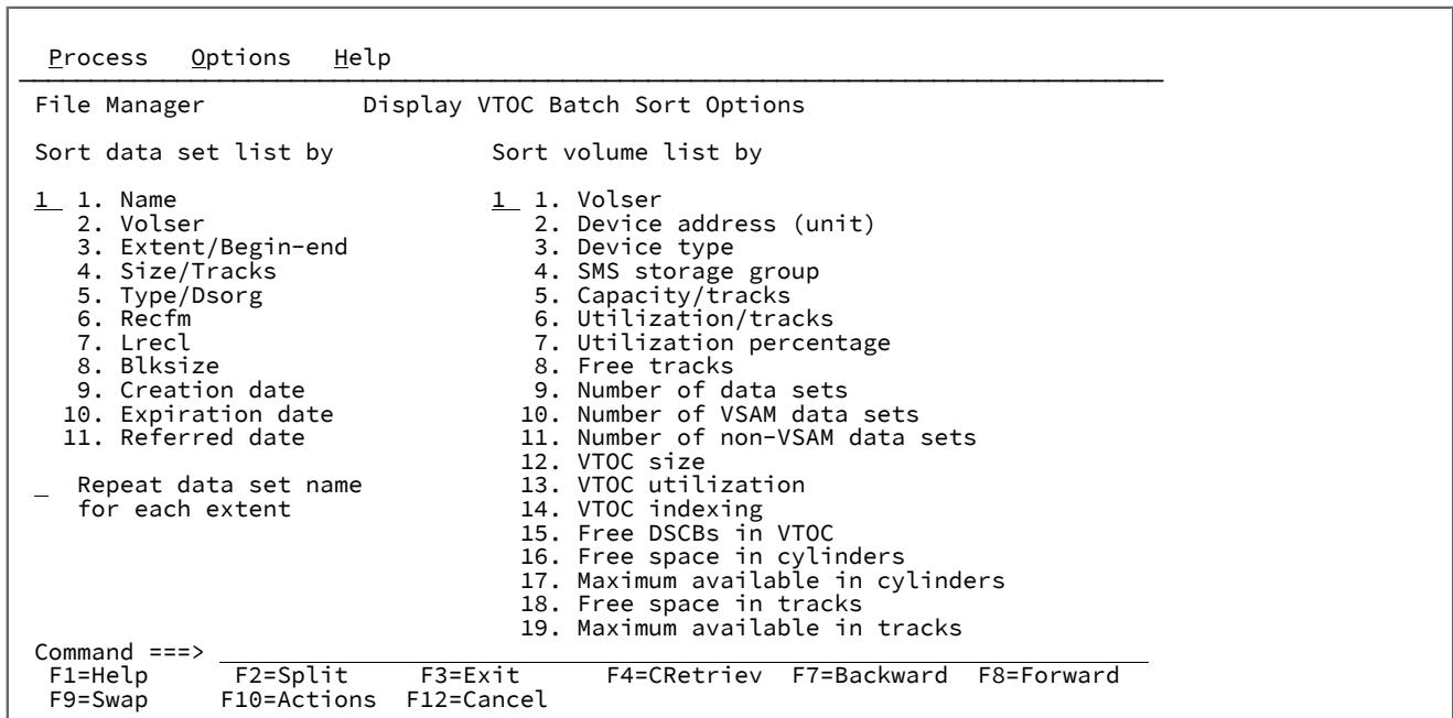
Figure 229. Display VTOC Batch Sort Options panel
