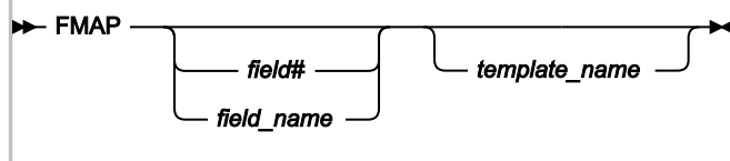
Figure 127. Syntax
