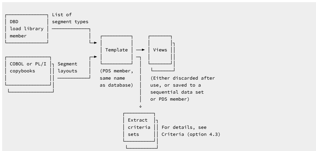
Figure 17. Overview of templates and views
