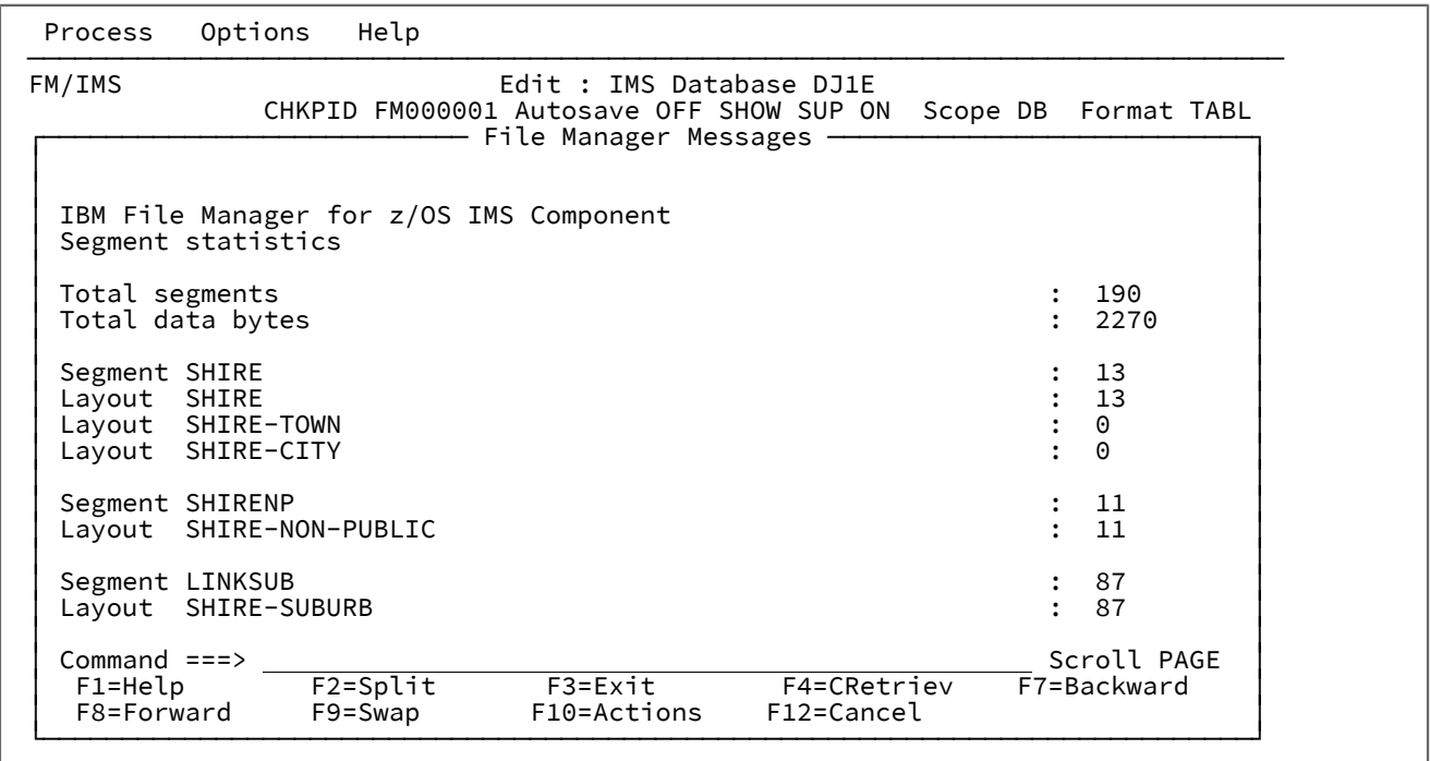
Figure 15. Example of statistics for an Edit session listed with the SEGSTATS command
