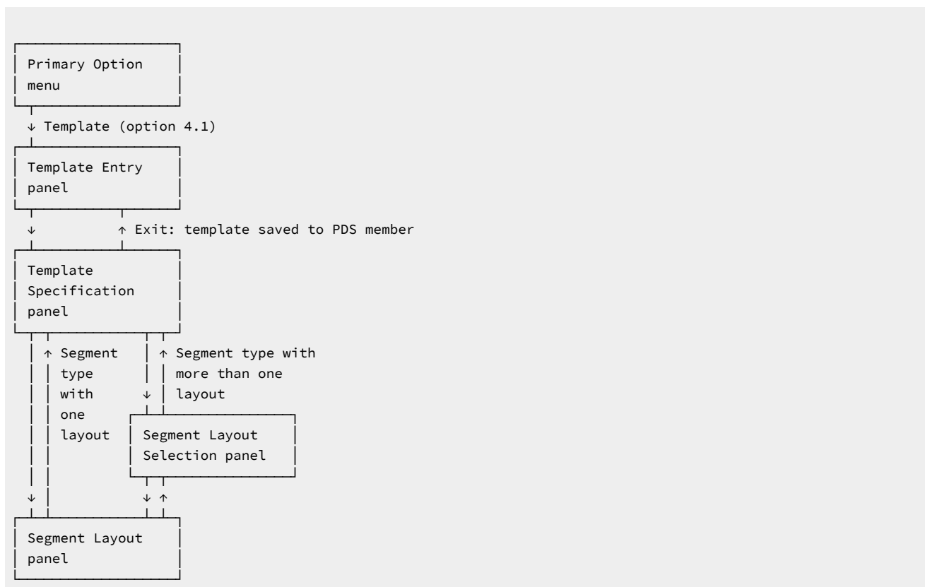
Figure 16. Editing a template
