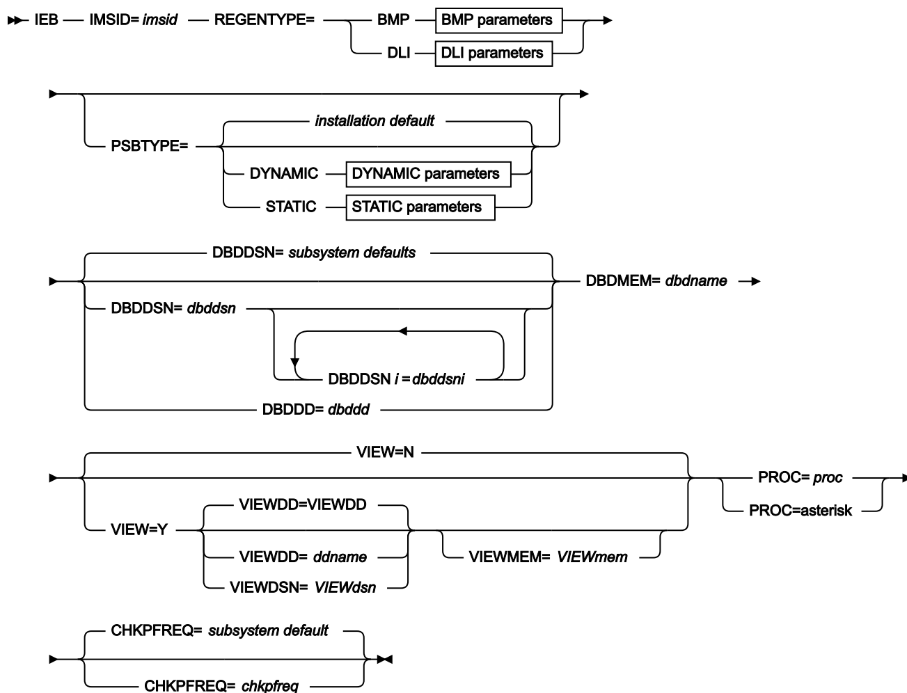
Figure 152. Syntax
