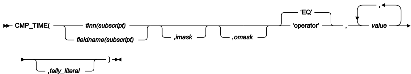
Figure 495. CMP_TIME syntax – with template
