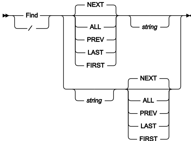
Figure 382. Syntax - selection lists
