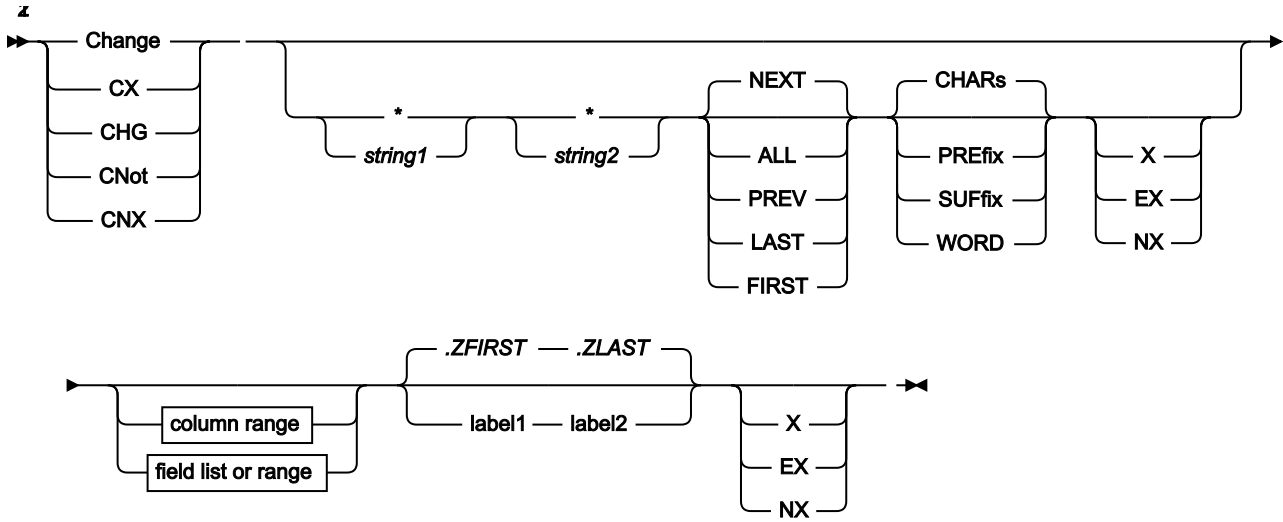
Figure 374. Syntax in the Editor
