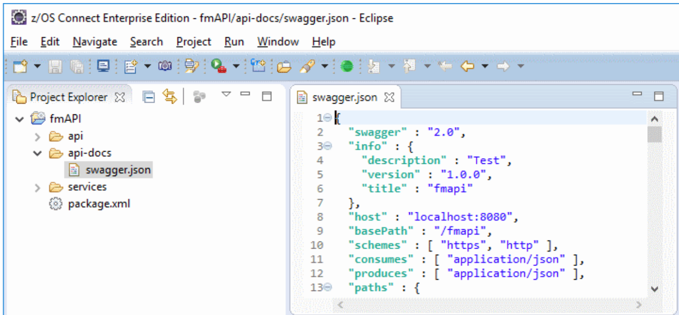
Figure 176. z/OS® Connect Swagger JSON
