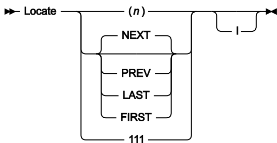
Figure 390. Syntax in Non-VSAM Extent Information panel
