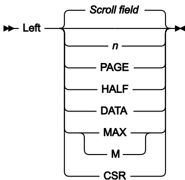
Figure 387. Syntax in View or Edit
