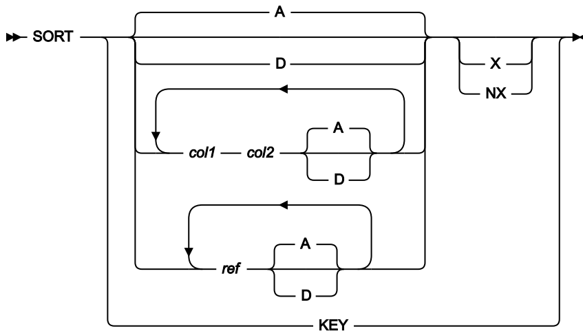
Figure 408. Syntax: View and Edit
