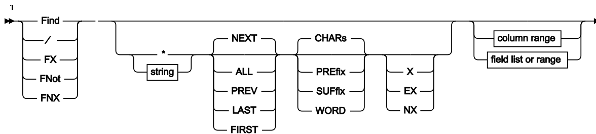
Figure 378. Syntax in View or Edit
