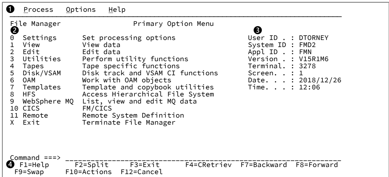
Figure 290. File Manager Primary Option Menu panel
