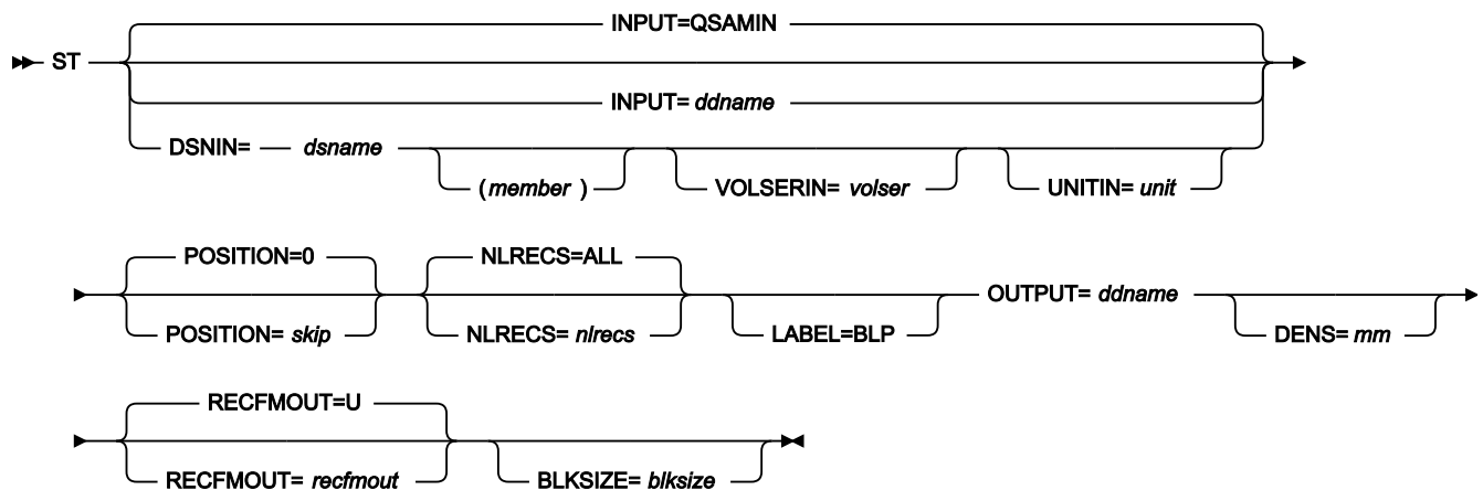
Figure 467. Syntax
