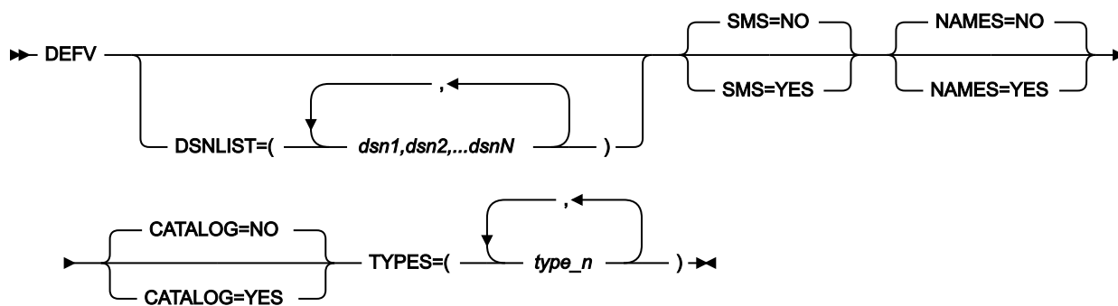
Figure 424. Syntax
