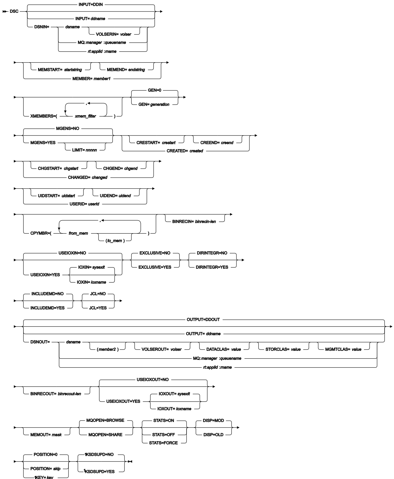
Figure 428. Syntax
