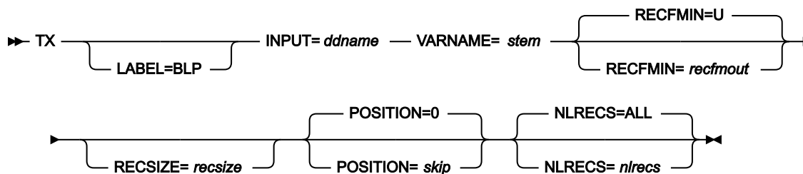
Figure 480. Syntax
