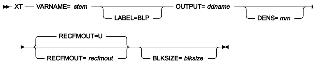
Figure 486. Syntax
