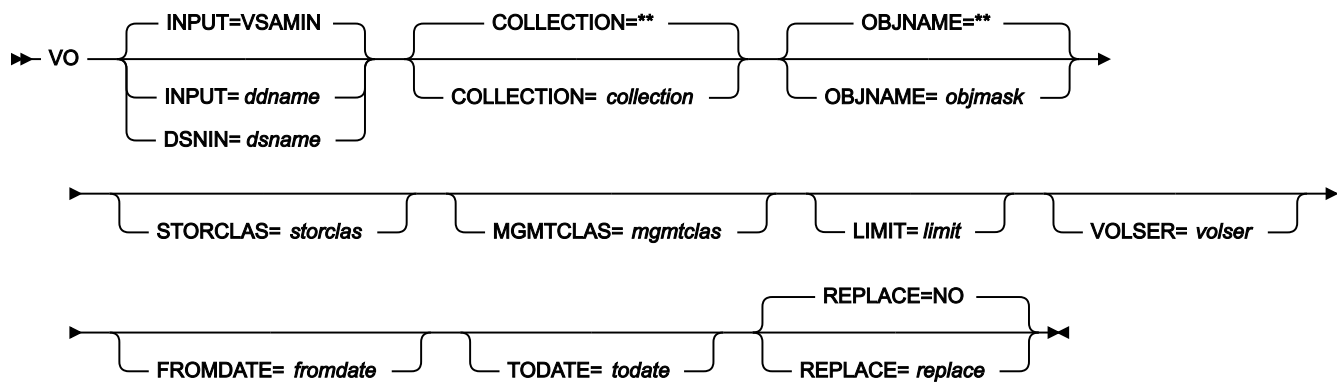
Figure 482. Syntax
