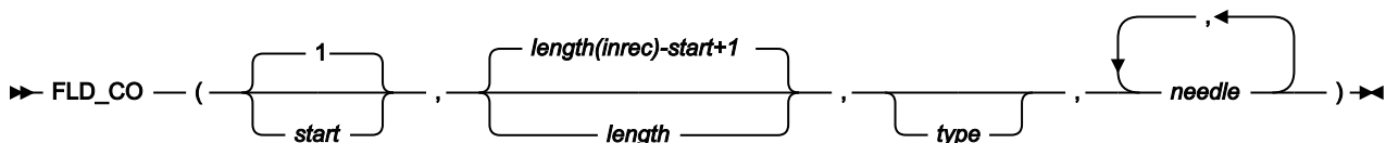
Figure 500. Syntax
