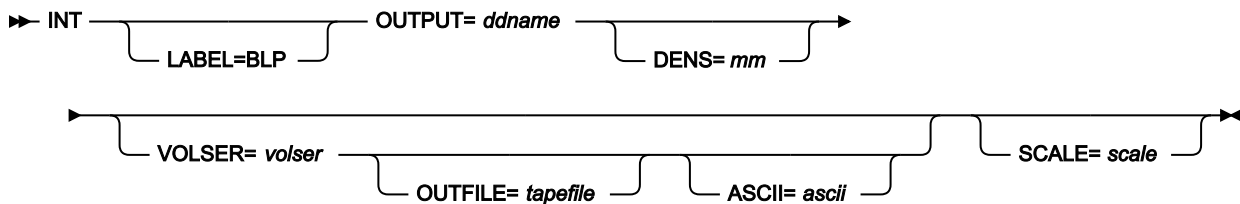
Figure 450. Syntax
