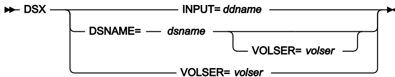
Figure 441. Syntax
