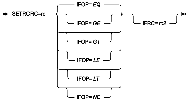
Figure 465. Syntax
