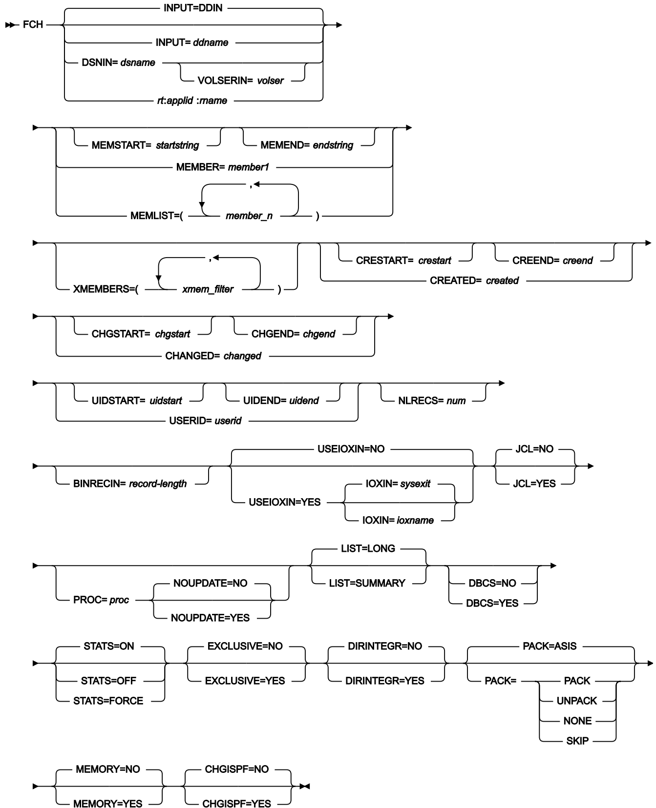
Figure 446. Syntax
