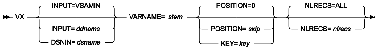
Figure 484. Syntax
