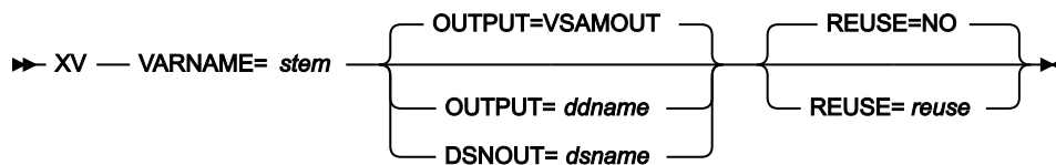
Figure 487. Syntax
