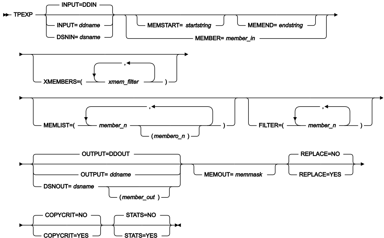
Figure 472. Syntax
