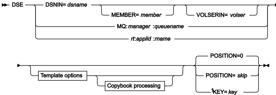
Figure 429. Syntax
