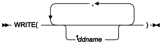
Figure 544. Syntax
