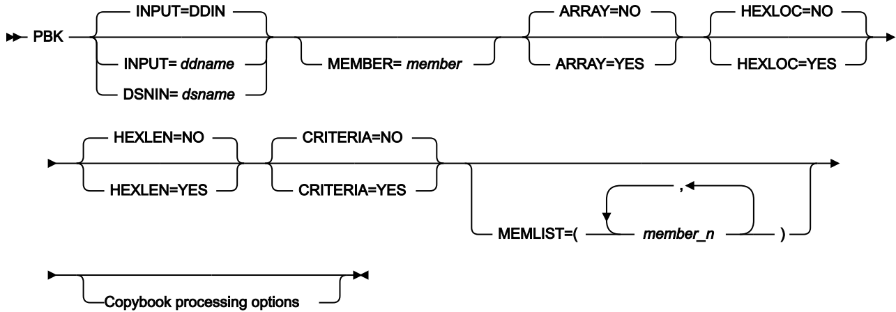
Figure 458. Syntax
