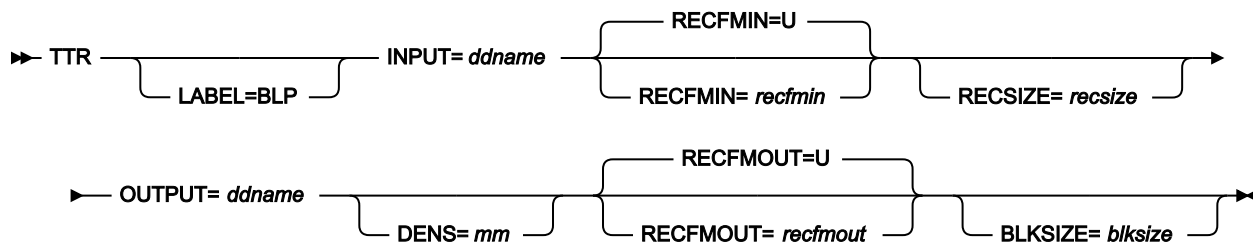
Figure 478. Syntax
