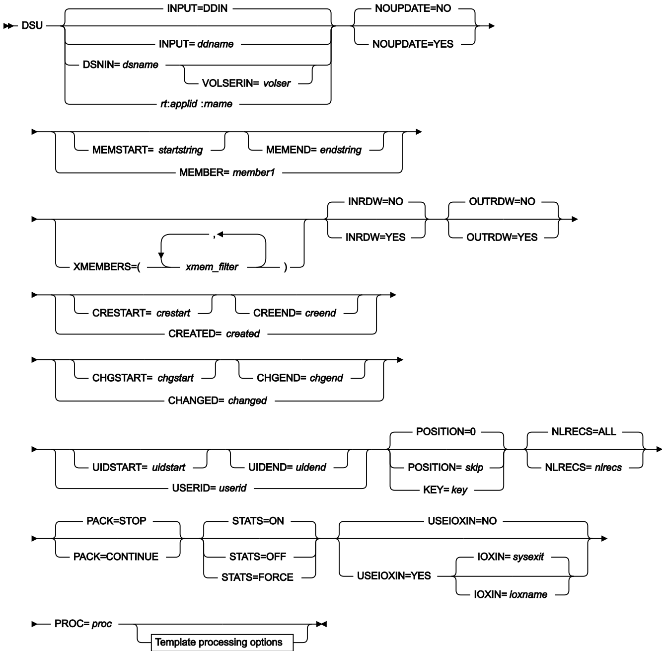
Figure 439. Syntax
