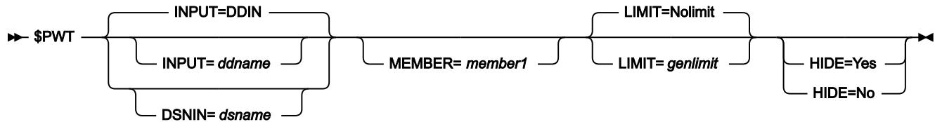
Figure 80. Syntax
