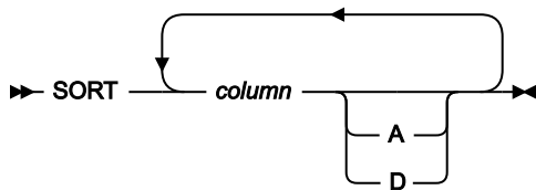
Figure 409. Syntax: selection list panels
