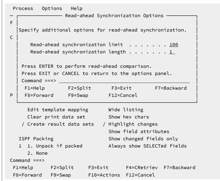
Figure 205. Read-ahead Synchronization Limit panel
