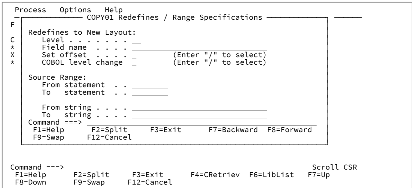
Figure 301. Redefines / Range Specifications panel
