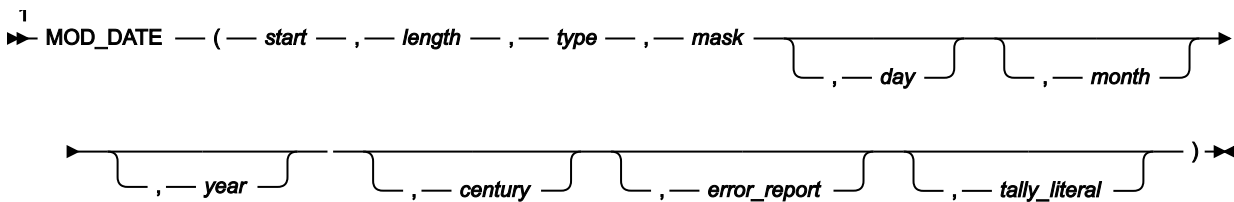
Figure 508. MOD_DATE syntax - without template
