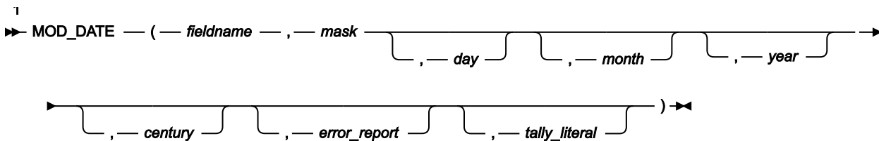
Figure 507. MOD_DATE syntax - with template
