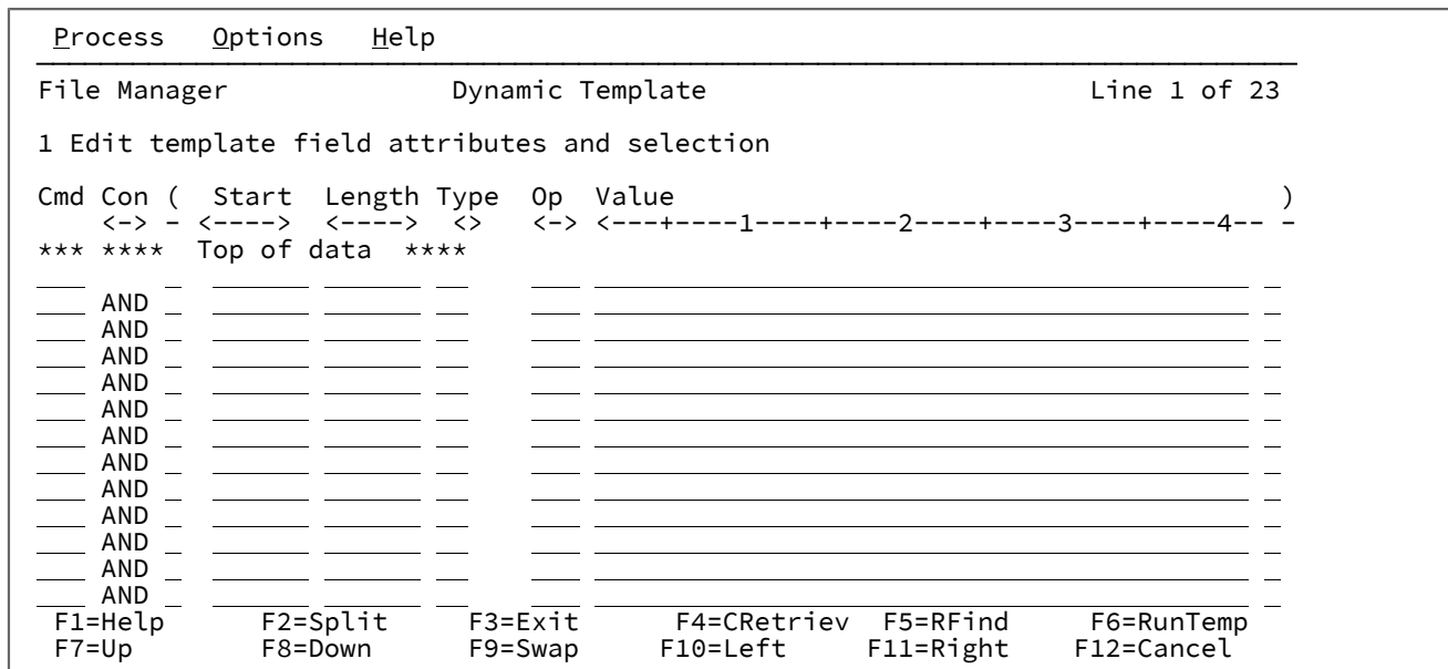
Figure 231. Dynamic Template panel
