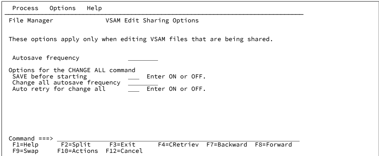
Figure 50. VSAM Edit Sharing Options panel
