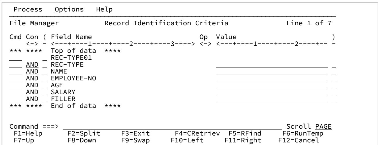
Figure 295. Record Identification Criteria panel
