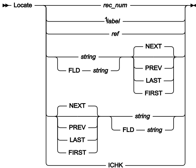
Figure 388. Syntax in View or Edit
