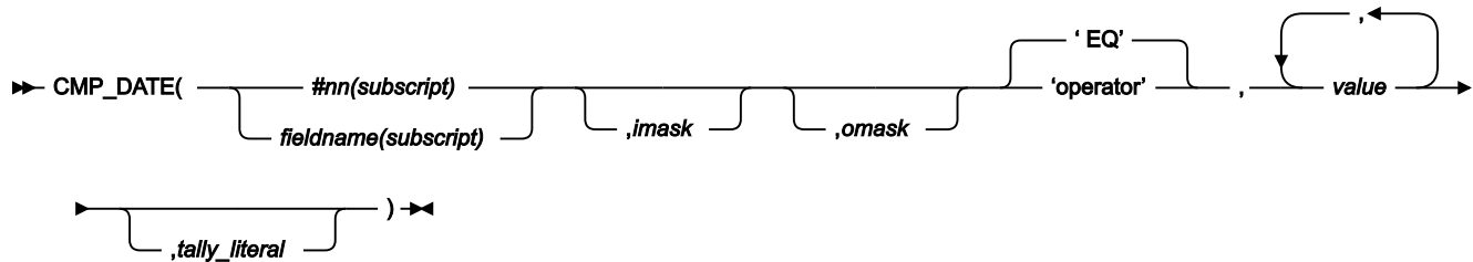
Figure 494. CMP_DATE syntax – without template
