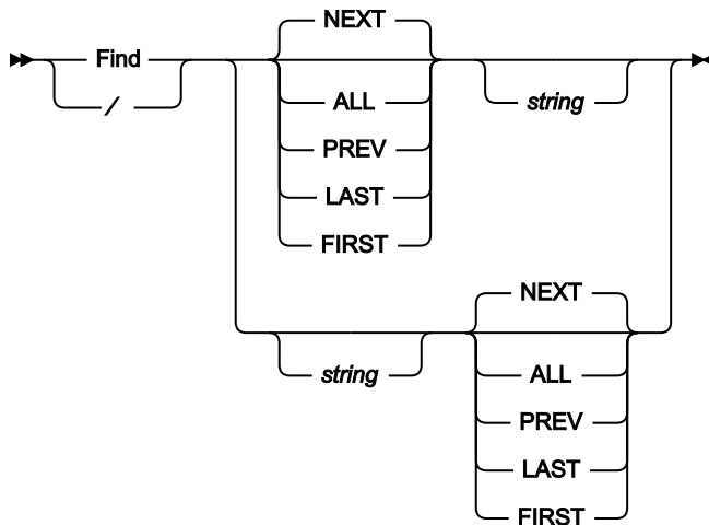
Figure 381. Syntax - member selection and Load Module Information panels
