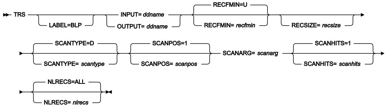
Figure 474. Syntax
