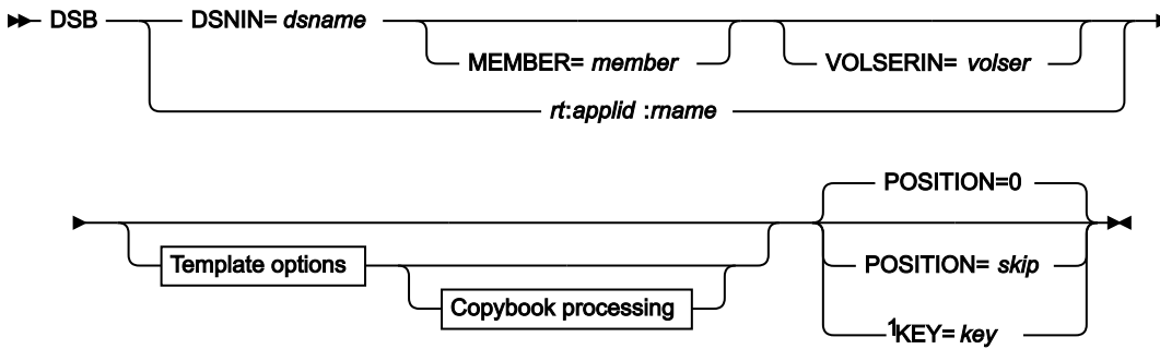
Figure 427. Syntax
