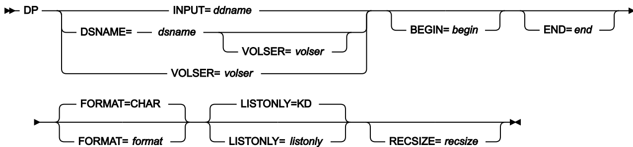
Figure 425. Syntax
