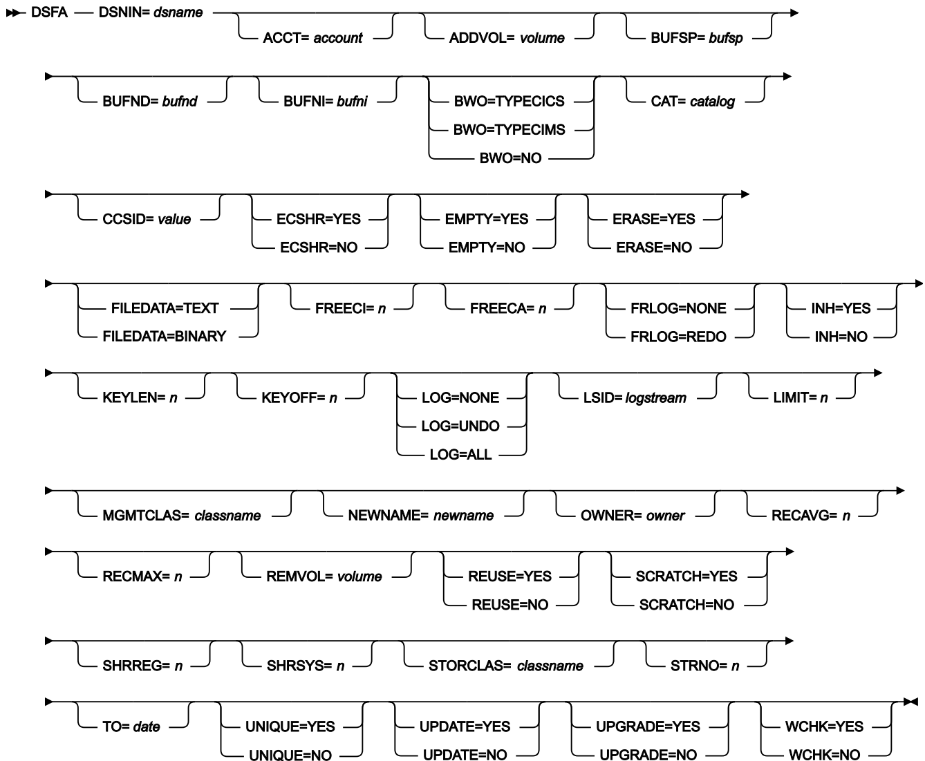
Figure 431. Syntax
