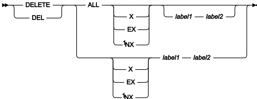
Figure 376. Syntax (CHAR, HEX, LHEX or TABL display format)
