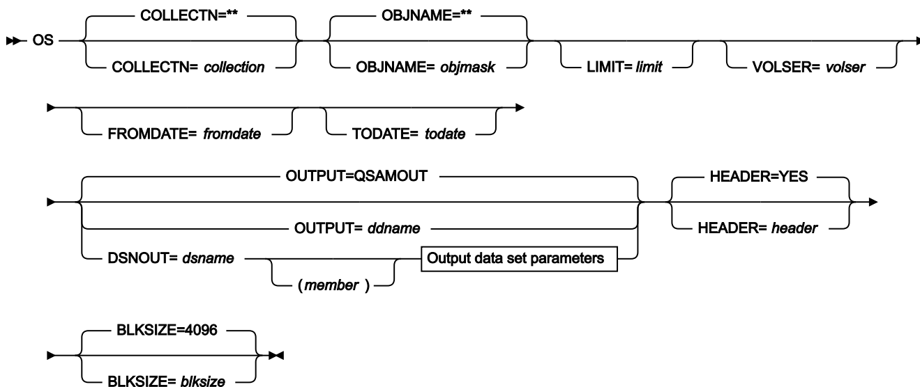
Figure 456. Syntax
