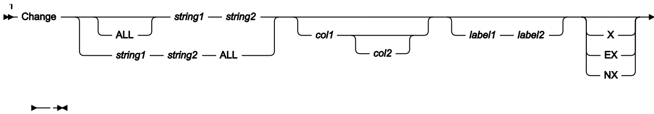
Figure 138. Syntax
