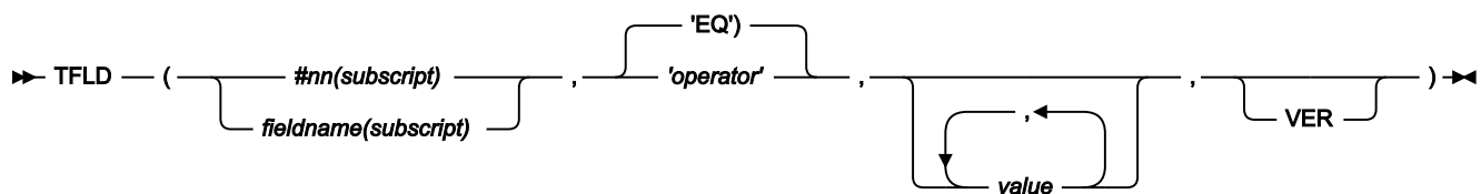
Figure 537. Syntax
