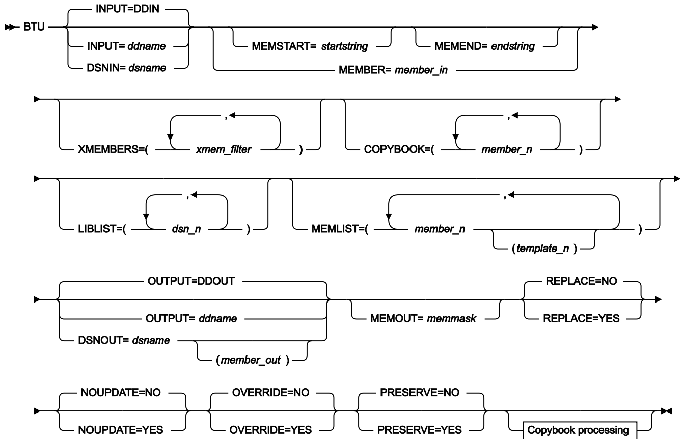
Figure 422. Syntax
