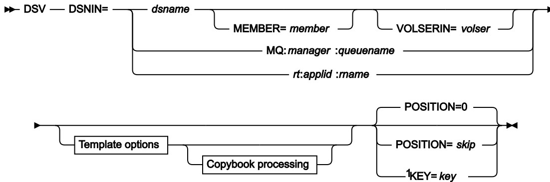
Figure 440. Syntax
