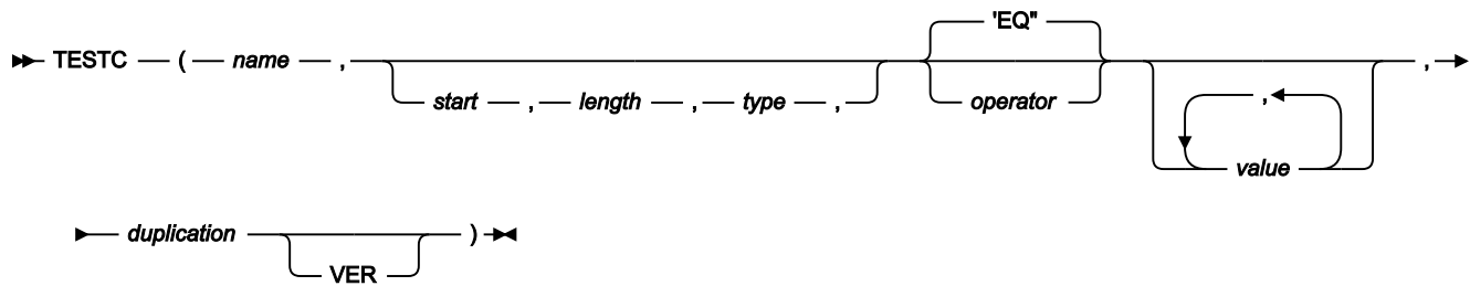
Figure 535. Syntax
