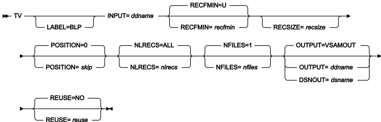
Figure 479. Syntax
