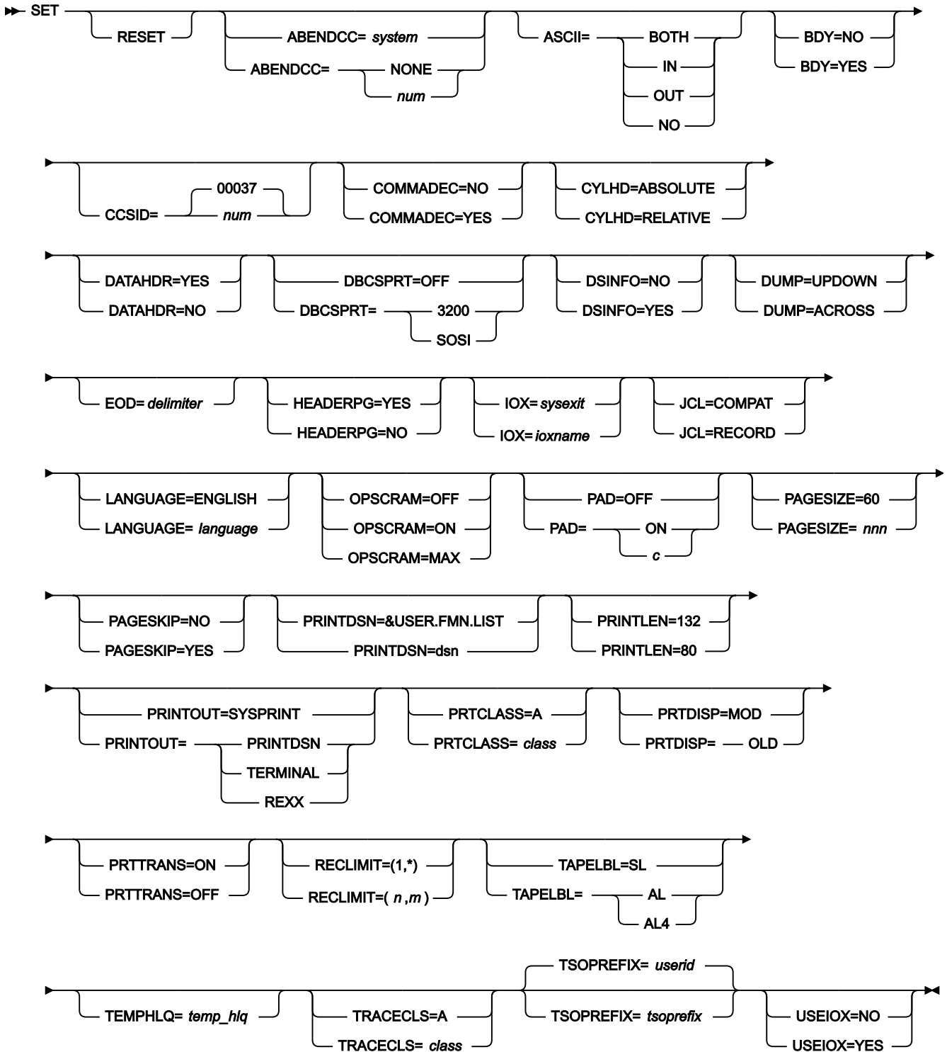
Figure 463. Syntax
