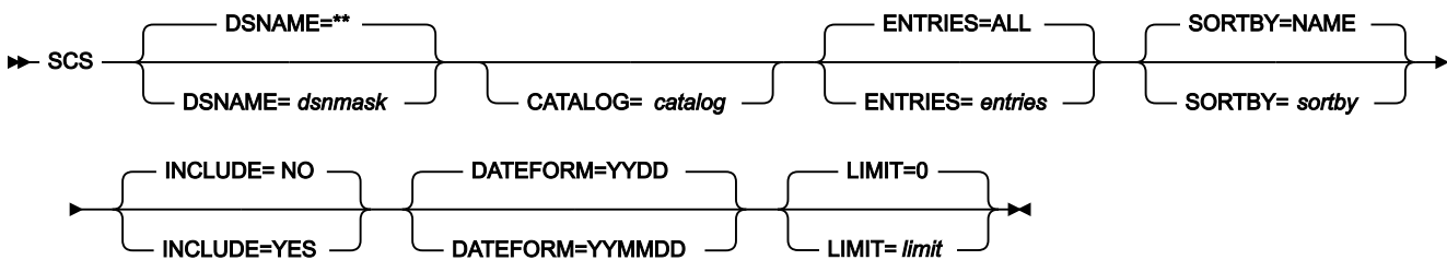
Figure 462. Syntax
