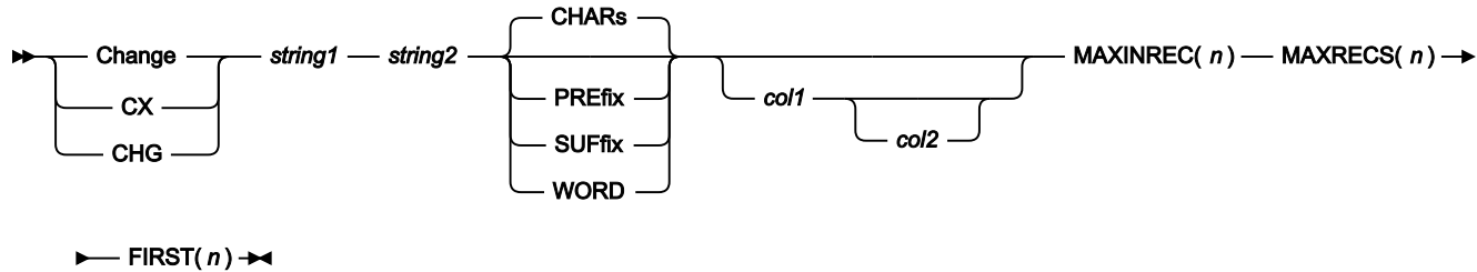
Figure 375. Syntax in the Find/Change Utility
