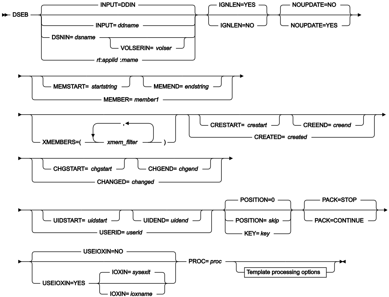
Figure 430. Syntax
