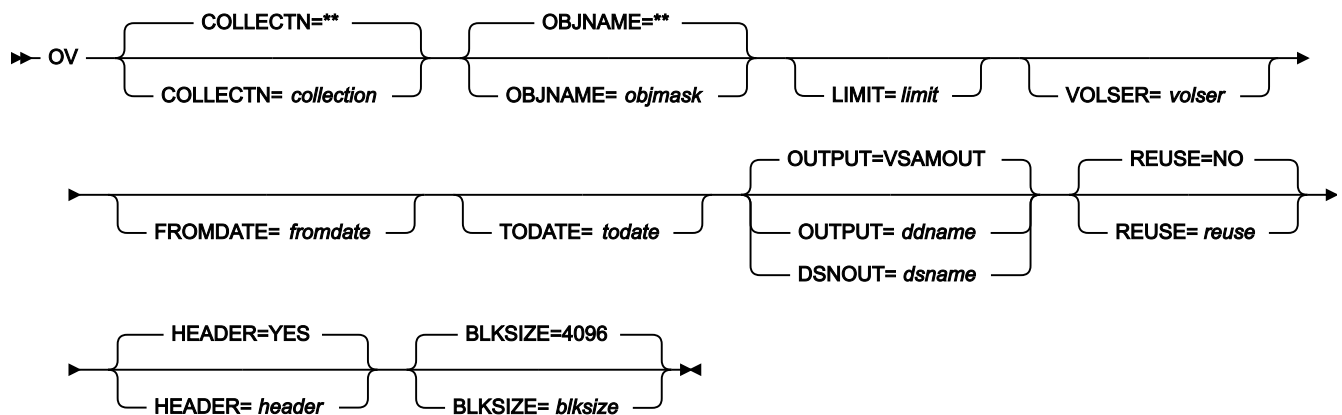
Figure 457. Syntax
