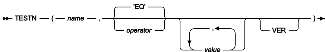
Figure 536. Syntax
