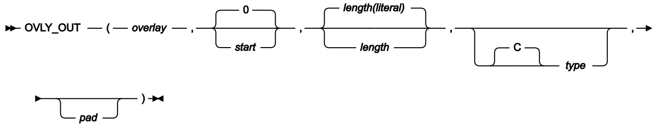
Figure 512. Syntax
