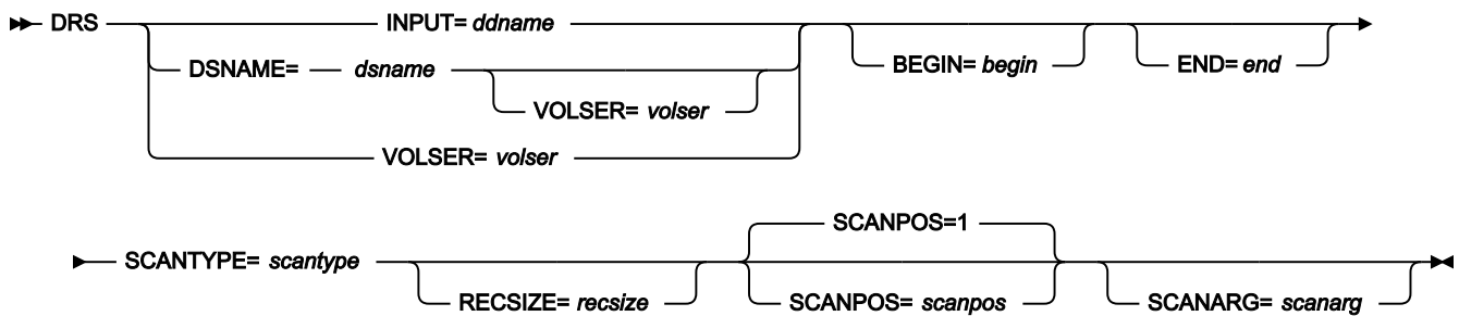
Figure 426. Syntax
