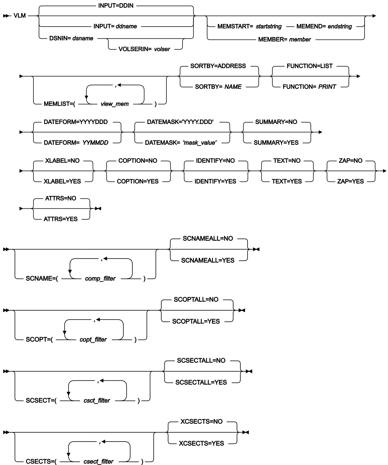
Figure 481. Syntax
