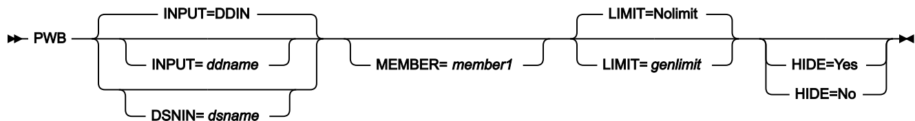
Figure 459. Syntax
