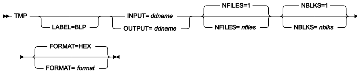
Figure 470. Syntax
