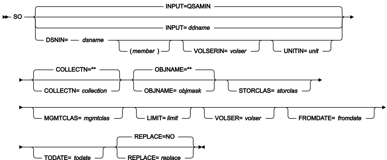
Figure 466. Syntax
