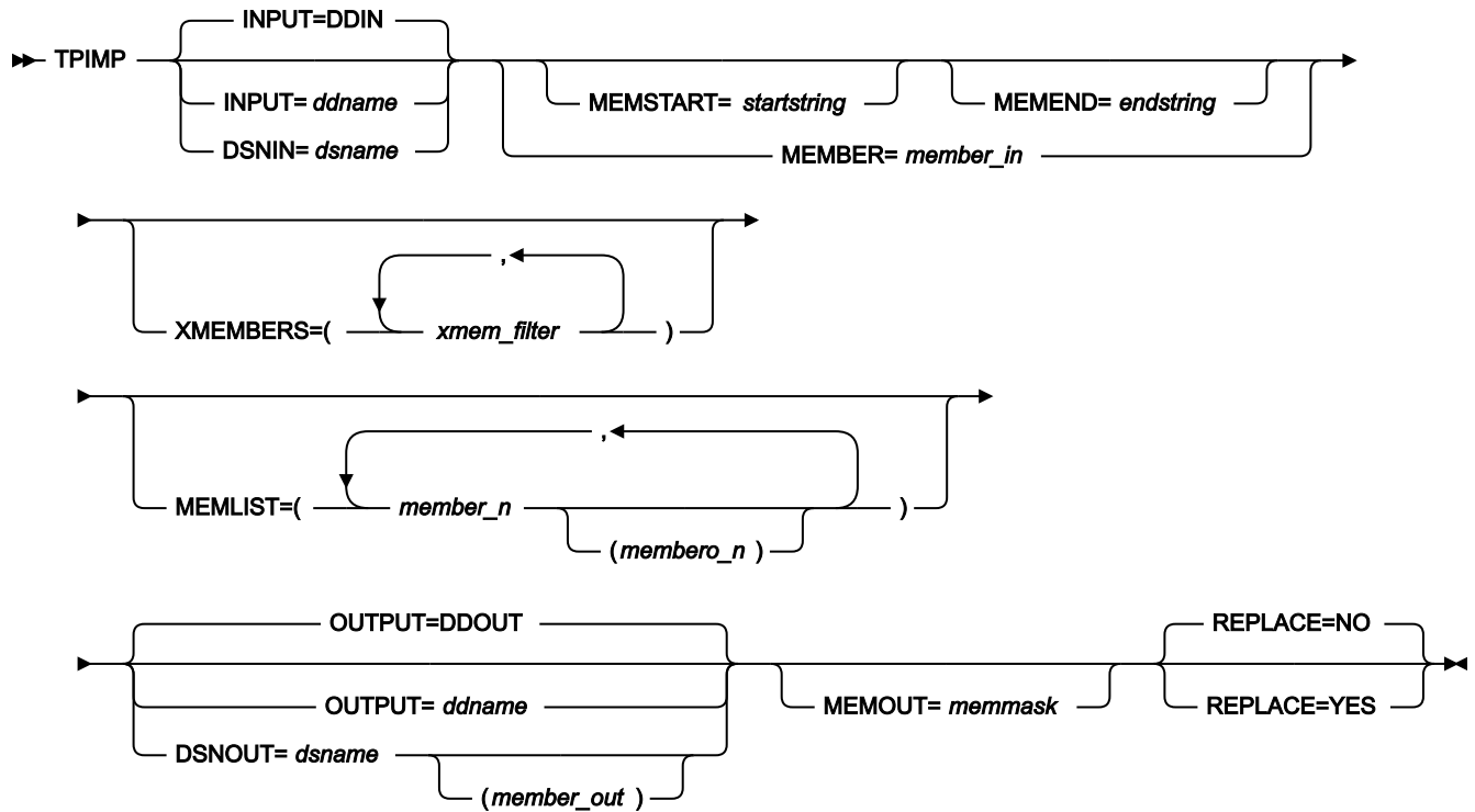
Figure 473. Syntax
