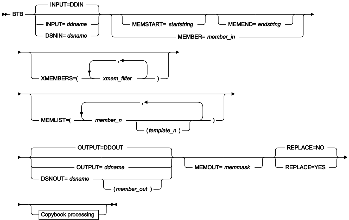
Figure 421. Syntax
