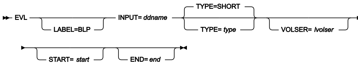
Figure 445. Syntax
