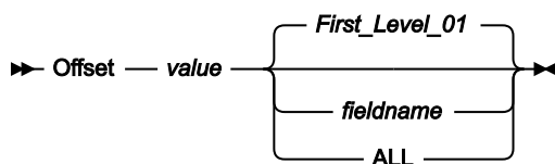
Figure 219. Syntax
