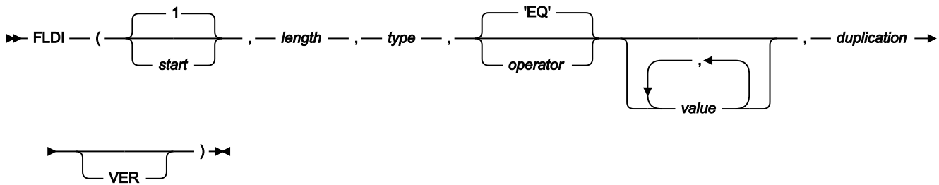
Figure 504. Syntax
