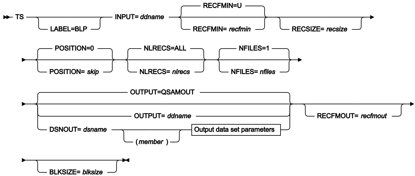
Figure 475. Syntax
