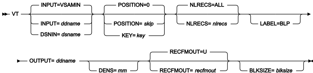
Figure 483. Syntax
