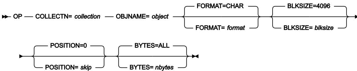
Figure 455. Syntax
