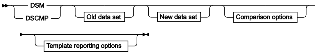
Figure 437. Syntax
