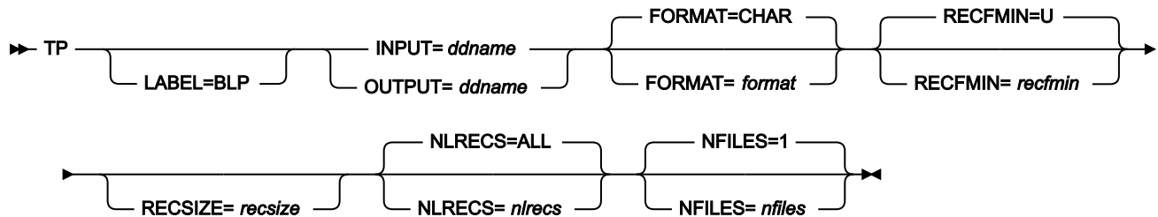
Figure 471. Syntax
