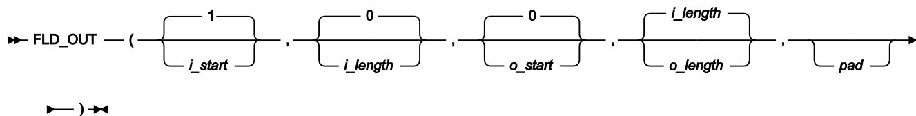
Figure 501. Syntax
