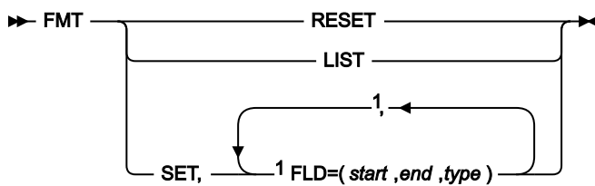
Figure 447. Syntax
