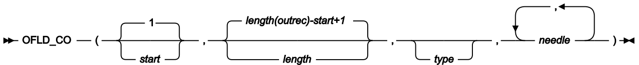
Figure 511. Syntax
