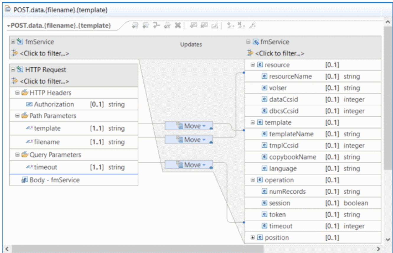
Figure 175. Generic request example: mapping API data in the request schema
