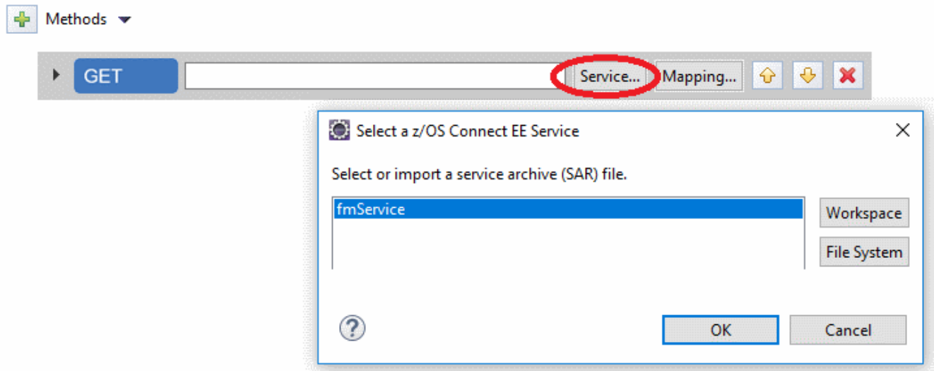
Figure 174. Associating the API with a File Manager service
