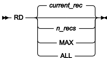
Figure 398. Syntax - View and Edit
