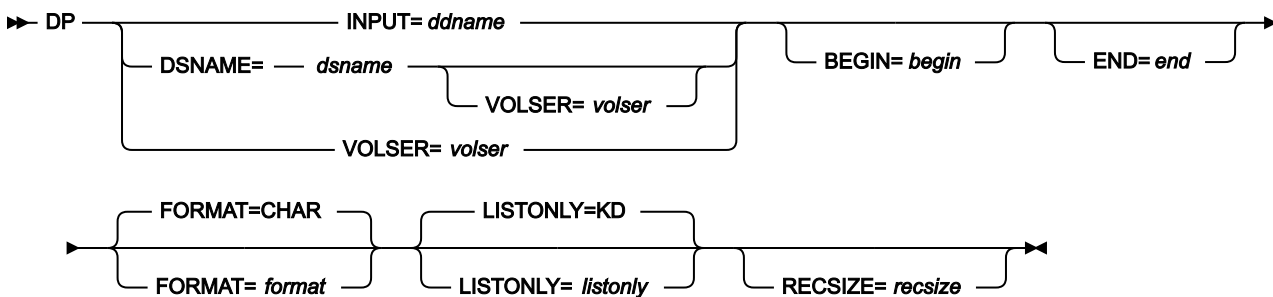
Figure 425. Syntax
