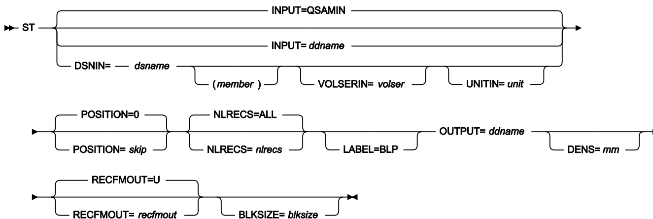
Figure 467. Syntax
