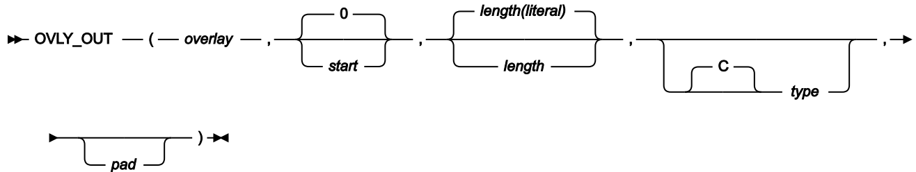
Figure 512. Syntax
