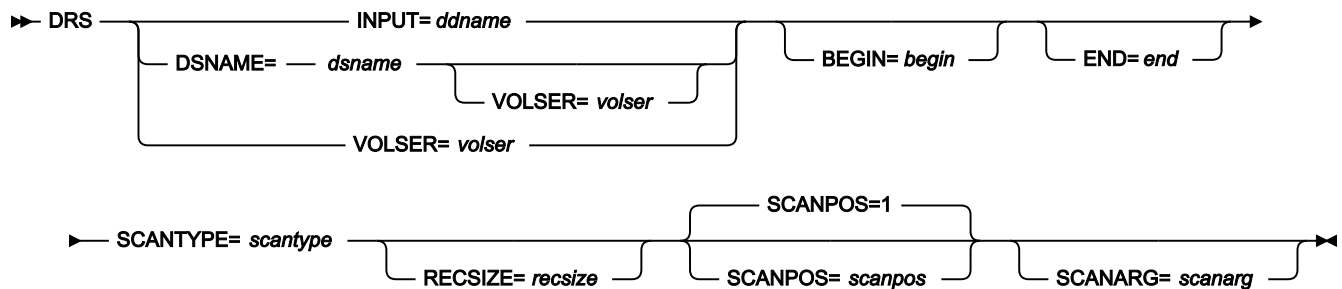
Figure 426. Syntax
