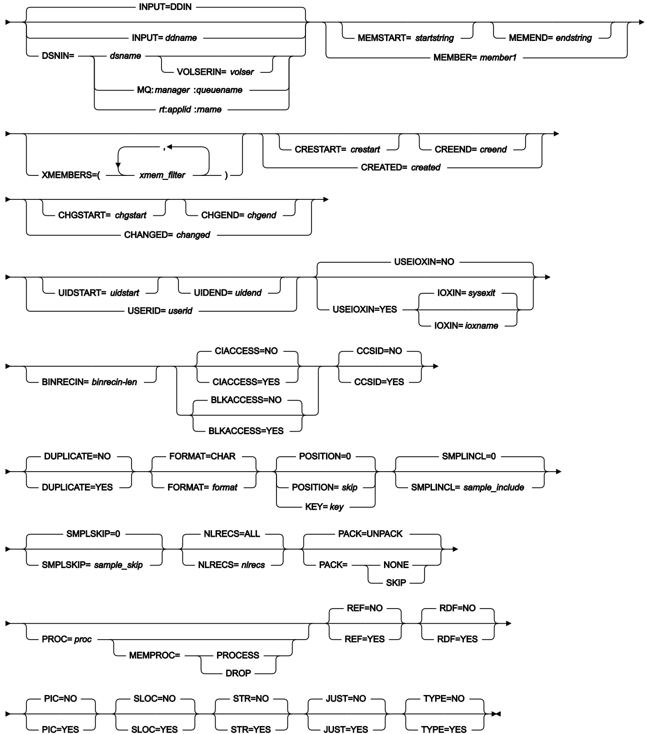
Figure 438. Syntax
