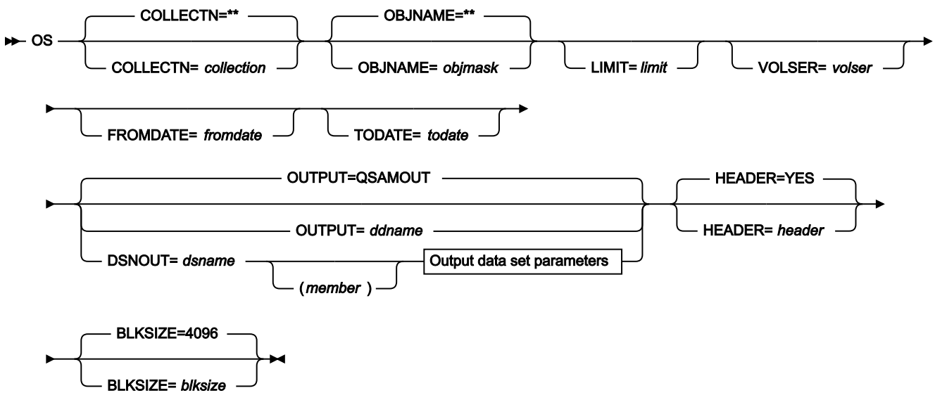
Figure 456. Syntax
