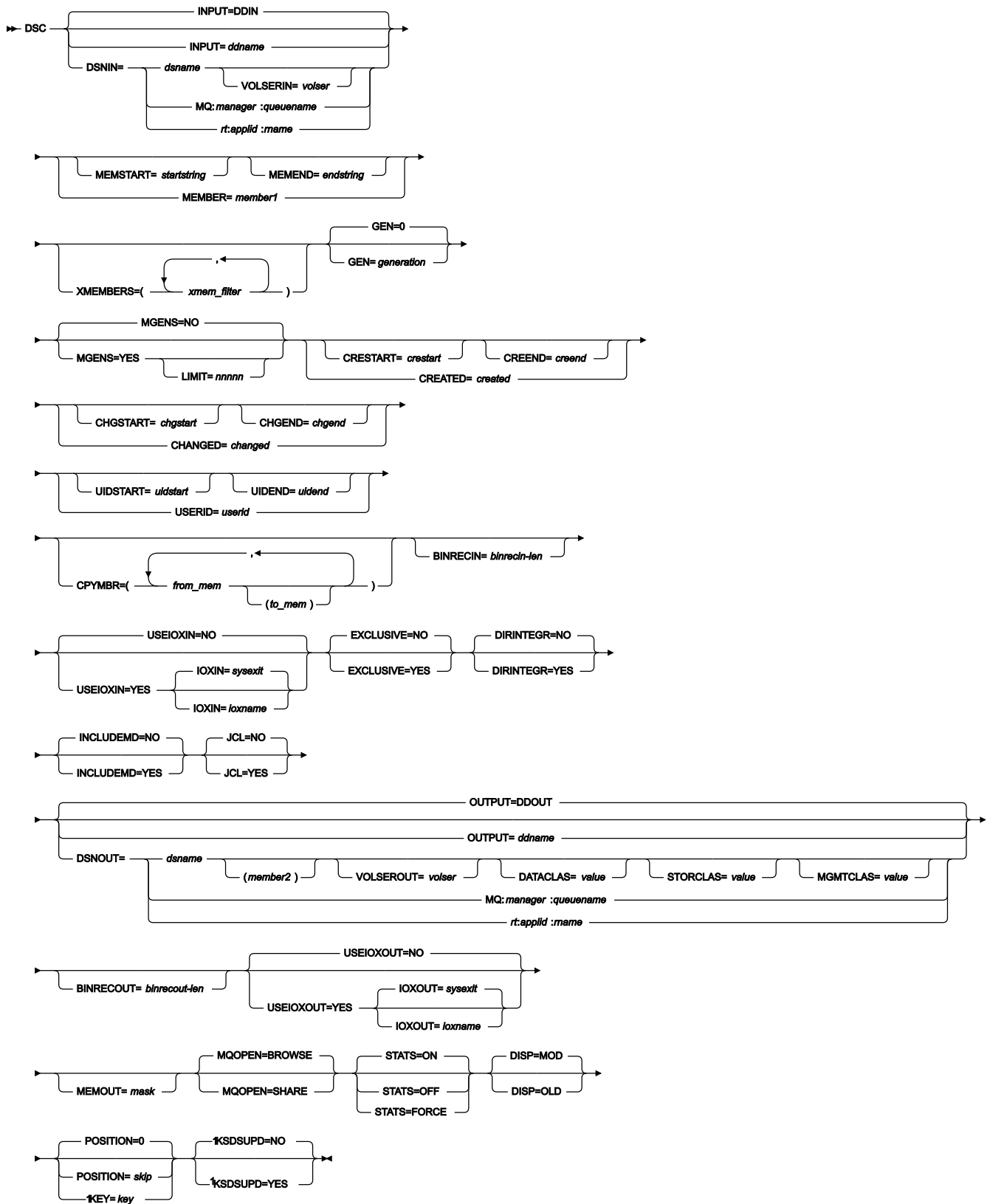
Figure 428. Syntax
