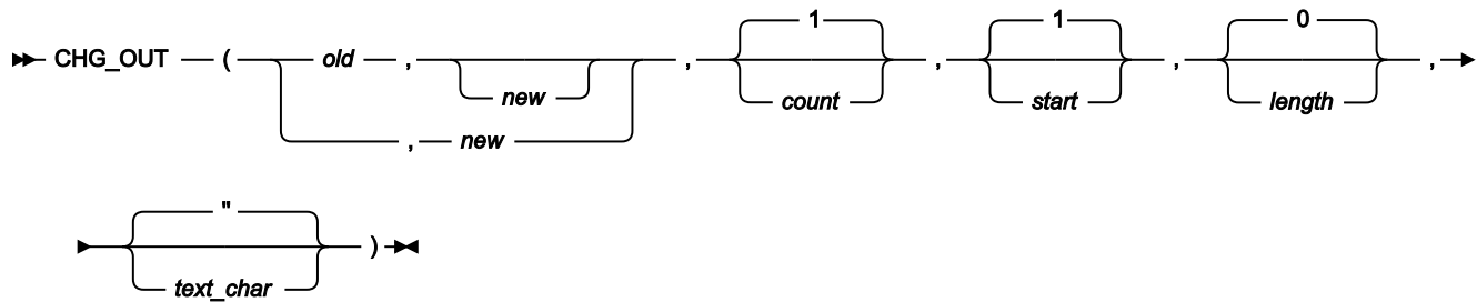
Figure 490. Syntax
