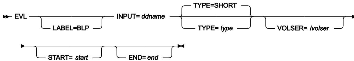
Figure 445. Syntax
