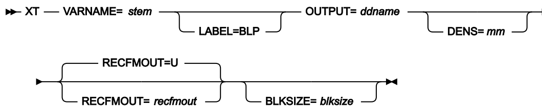
Figure 486. Syntax
