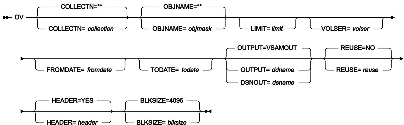
Figure 457. Syntax
