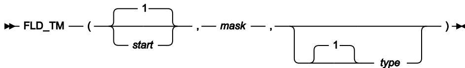
Figure 502. Syntax
