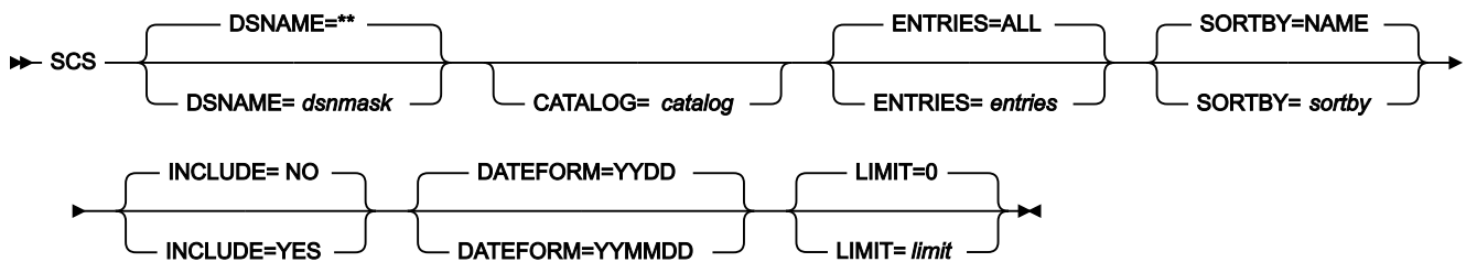
Figure 462. Syntax
