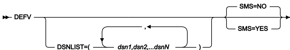
Figure 424. Syntax
