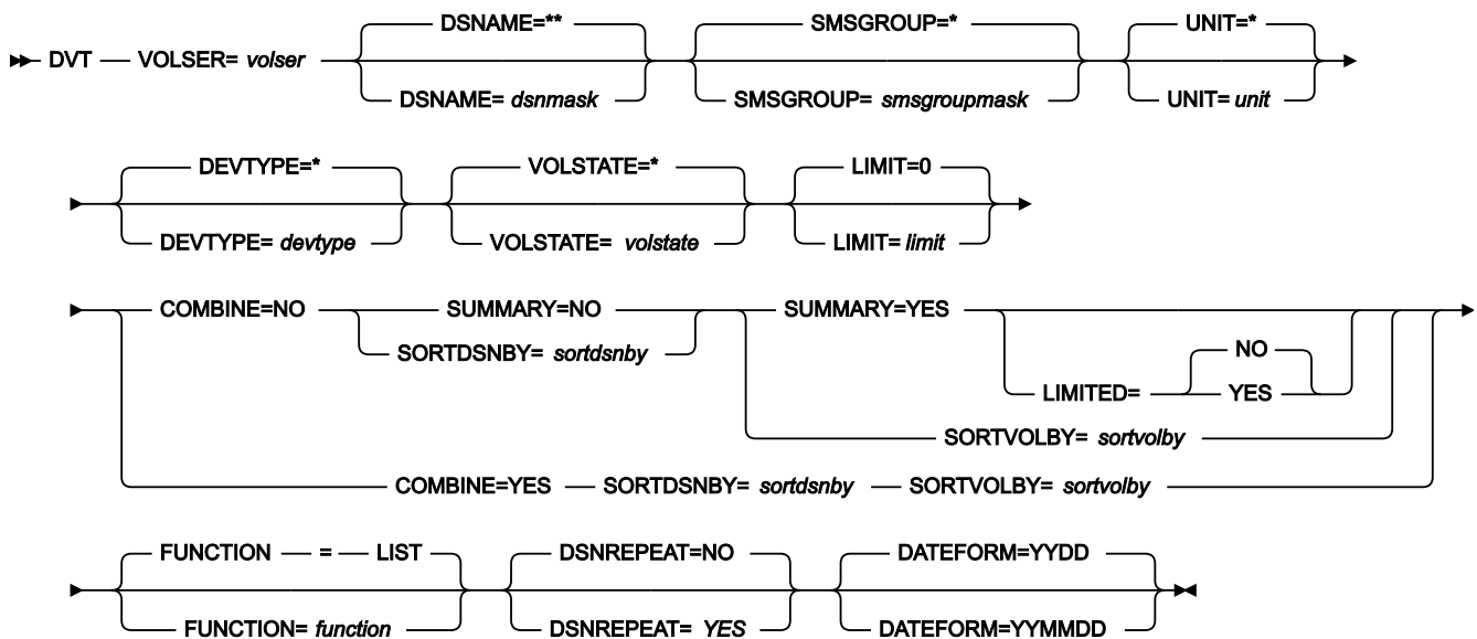
Figure 442. Syntax
