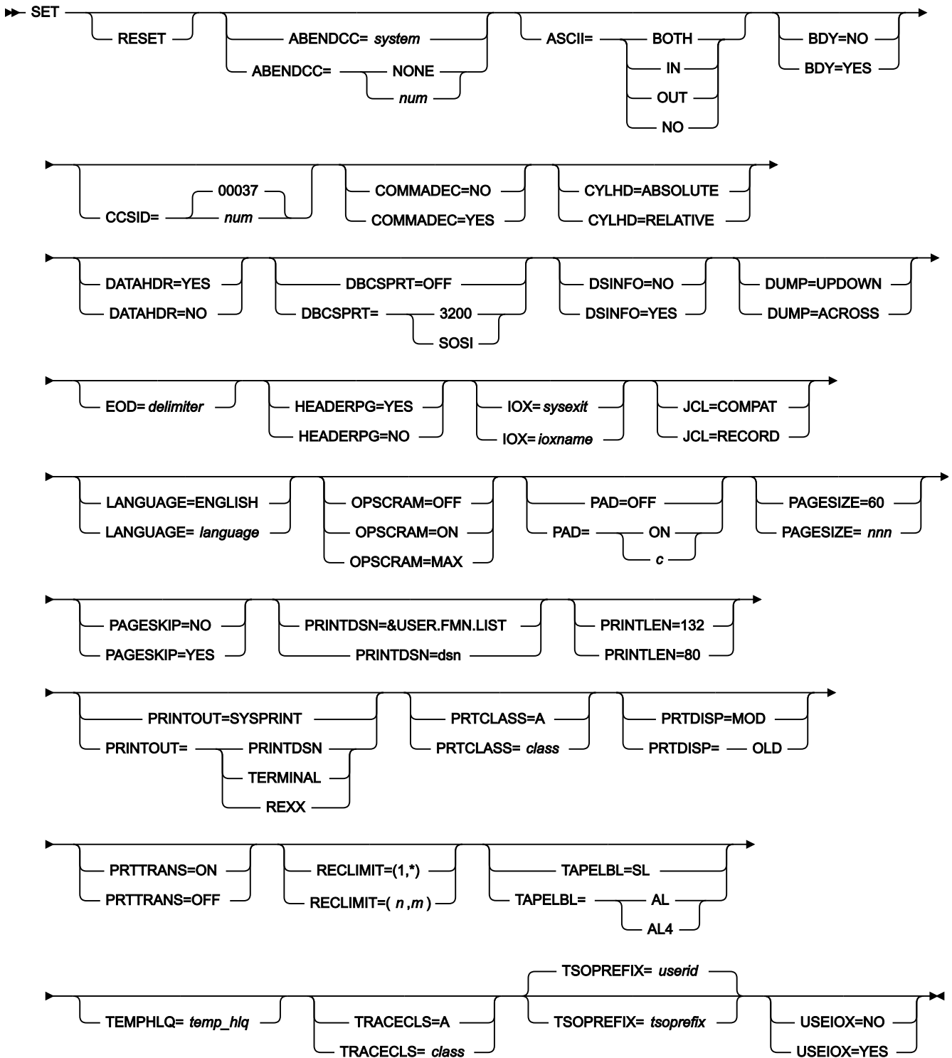
Figure 463. Syntax
