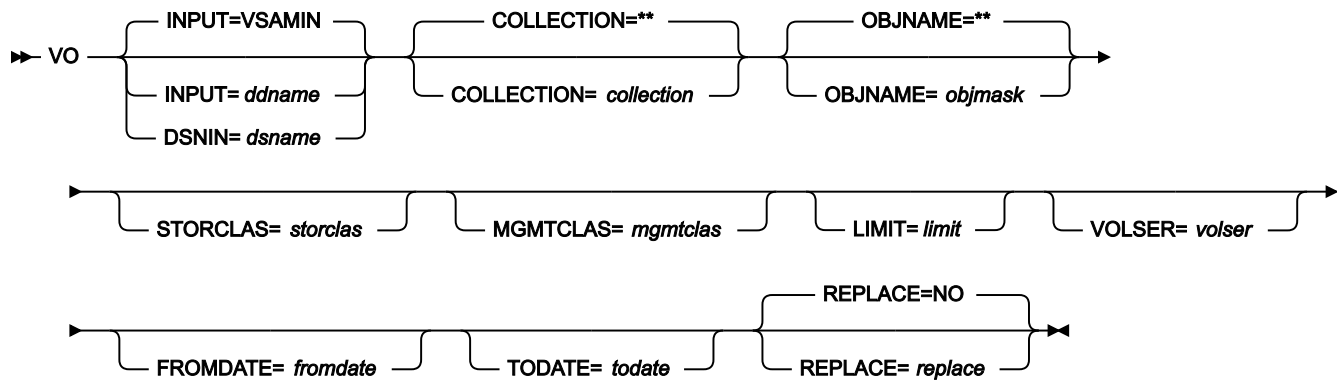
Figure 482. Syntax
