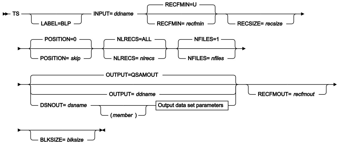
Figure 475. Syntax
