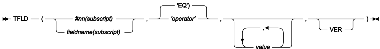
Figure 537. Syntax
