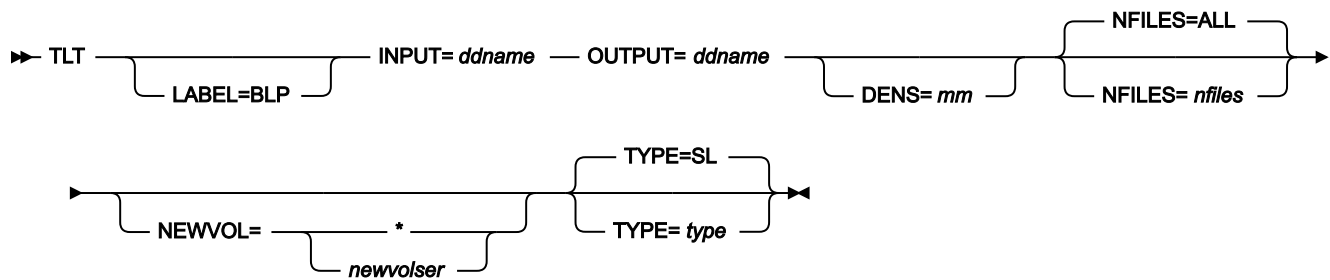
Figure 469. Syntax
