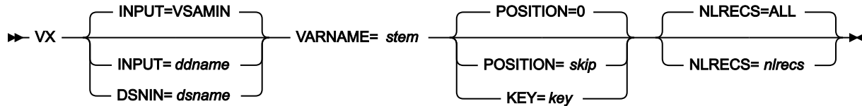
Figure 484. Syntax
