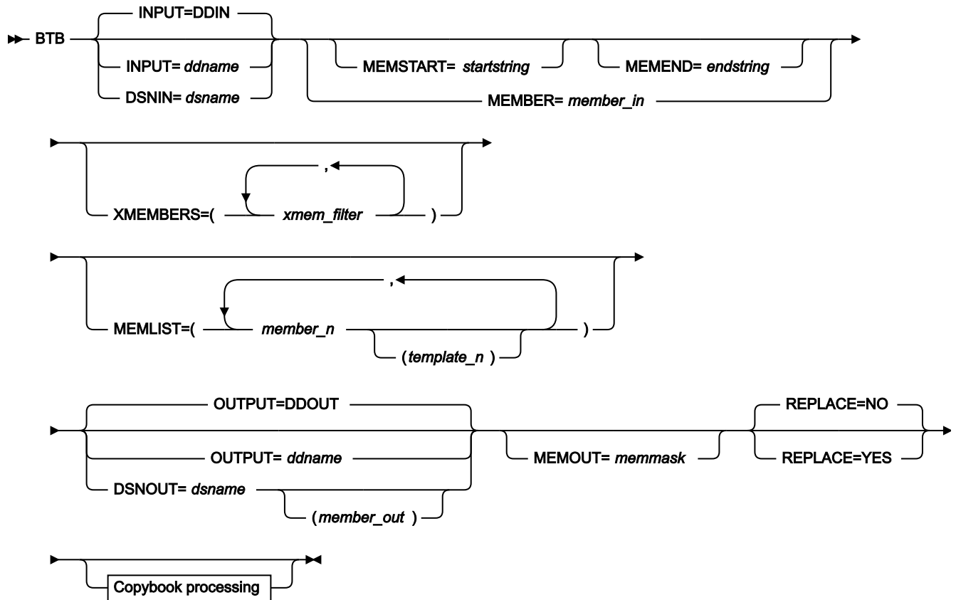
Figure 421. Syntax
