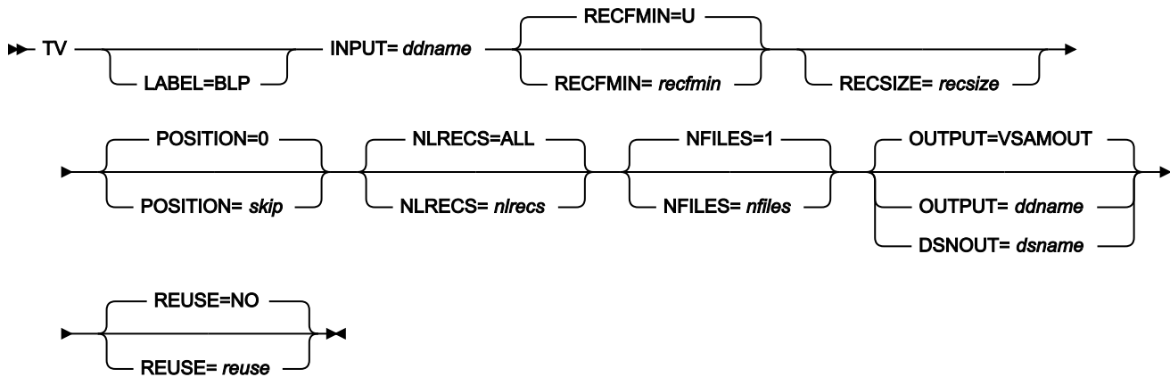
Figure 479. Syntax
