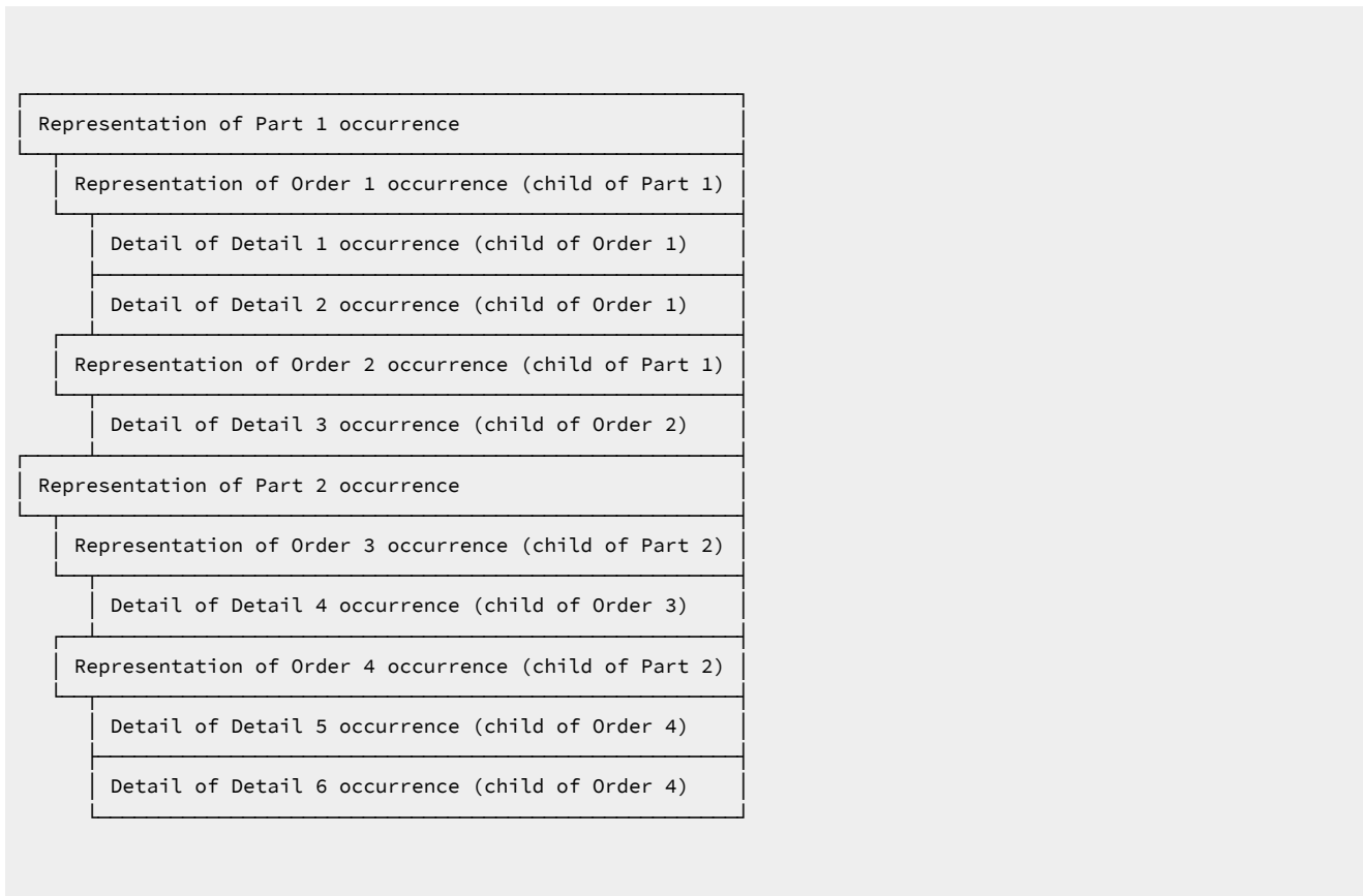
Figure 5. DETAILS occurrences with parent segments
