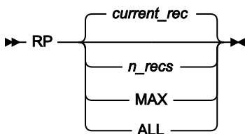
Figure 403. Syntax
