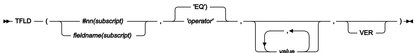
Figure 535. Syntax
