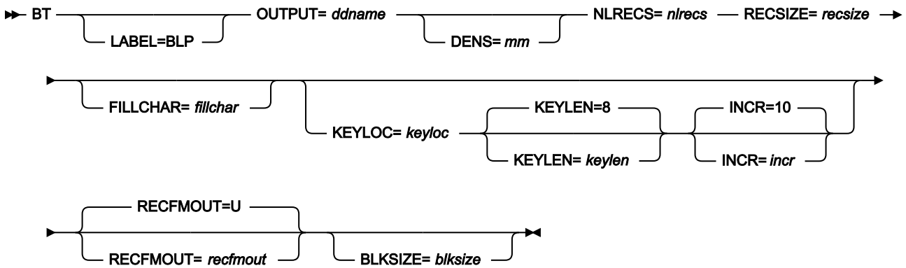
Figure 418. Syntax
