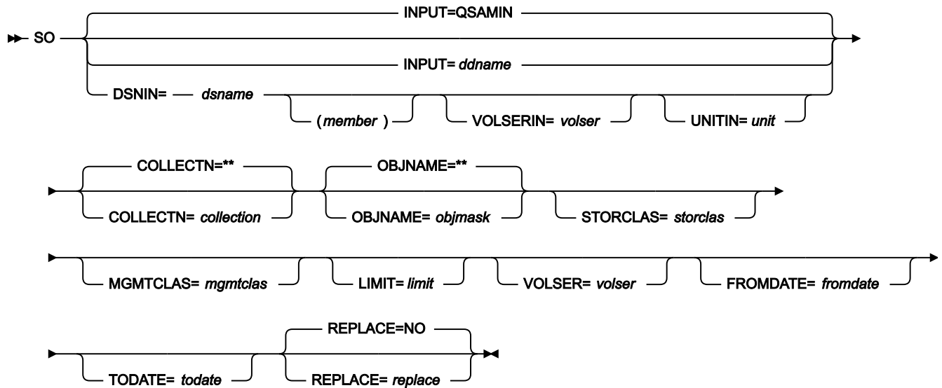
Figure 464. Syntax
