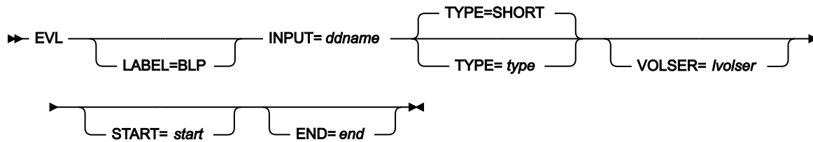
Figure 443. Syntax
