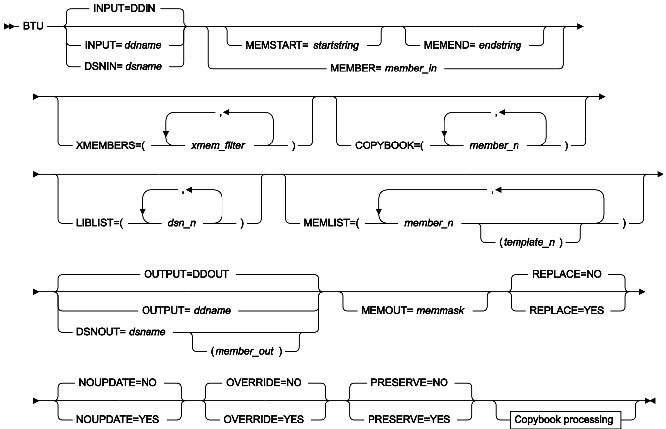
Figure 420. Syntax
