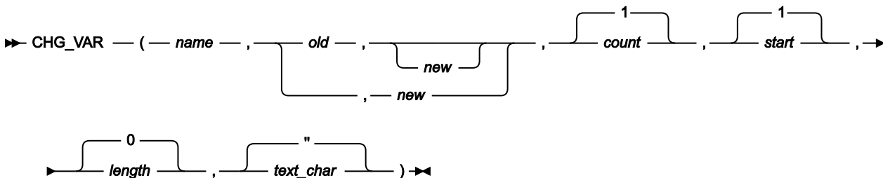
Figure 489. Syntax
