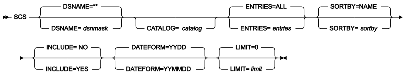
Figure 460. Syntax
