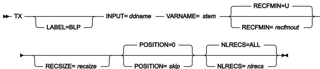
Figure 478. Syntax
