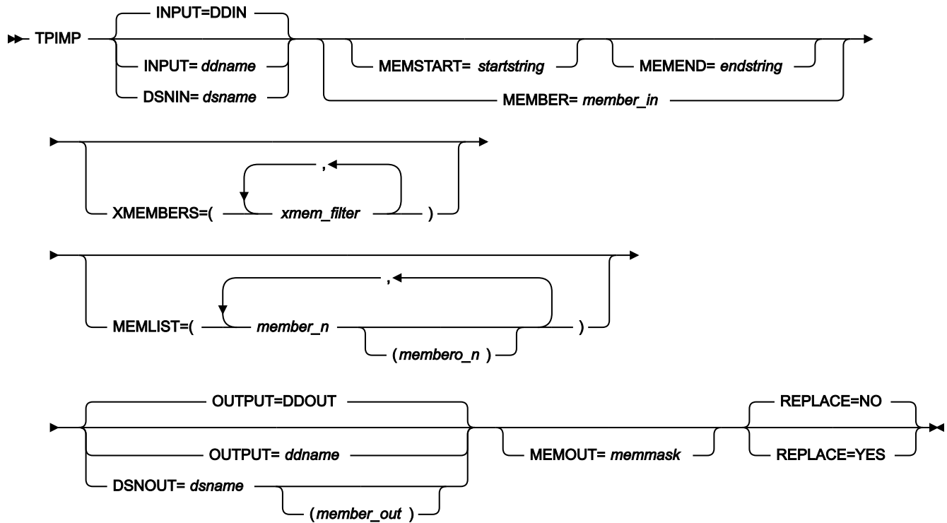
Figure 471. Syntax
