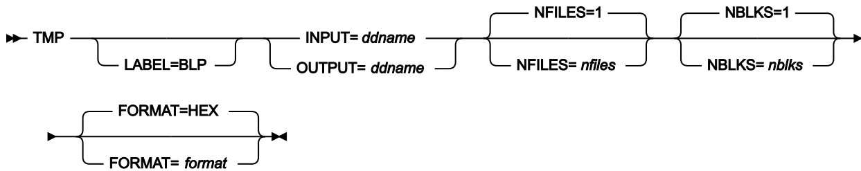
Figure 468. Syntax
