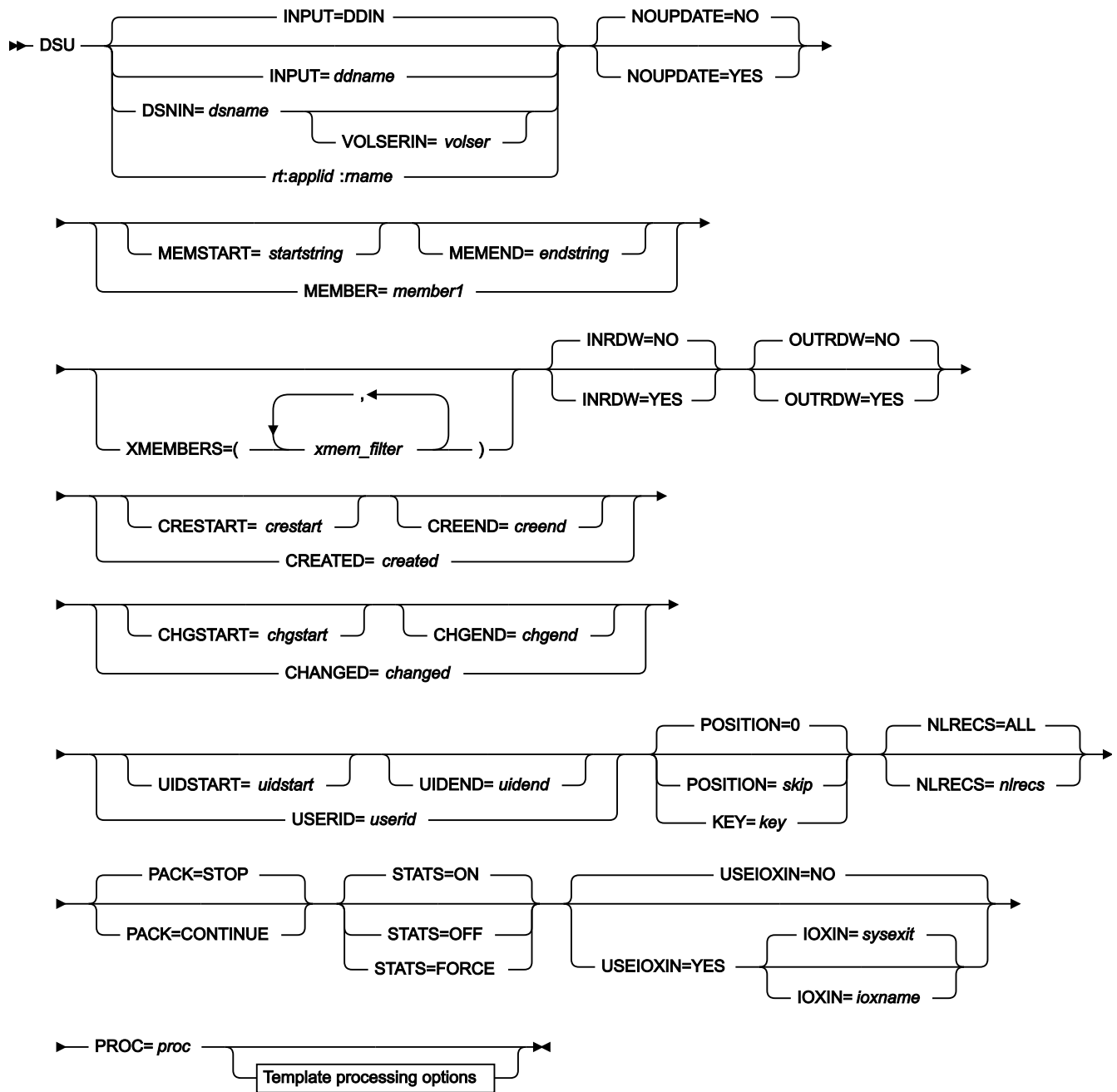
Figure 437. Syntax
