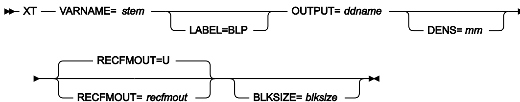
Figure 484. Syntax
