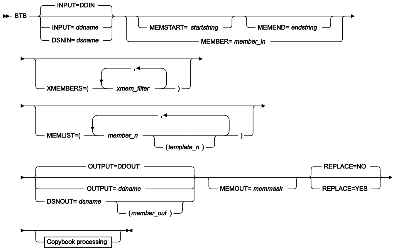
Figure 419. Syntax
