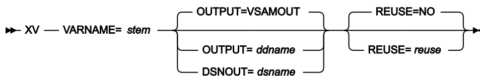
Figure 485. Syntax
