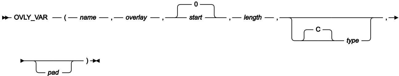
Figure 511. Syntax
