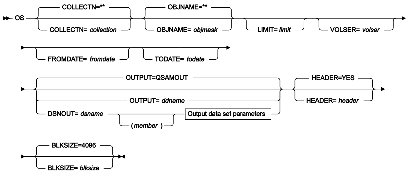
Figure 454. Syntax
