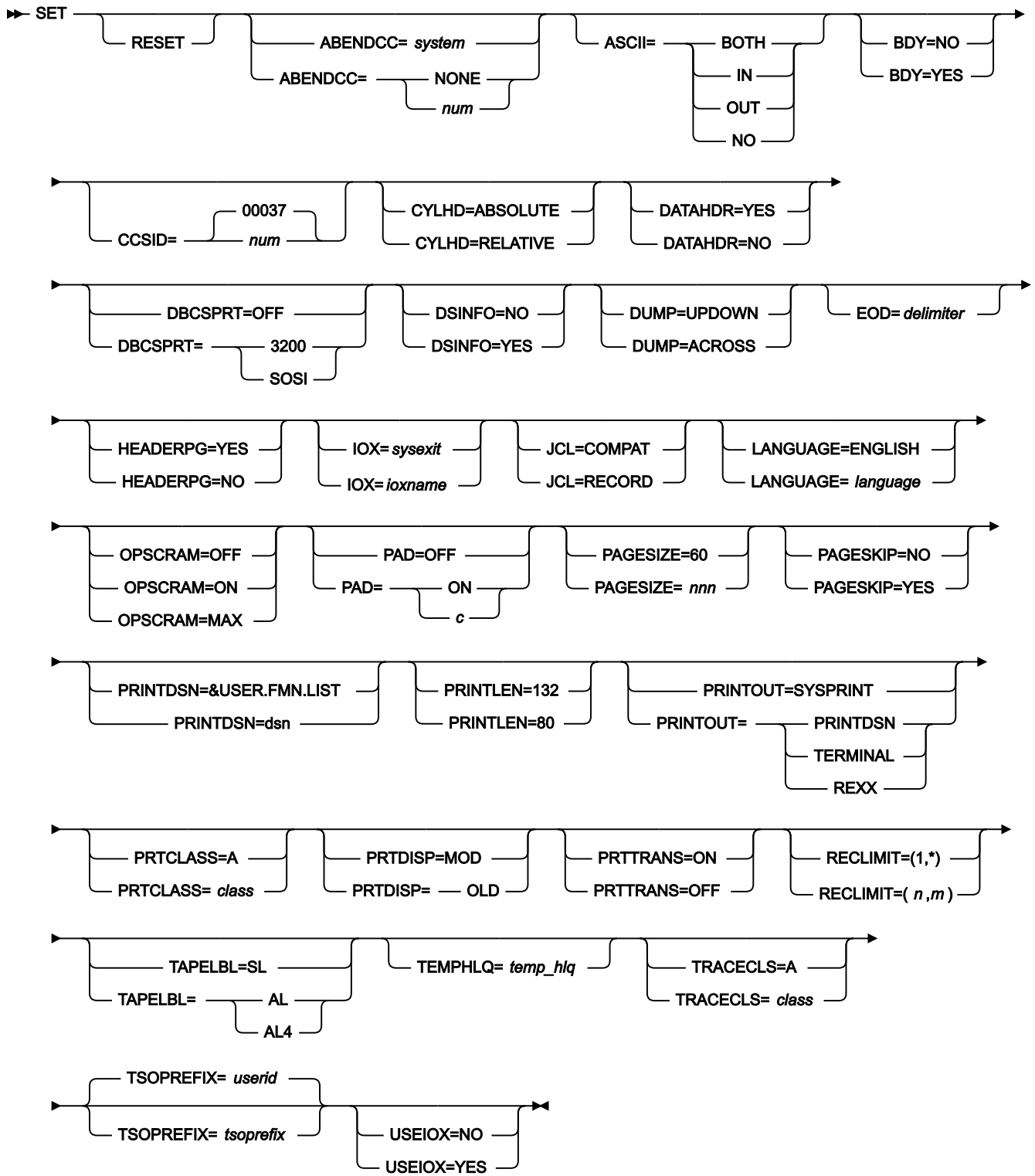
Figure 461. Syntax
