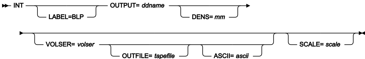
Figure 448. Syntax
