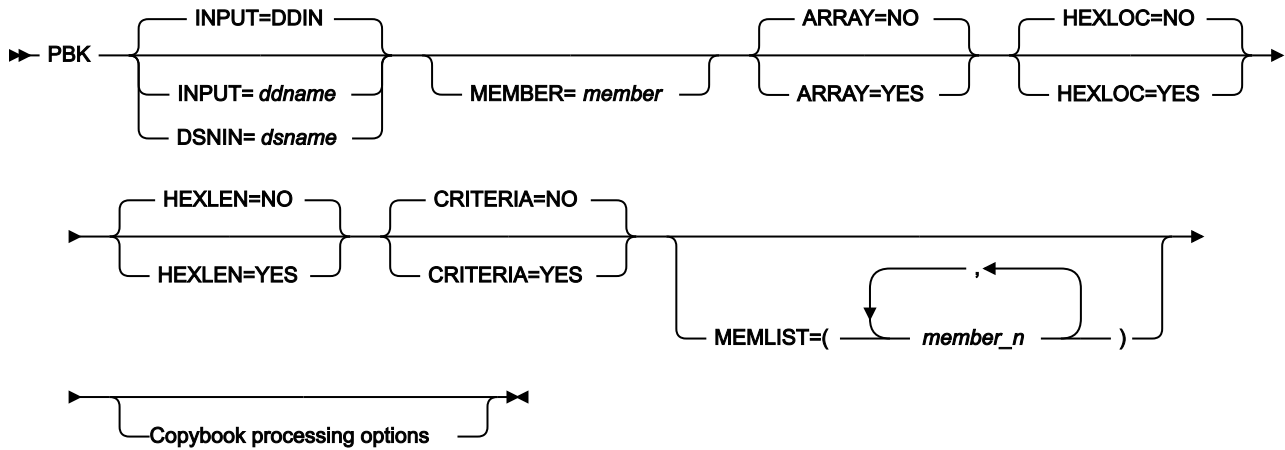
Figure 456. Syntax
