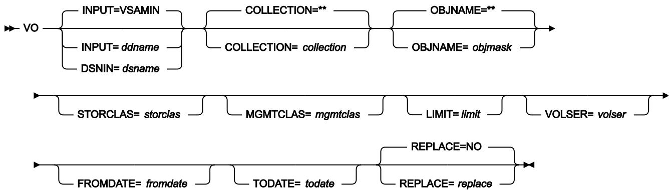
Figure 480. Syntax
