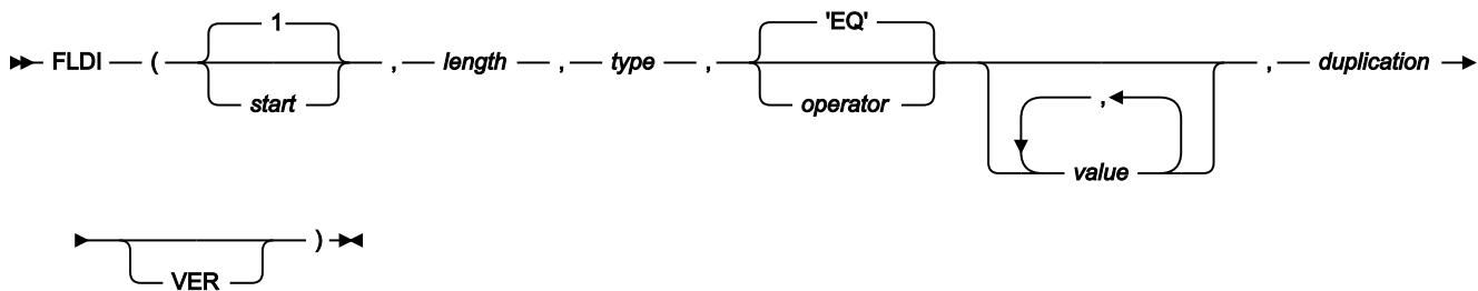
Figure 502. Syntax
