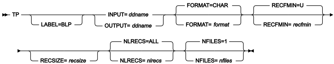
Figure 469. Syntax
