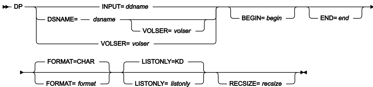
Figure 423. Syntax
