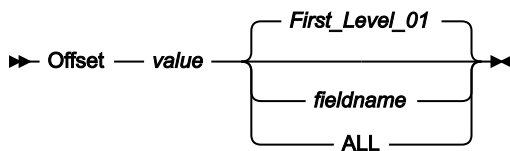
Figure 217. Syntax
