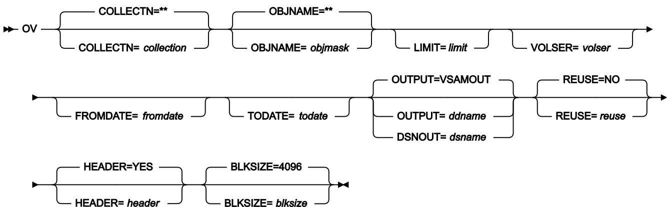
Figure 455. Syntax
