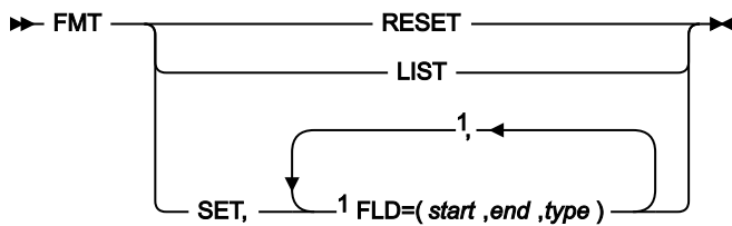
Figure 445. Syntax
