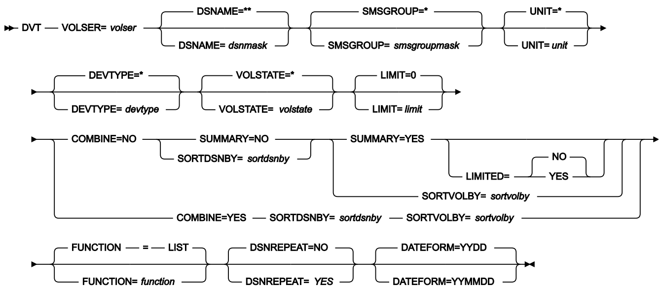
Figure 440. Syntax
