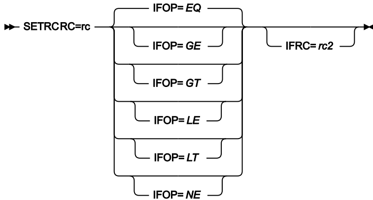
Figure 463. Syntax
