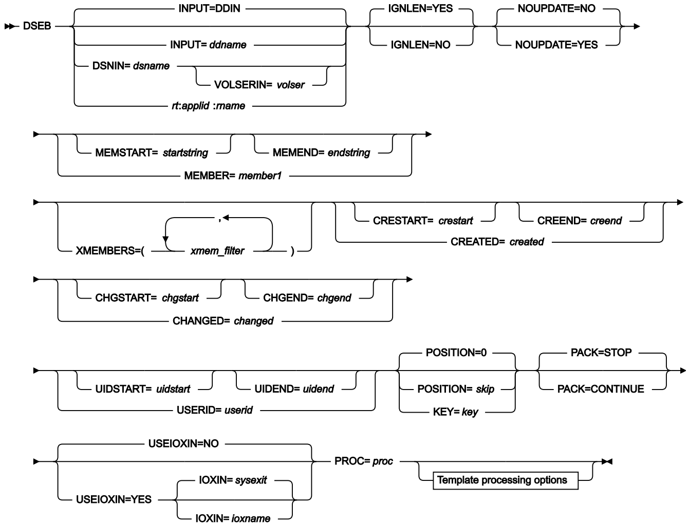
Figure 428. Syntax
