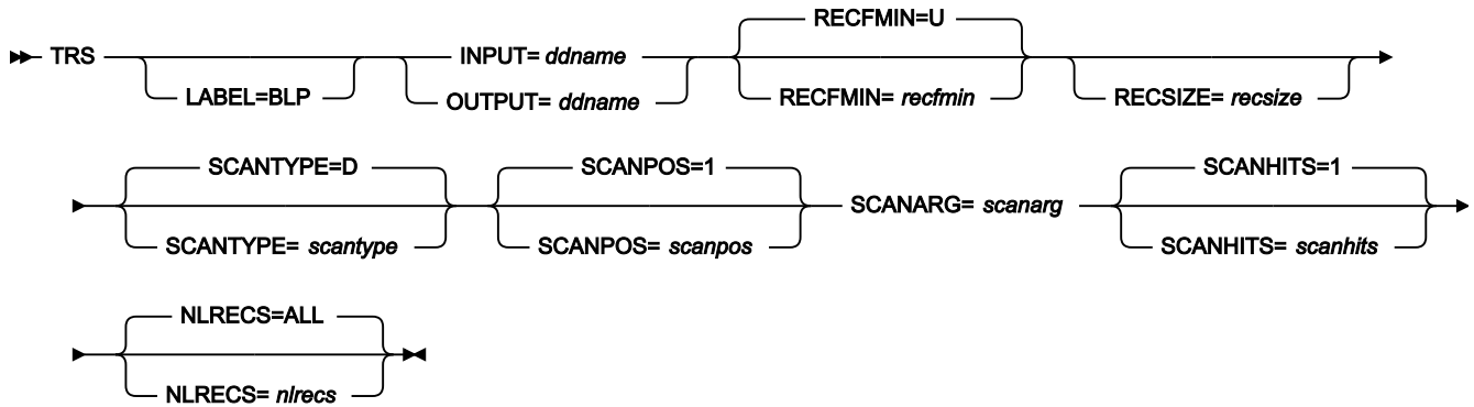
Figure 472. Syntax
