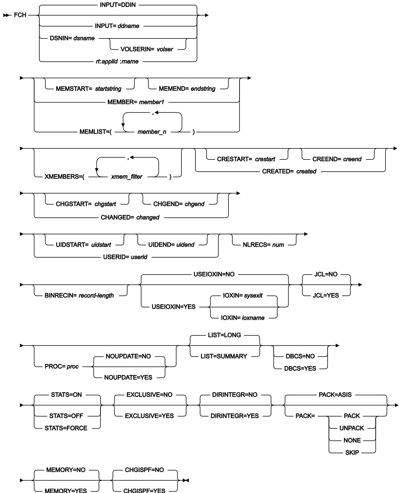
Figure 444. Syntax
