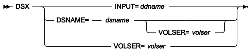
Figure 439. Syntax
