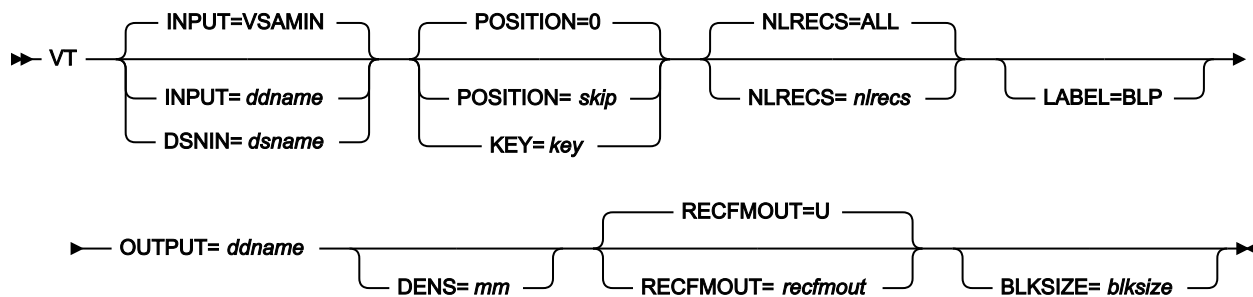
Figure 481. Syntax
