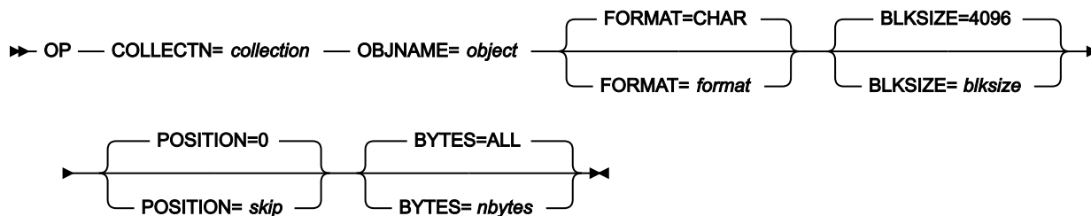
Figure 453. Syntax
