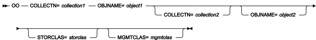
Figure 452. Syntax
