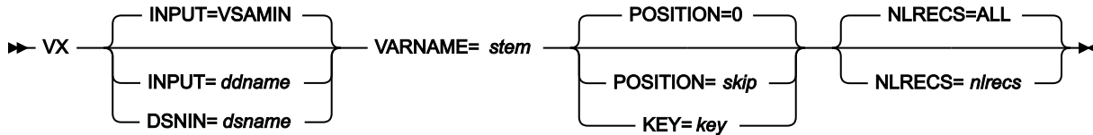
Figure 482. Syntax
