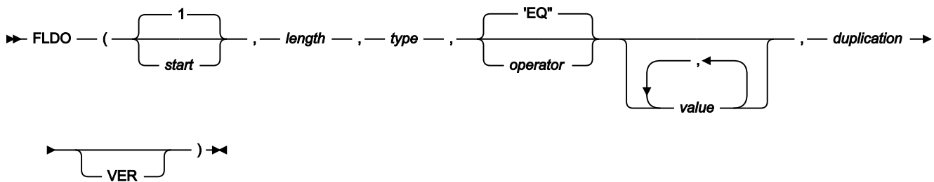
Figure 503. Syntax
