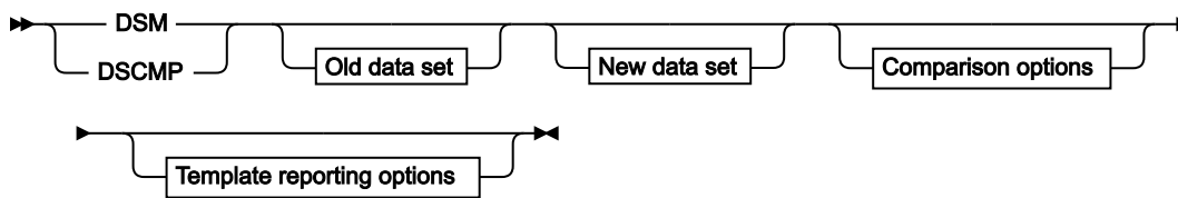
Figure 435. Syntax
