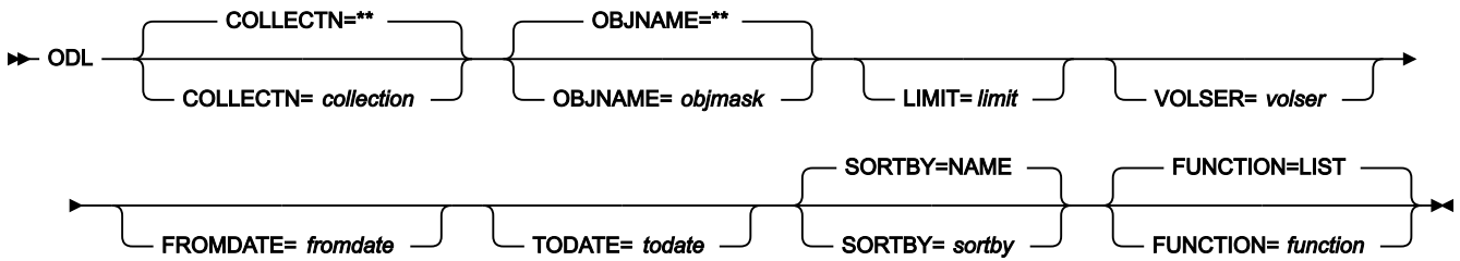
Figure 450. Syntax
