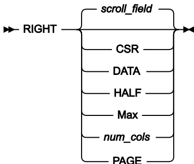
Figure 170. Template editing
