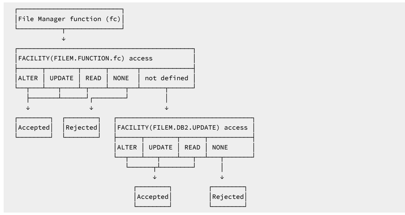
Figure 15. Security system validation for update functions
