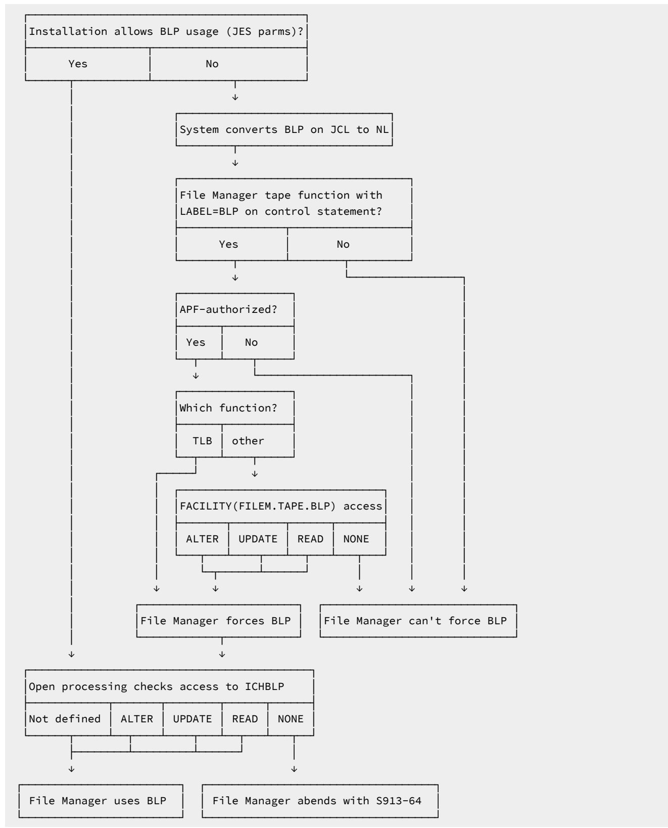
Figure 13. BLP processing by File Manager
