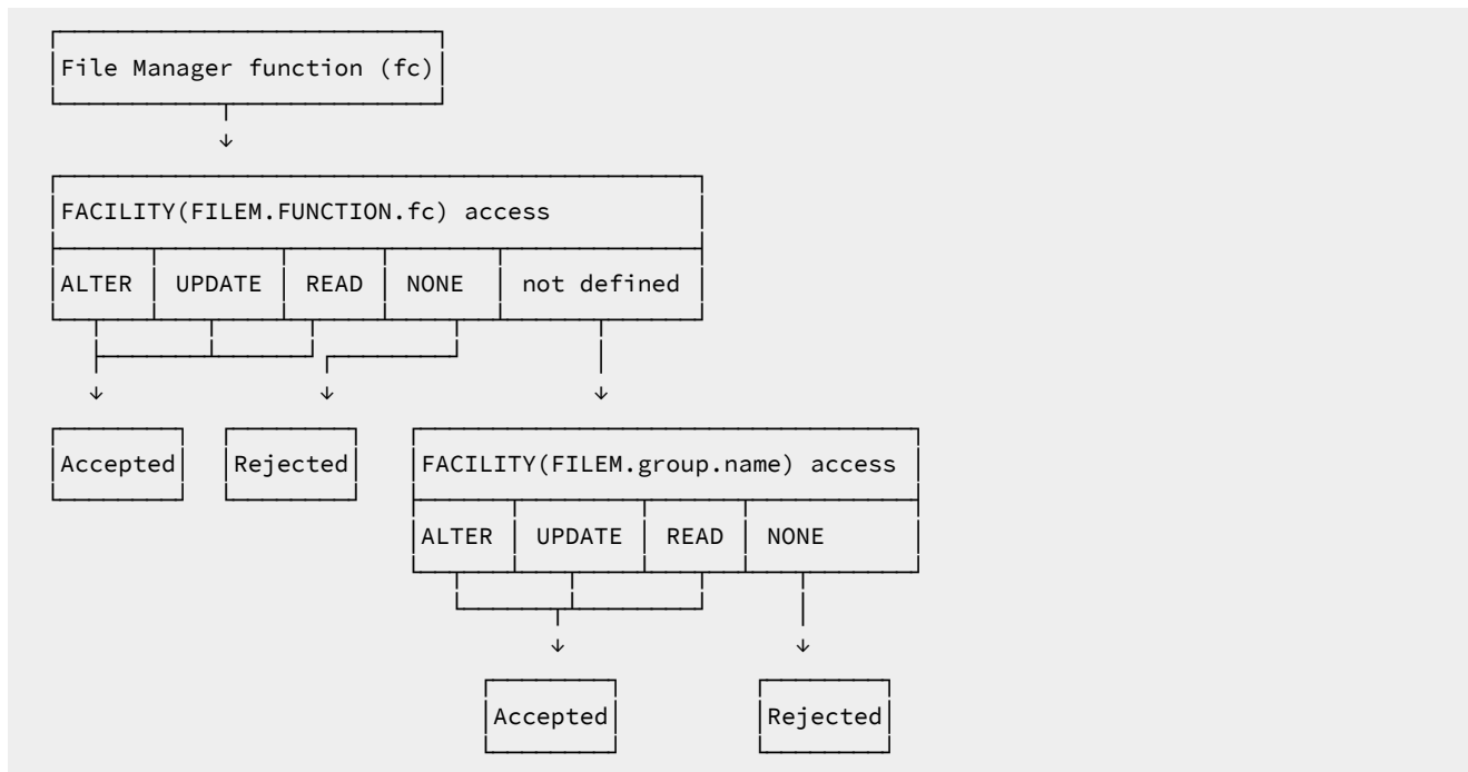
Figure 10. Access to File Manager functions
