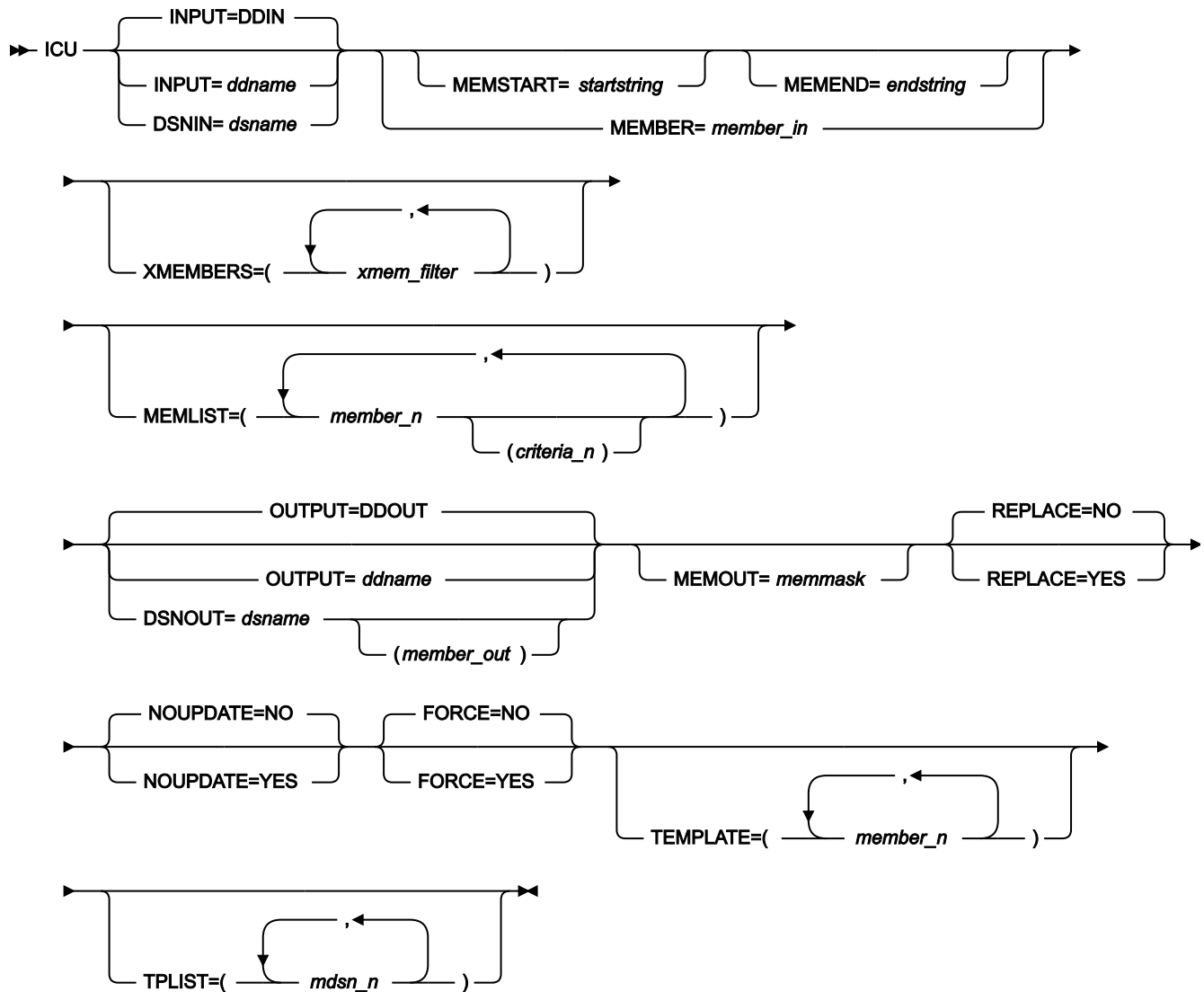
Figure 139. Syntax
