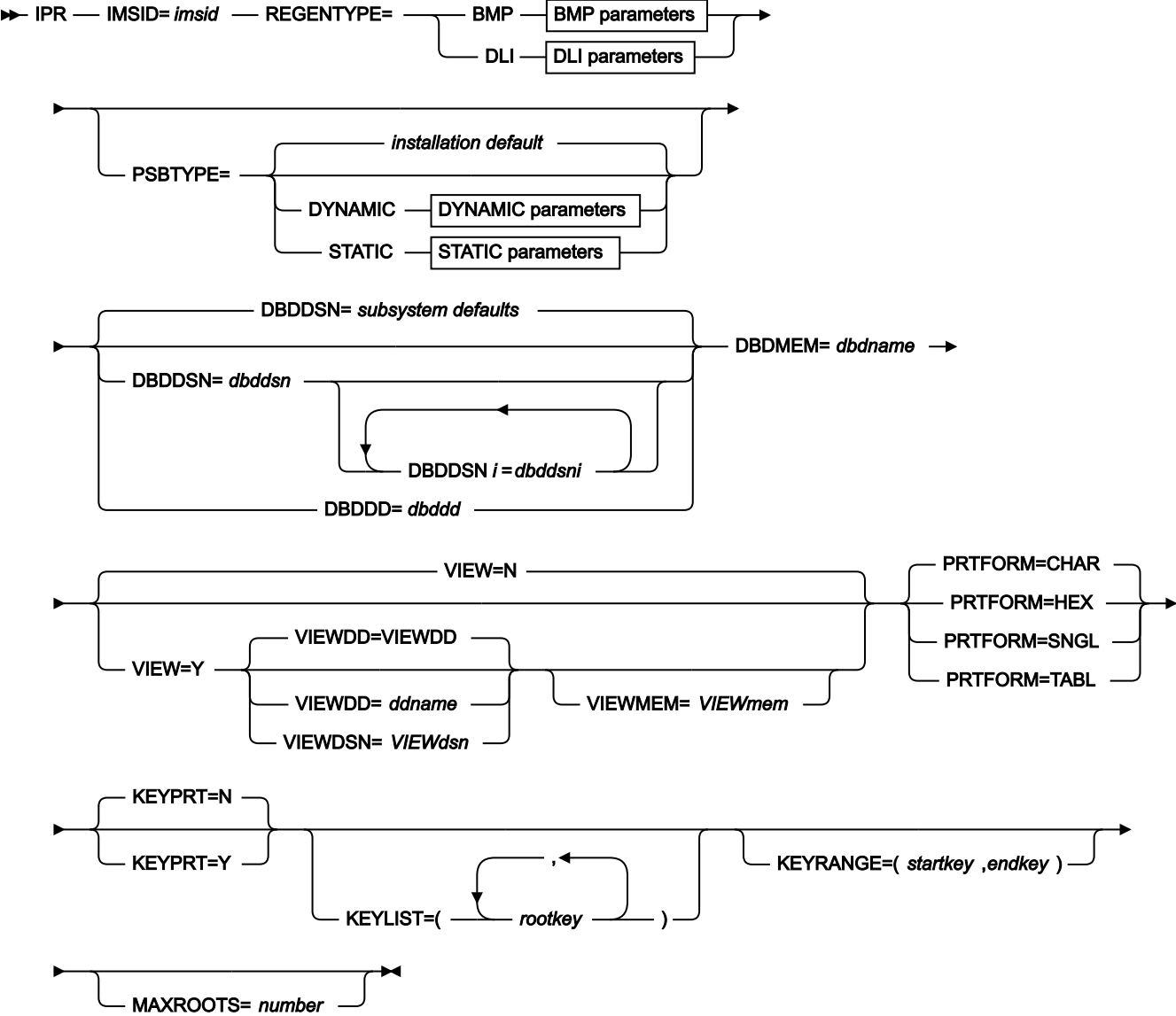
Figure 150. Syntax
