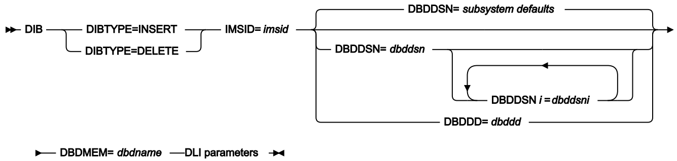
Figure 171. Syntax
