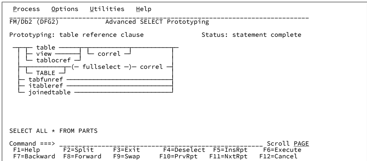
Figure 112. Advanced SELECT prototyping: the completed statement (example 1)
