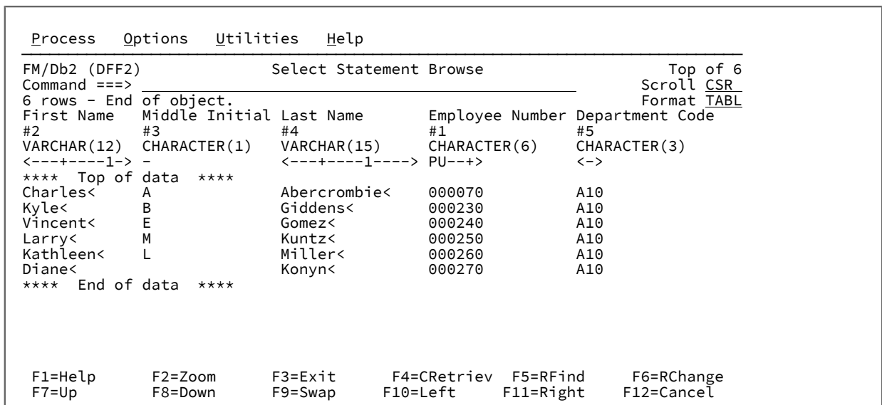
Figure 37. Select Statement Browse panel
