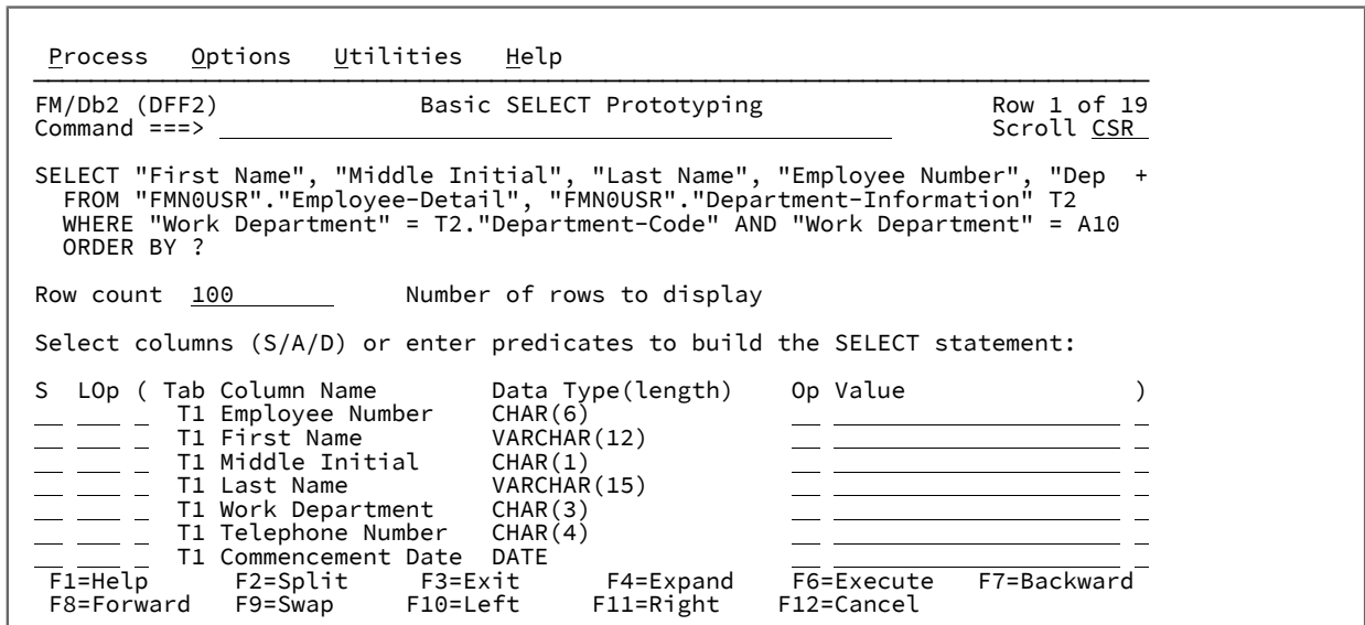
Figure 36. Basic SELECT Prototyping panel (6)
