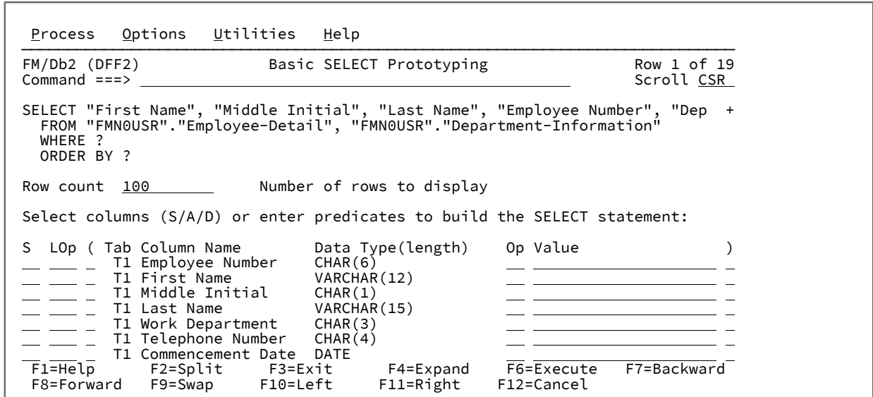
Figure 33. Basic SELECT Prototyping panel (3)
