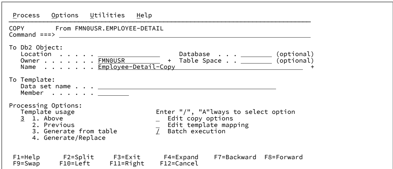
Figure 40. Basic SELECT Prototyping panel (2)
