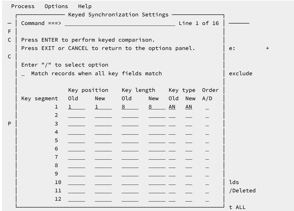
Figure 203. Keyed Synchronization Settings panel - no key segment information
