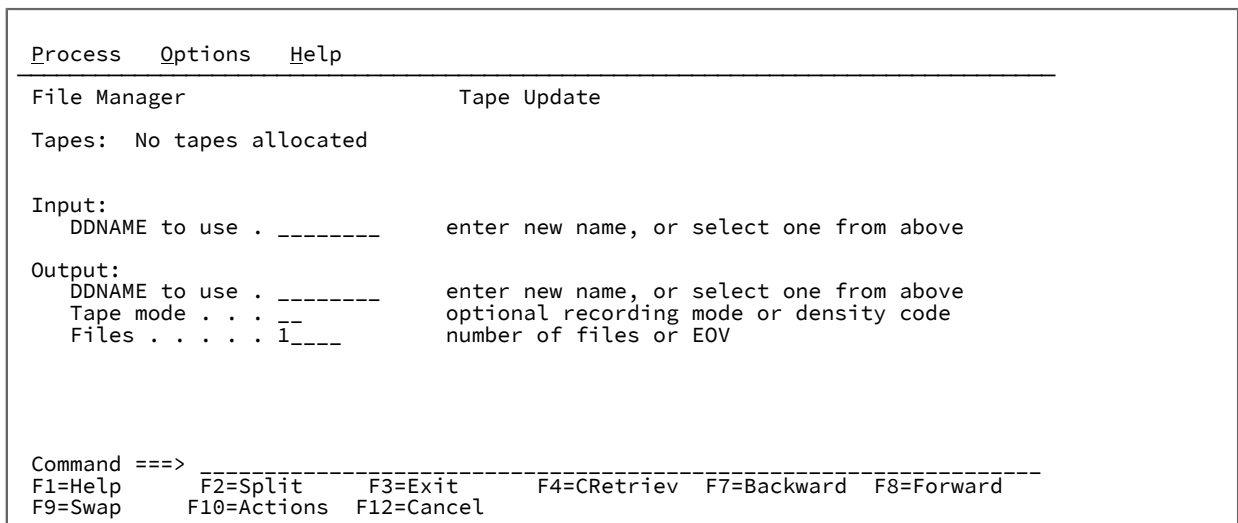
Figure 121. Tape Update panel
