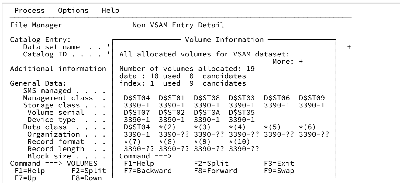
Figure 103. Volume Information panel
