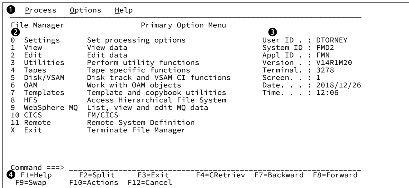
Figure 287. File Manager Primary Option Menu panel
