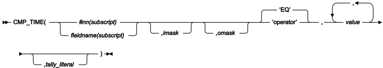
Figure 492. CMP_TIME syntax – with template
