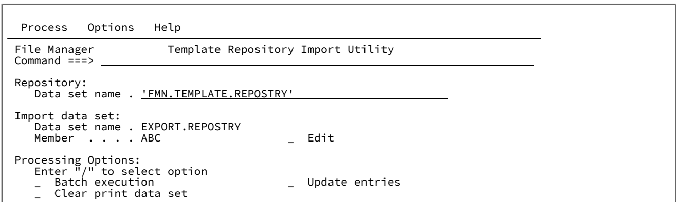
Figure 63. Template Repository Import Utility panel
