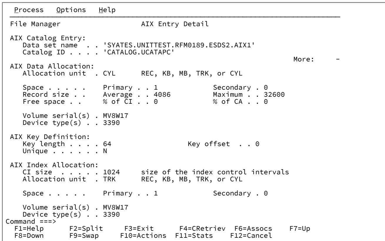
Figure 184. (Part 2 of 2) AIX® Entry Detail panel
