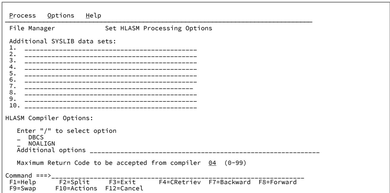
Figure 310. Set HLASM Processing Options
