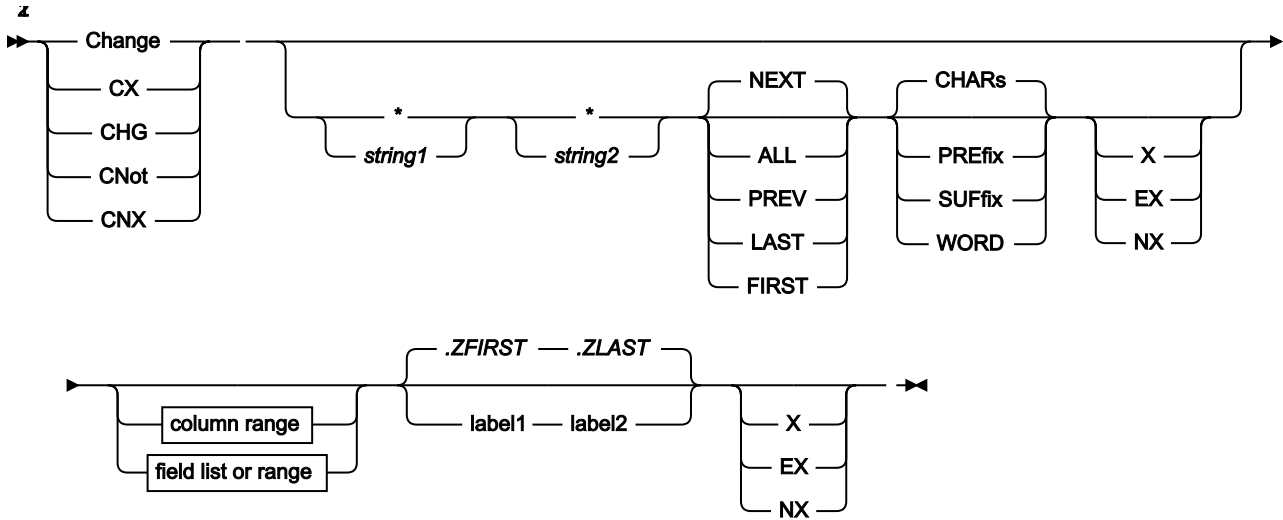
Figure 371. Syntax in the Editor
