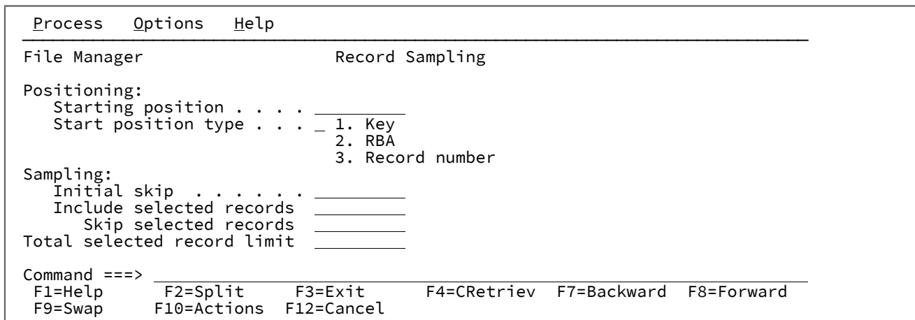
Figure 294. Record Sampling panel, when a template is used
