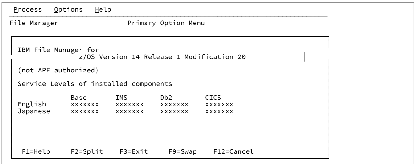
Figure 5. File Manager Primary Option Menu panel with example PTF information
