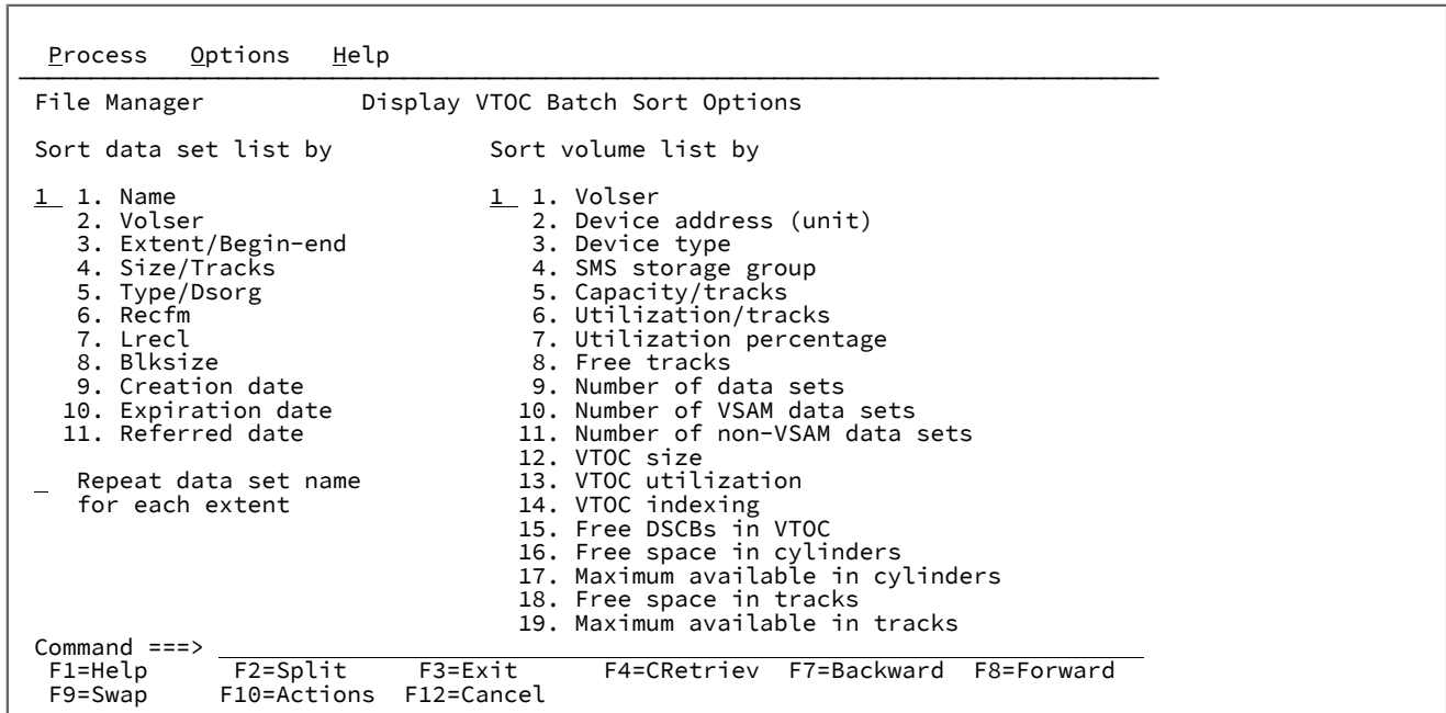
Figure 226. Display VTOC Batch Sort Options panel
