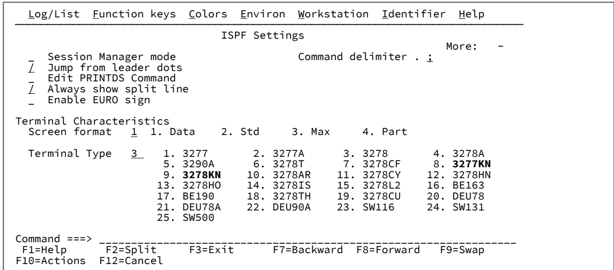
Figure 22. ISPF Settings panel
