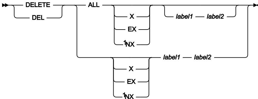
Figure 373. Syntax (CHAR, HEX, LHEX or TABL display format)
