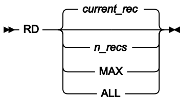
Figure 395. Syntax - View and Edit
