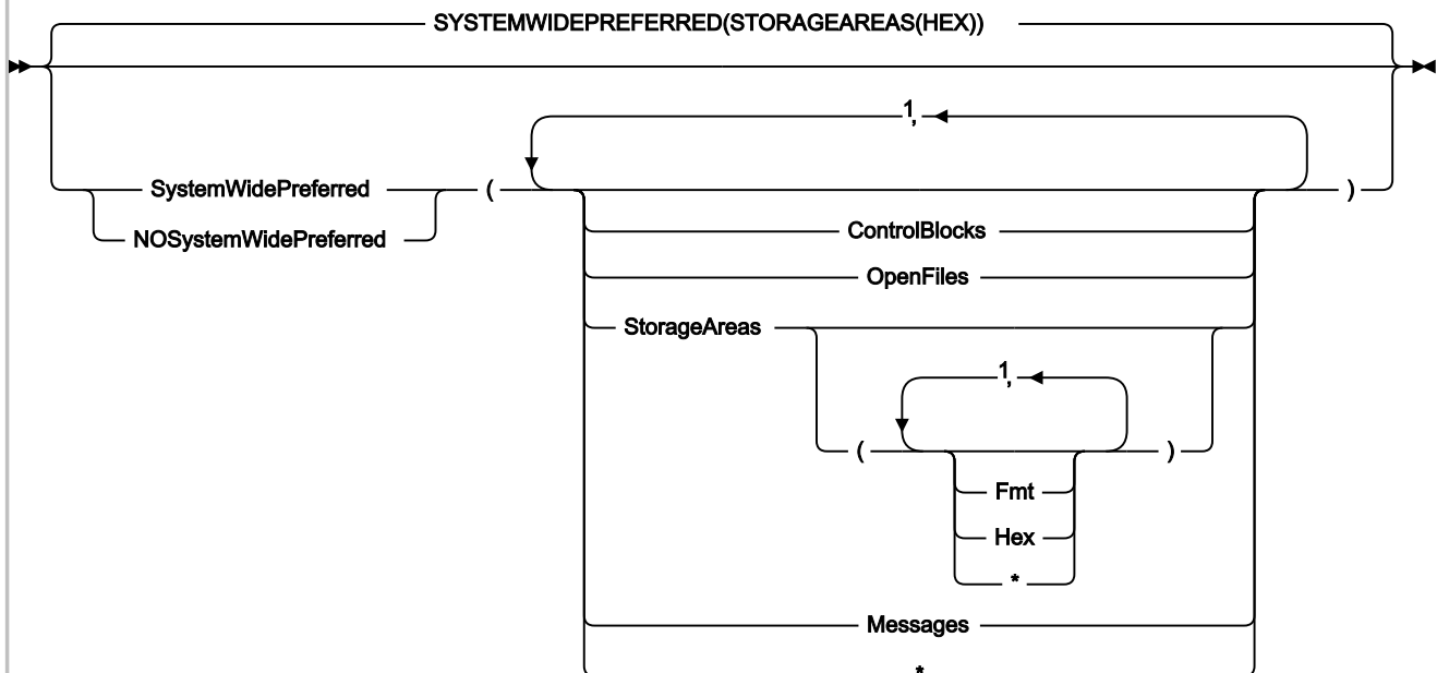
Figure 338. Syntax
