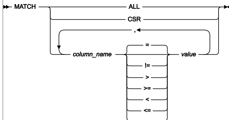
Figure 21. Syntax
