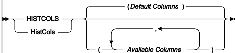
Figure 309. Syntax
