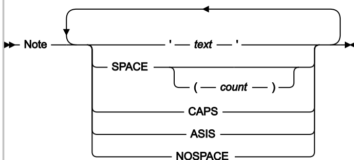
Figure 268. Syntax
