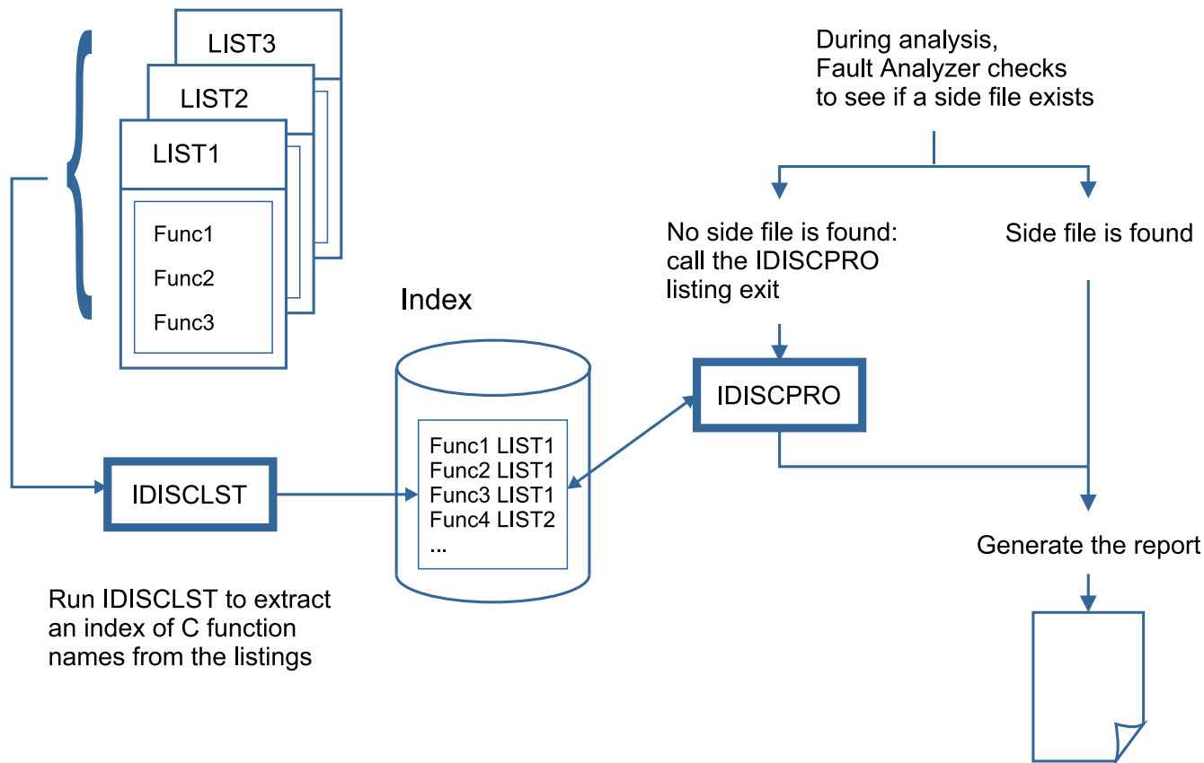
Figure 199. Extracting function names from C programs that were not compiled with #pragma csect
