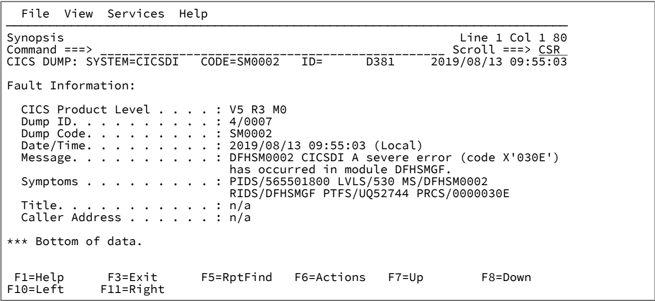
Figure 168. Sample CICS System Abend Synopsis display
