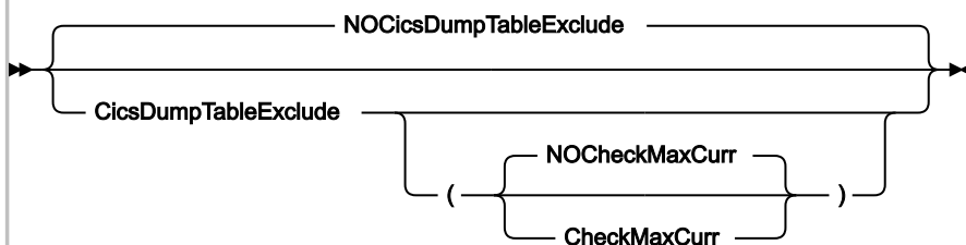
Figure 291. Syntax
