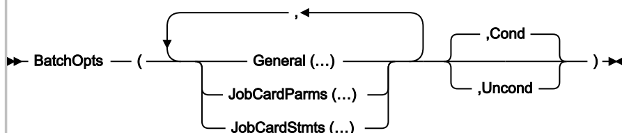
Figure 60. Syntax
