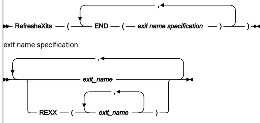
Figure 330. Syntax
