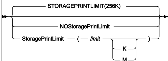
Figure 336. Syntax
