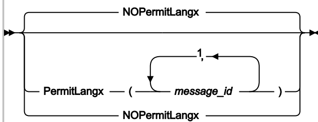
Figure 326. Syntax
