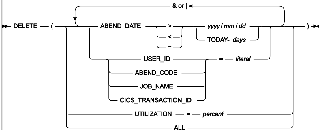
Figure 214. Syntax
