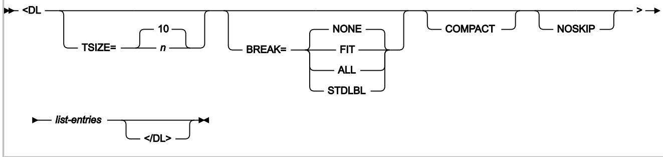
Figure 276. Syntax
