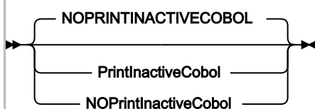
Figure 328. Syntax
