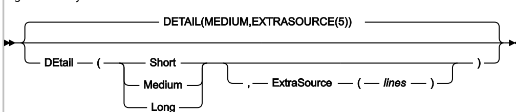
Figure 296. Syntax
