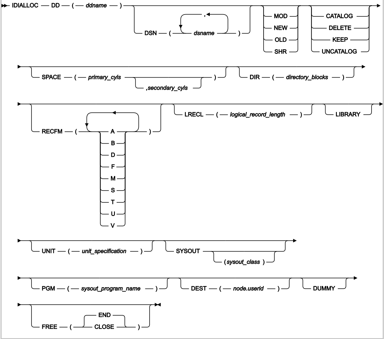
Figure 244. Syntax
