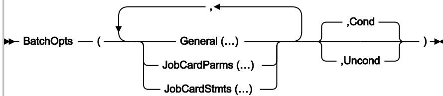
Figure 304. Syntax
