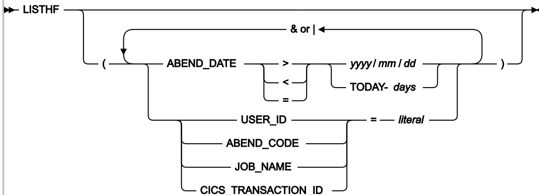
Figure 212. Syntax
