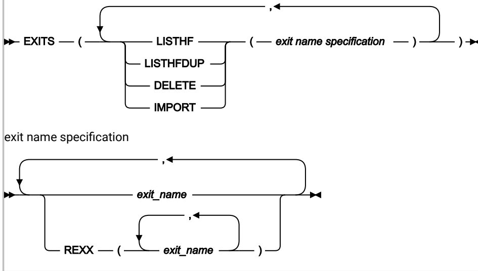
Figure 220. Syntax
