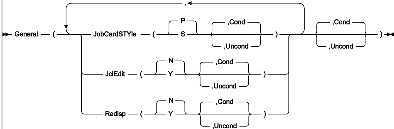
Figure 305. Syntax
