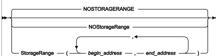
Figure 337. Syntax
