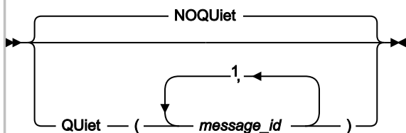
Figure 329. Syntax
