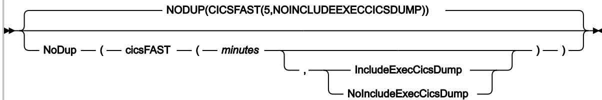
Figure 322. Syntax
