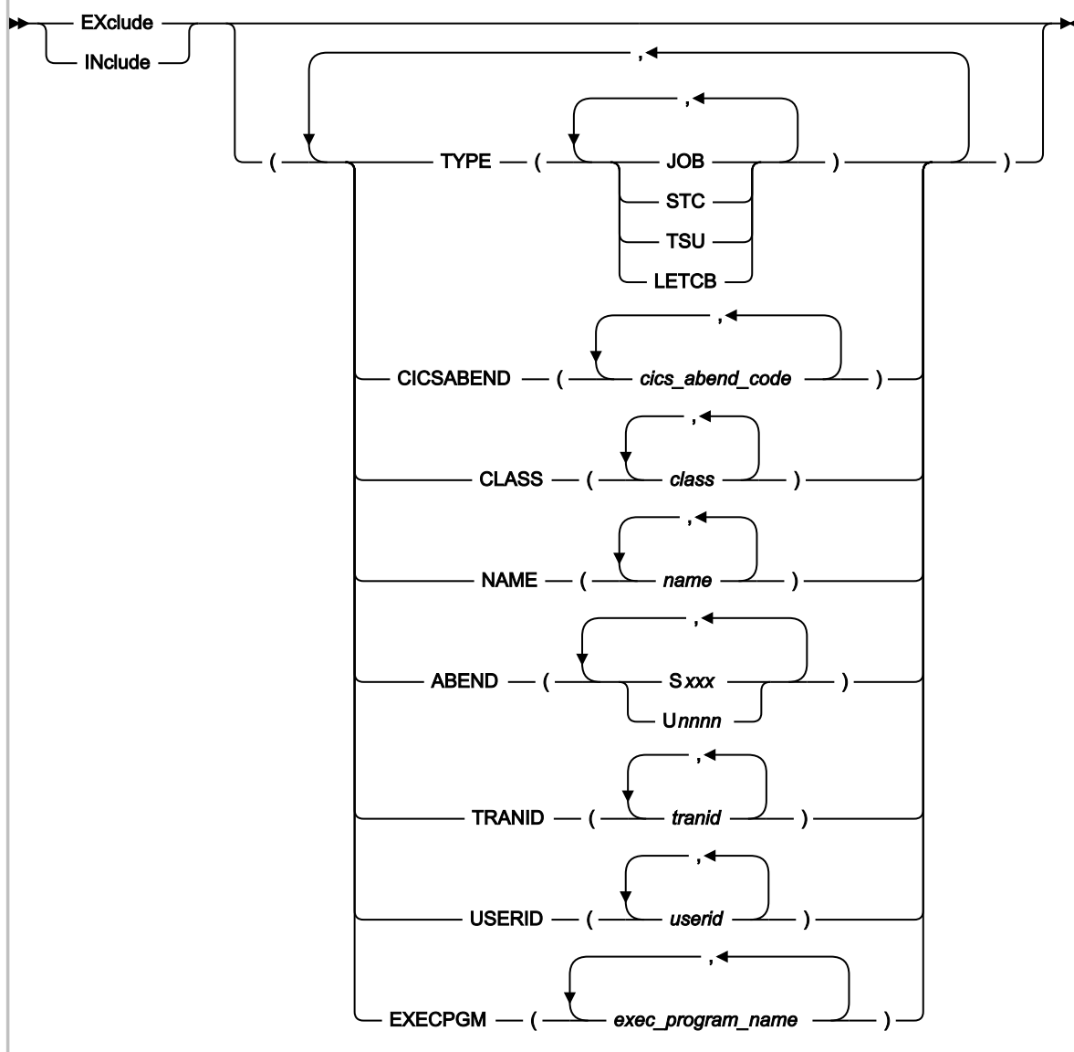
Figure 300. Syntax
