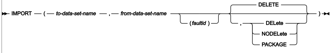
Figure 218. Syntax
