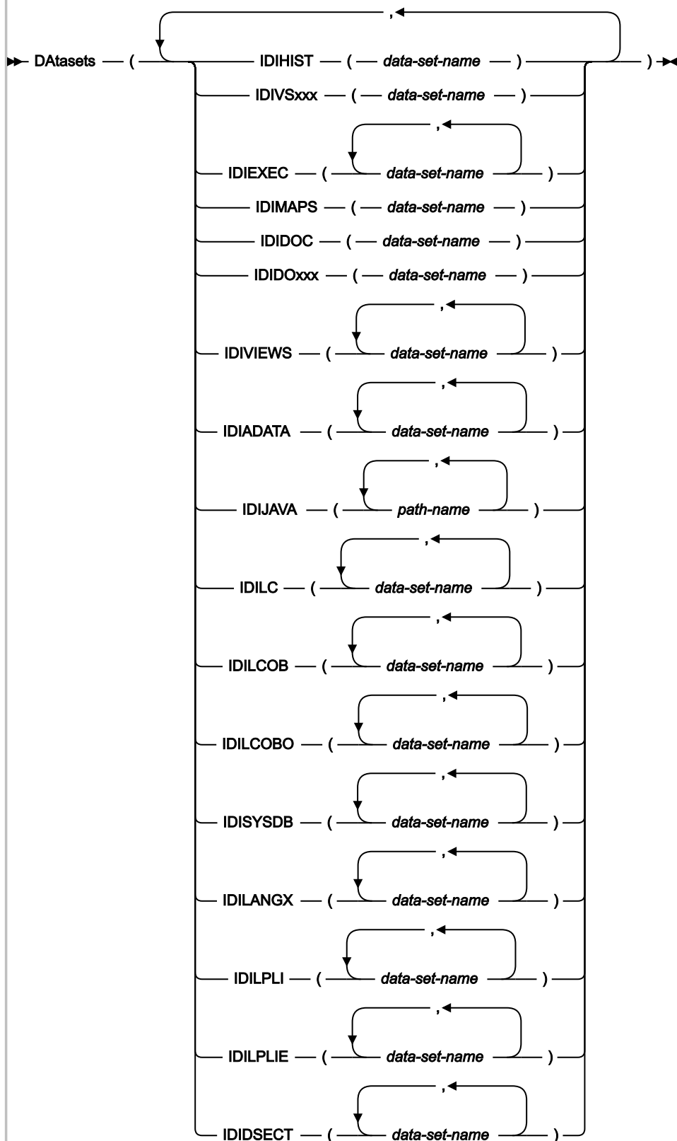
Figure 293. Syntax
