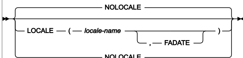
Figure 317. Syntax
