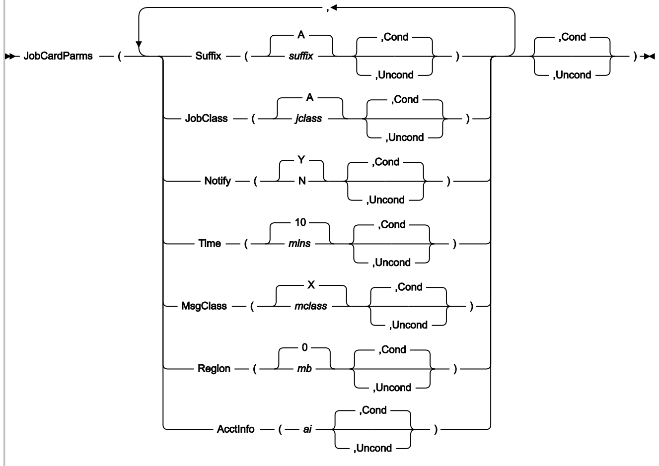
Figure 306. Syntax
