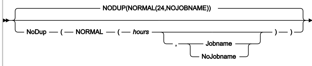
Figure 324. Syntax
