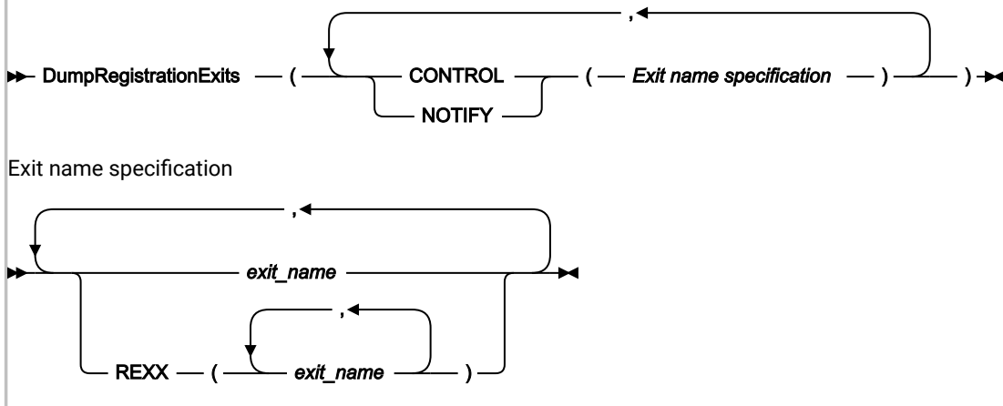
Figure 298. Syntax
