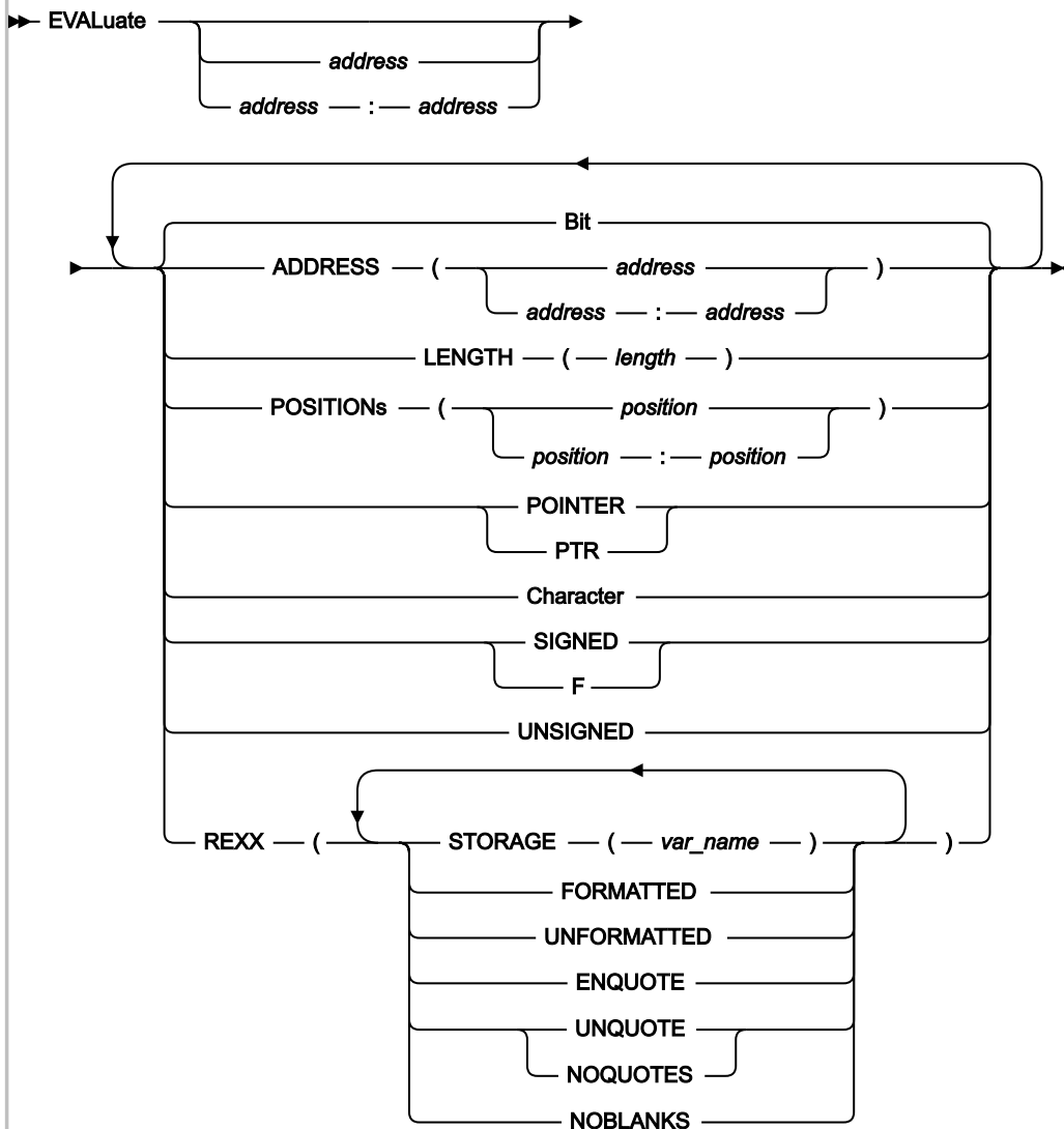
Figure 242. Syntax
