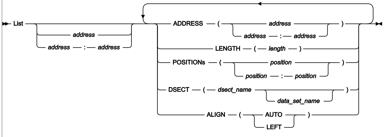
Figure 266. Syntax
