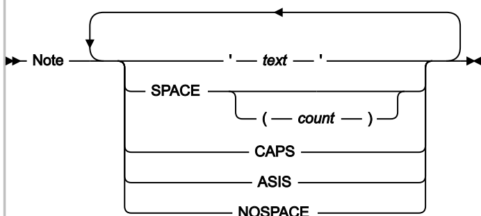
Figure 267. Syntax
