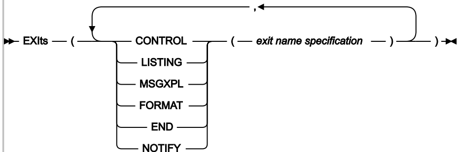
Figure 301. Syntax
