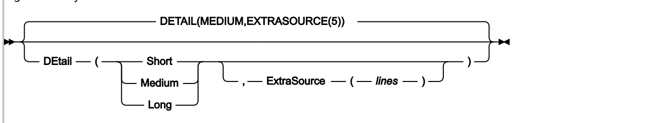
Figure 295. Syntax
