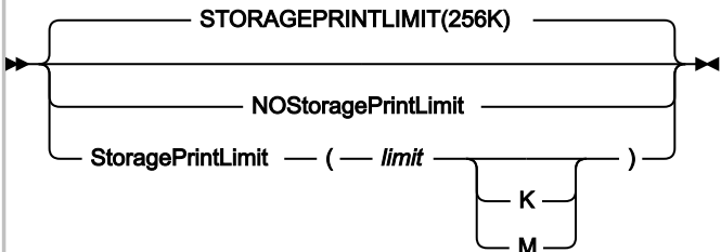
Figure 335. Syntax
