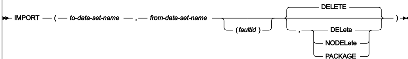
Figure 217. Syntax
