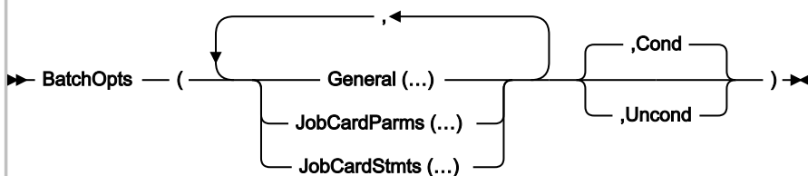
Figure 60. Syntax
