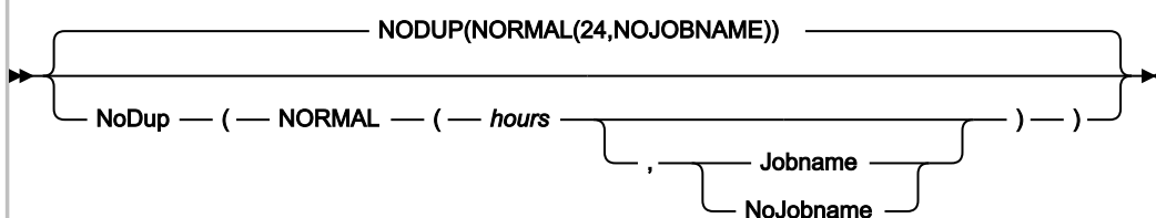
Figure 323. Syntax
