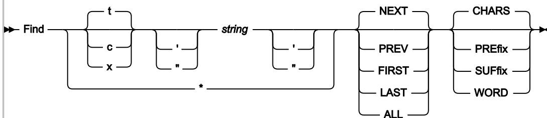
Figure 39. Syntax
