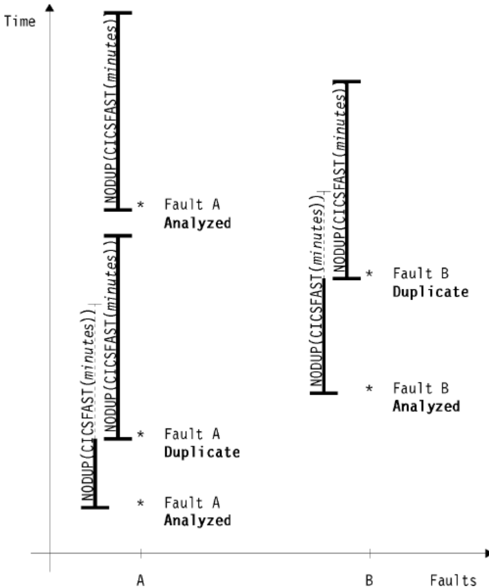
Figure 322. NoDup(CICSFAST) illustration
