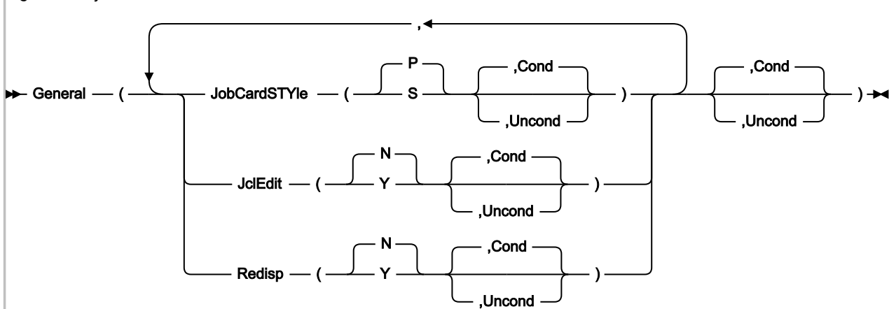
Figure 61. Syntax
