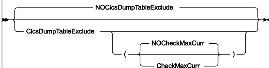
Figure 290. Syntax
