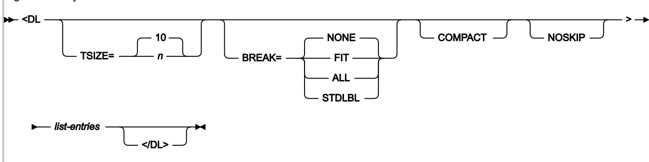
Figure 275. Syntax
