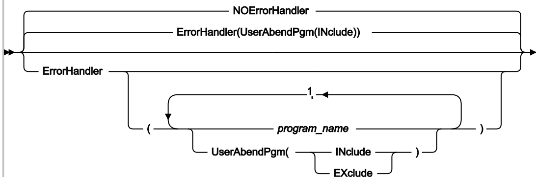
Figure 298. Syntax
