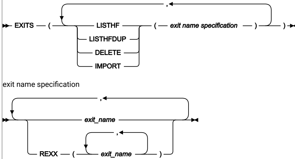
Figure 219. Syntax
