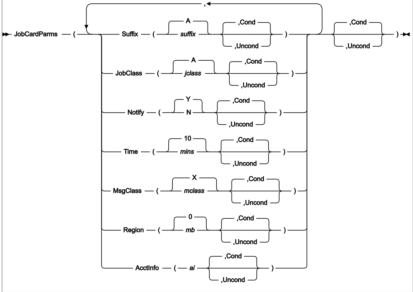
Figure 62. Syntax
