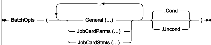
Figure 303. Syntax
