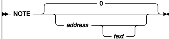
Figure 45. Syntax
