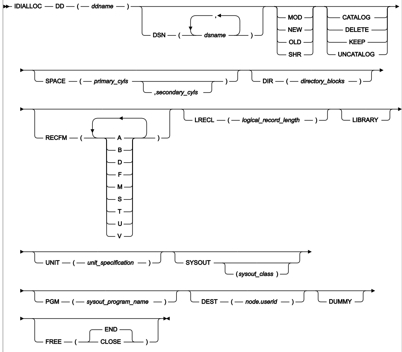
Figure 243. Syntax
