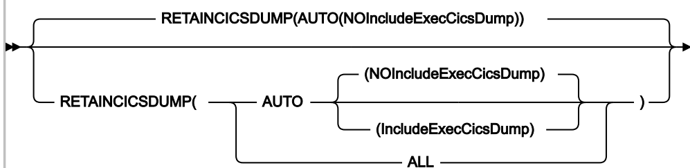
Figure 330. Syntax
