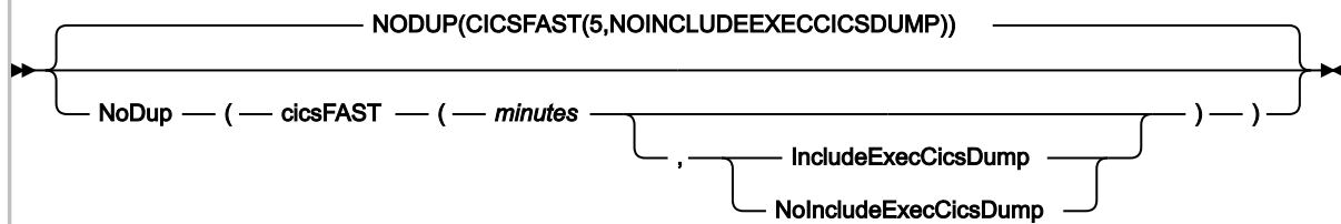
Figure 321. Syntax
