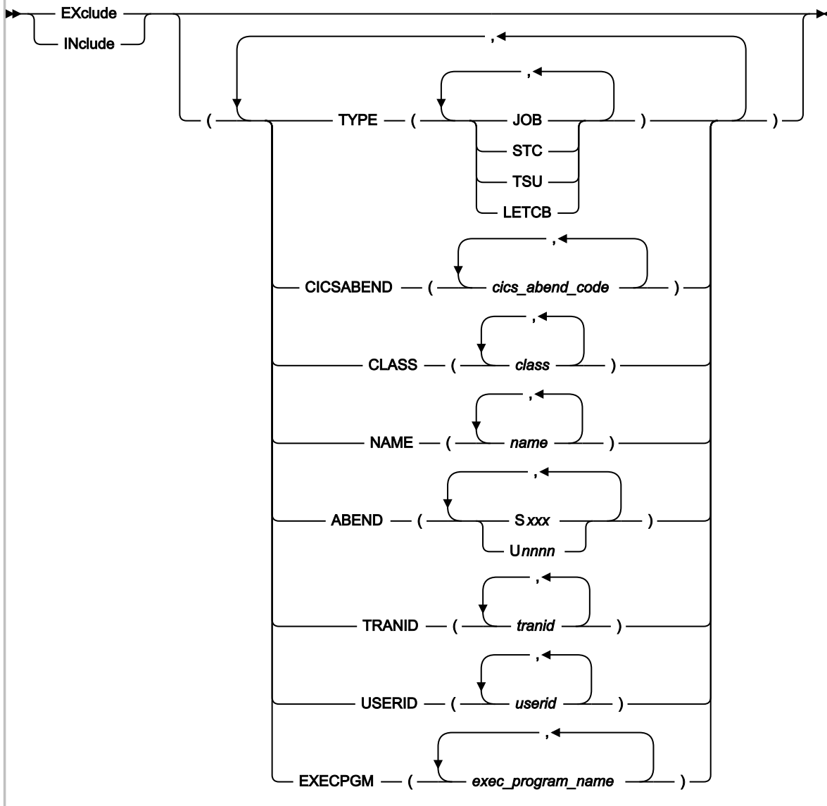
Figure 299. Syntax
