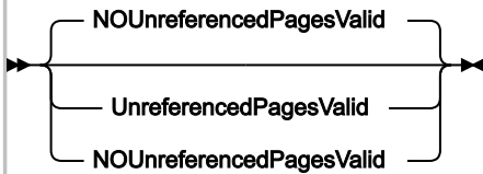
Figure 339. Syntax
