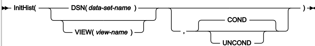
Figure 309. Syntax
