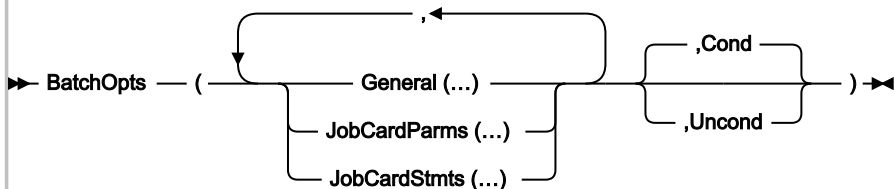
Figure 303. Syntax
