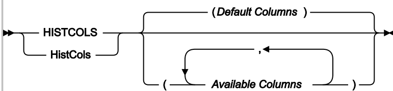
Figure 308. Syntax
