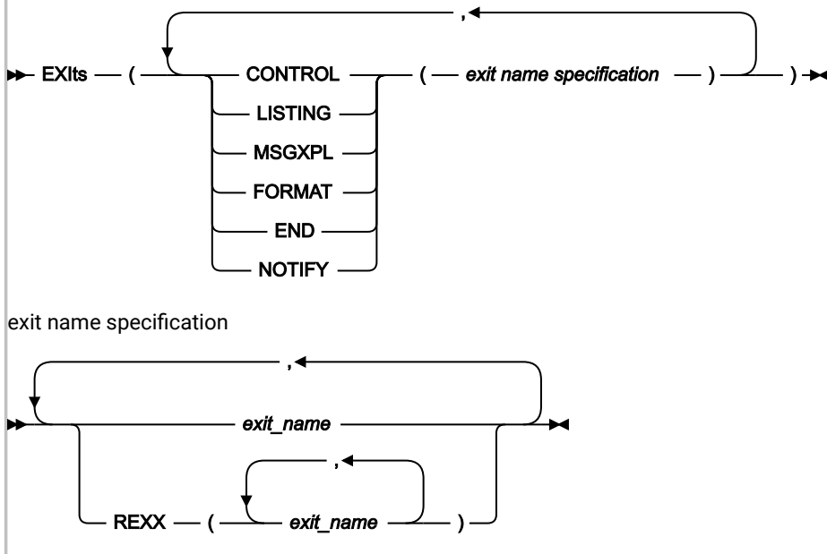
Figure 301. Syntax
