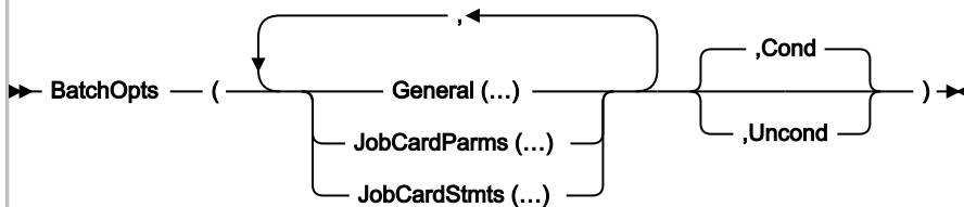
Figure 60. Syntax
