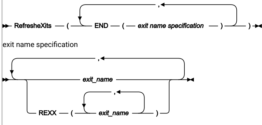
Figure 329. Syntax
