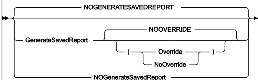
Figure 312. Syntax
