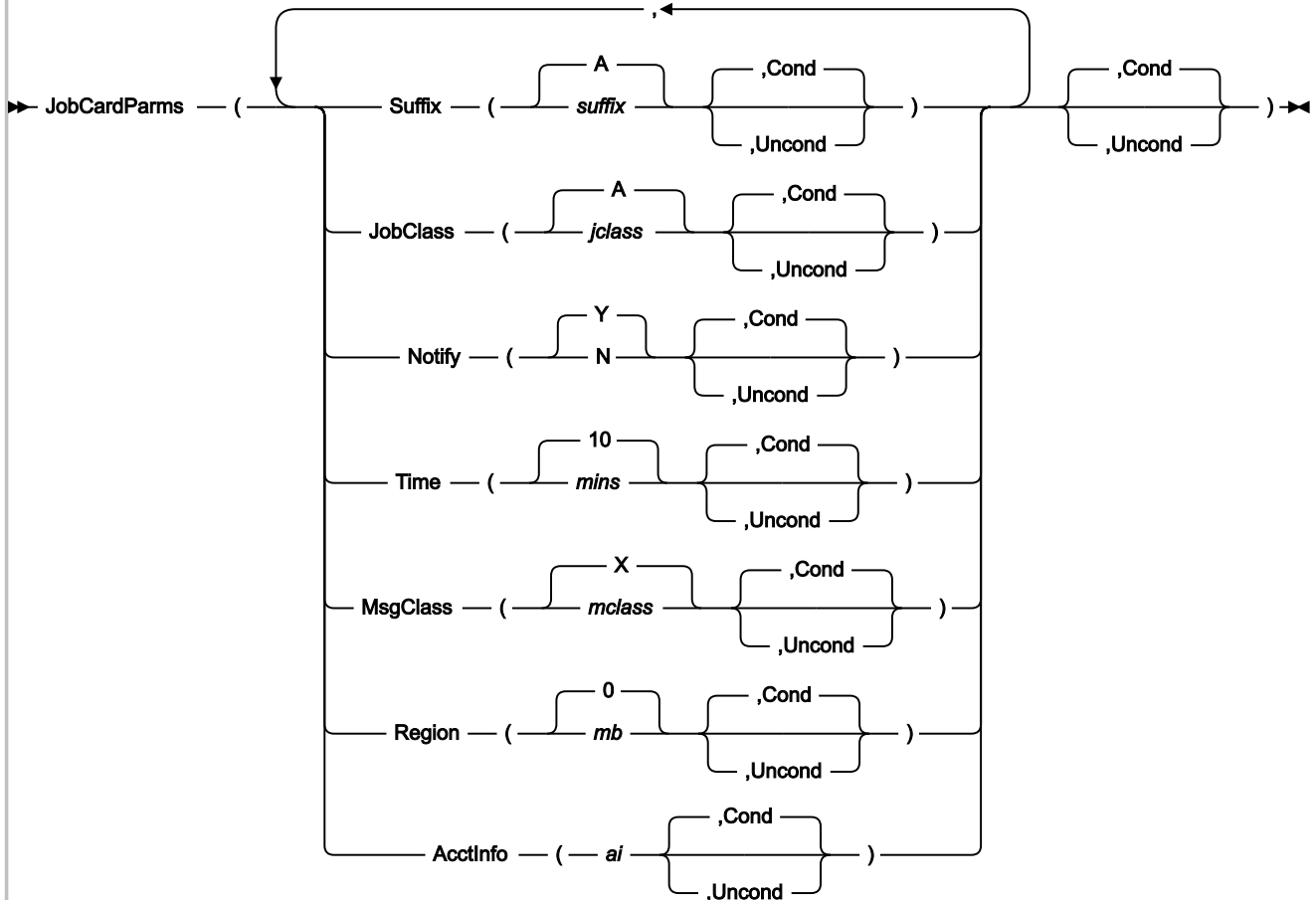
Figure 62. Syntax
