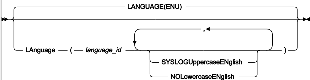
Figure 314. Syntax
