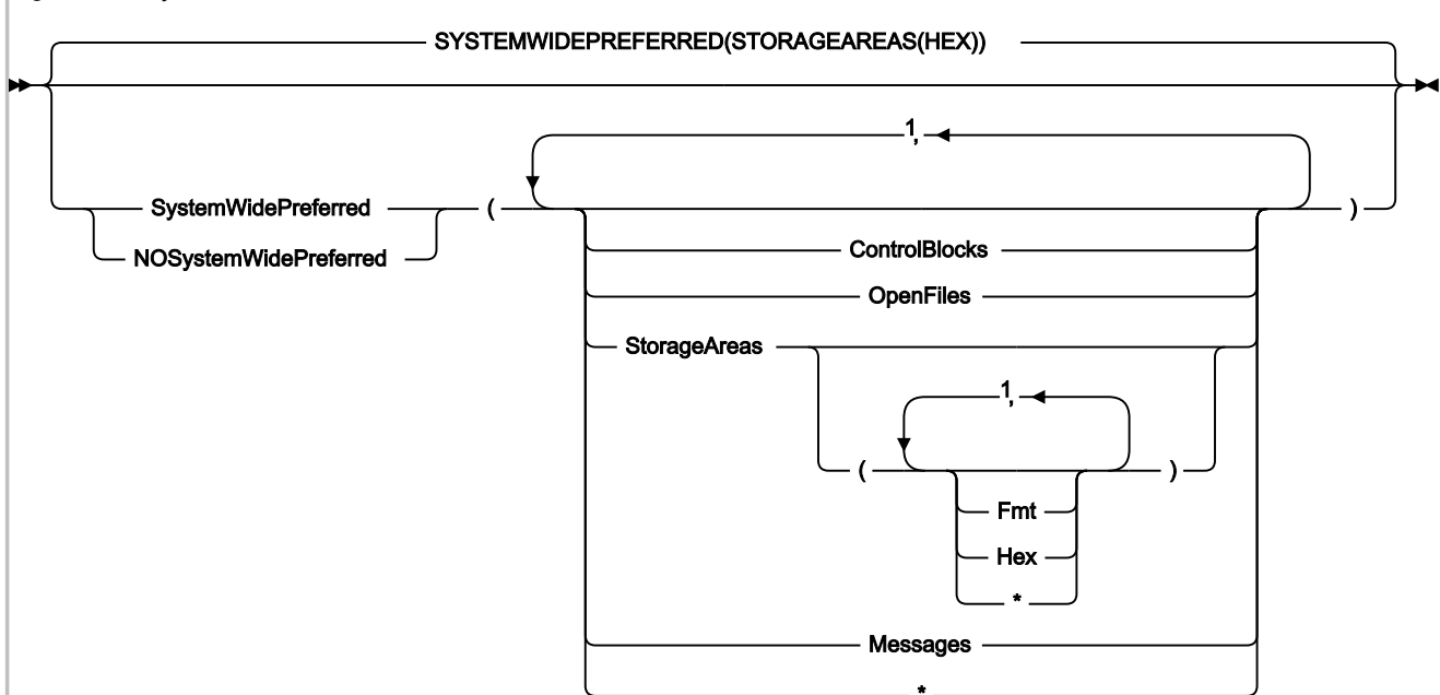
Figure 337. Syntax
