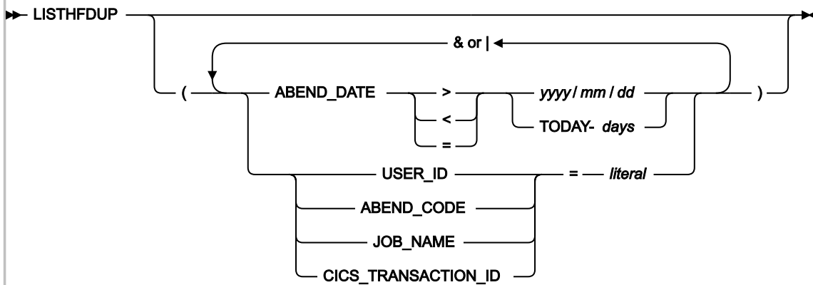
Figure 212. Syntax
