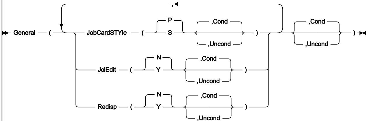
Figure 61. Syntax
