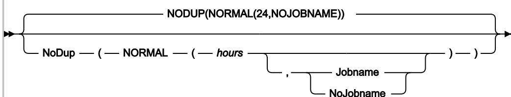
Figure 323. Syntax
