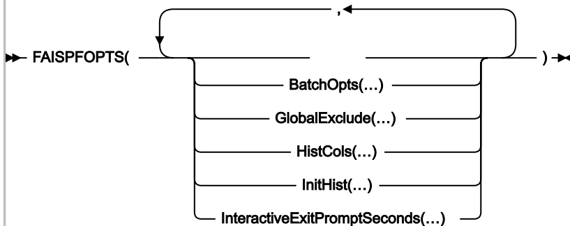
Figure 302. Syntax
