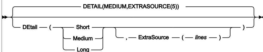
Figure 295. Syntax
