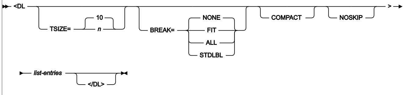
Figure 275. Syntax
