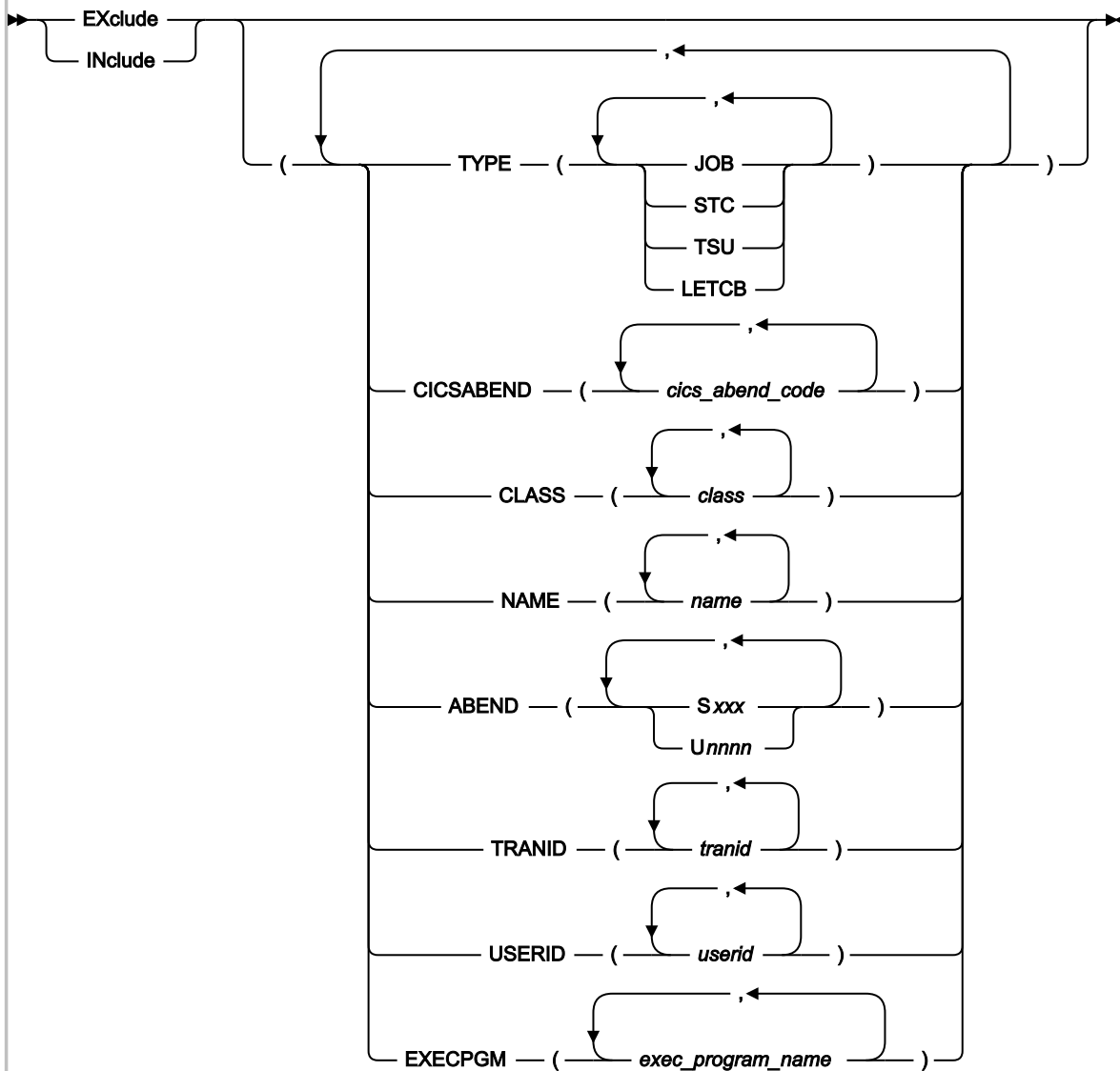
Figure 299. Syntax
