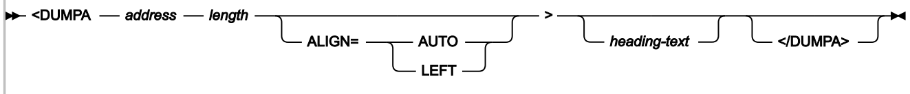
Figure 278. Syntax
