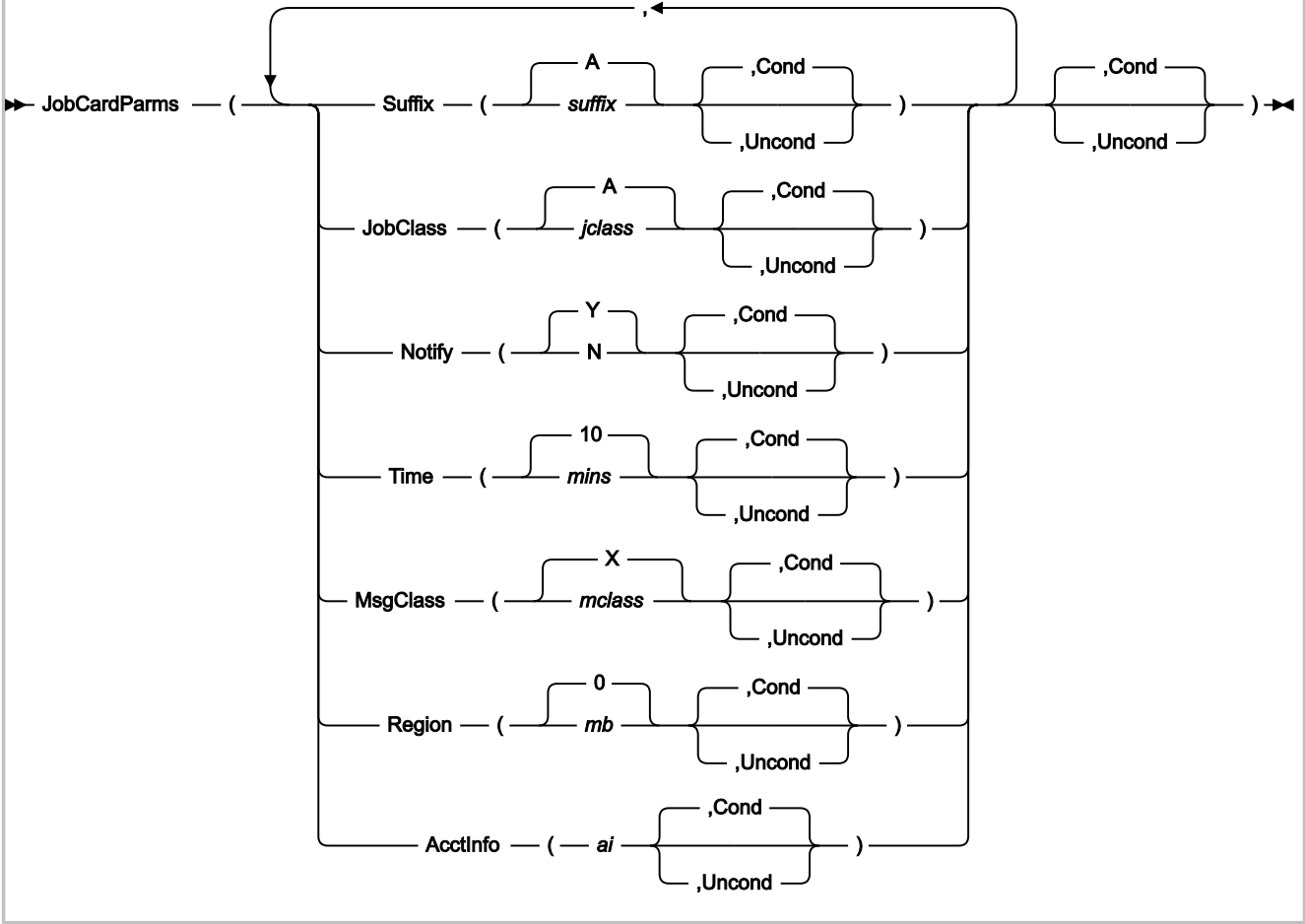
Figure 305. Syntax
