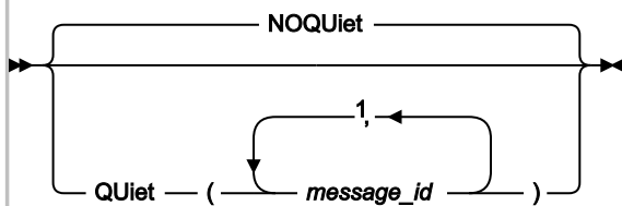
Figure 328. Syntax
