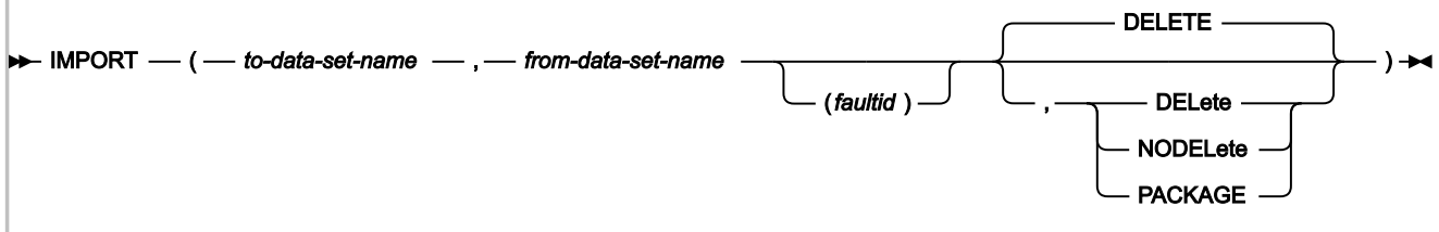
Figure 217. Syntax
