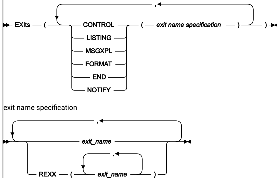
Figure 301. Syntax
