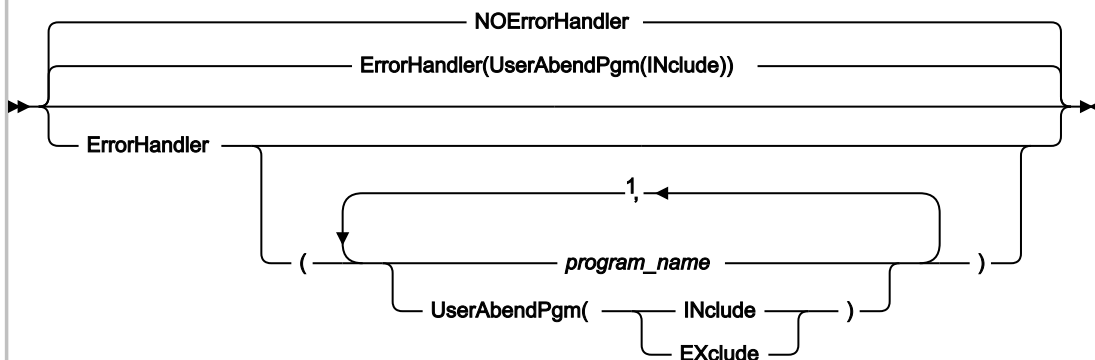
Figure 298. Syntax
