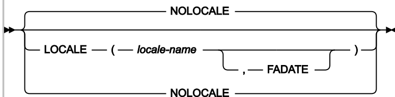
Figure 316. Syntax
