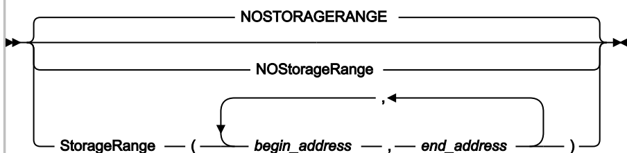
Figure 336. Syntax
