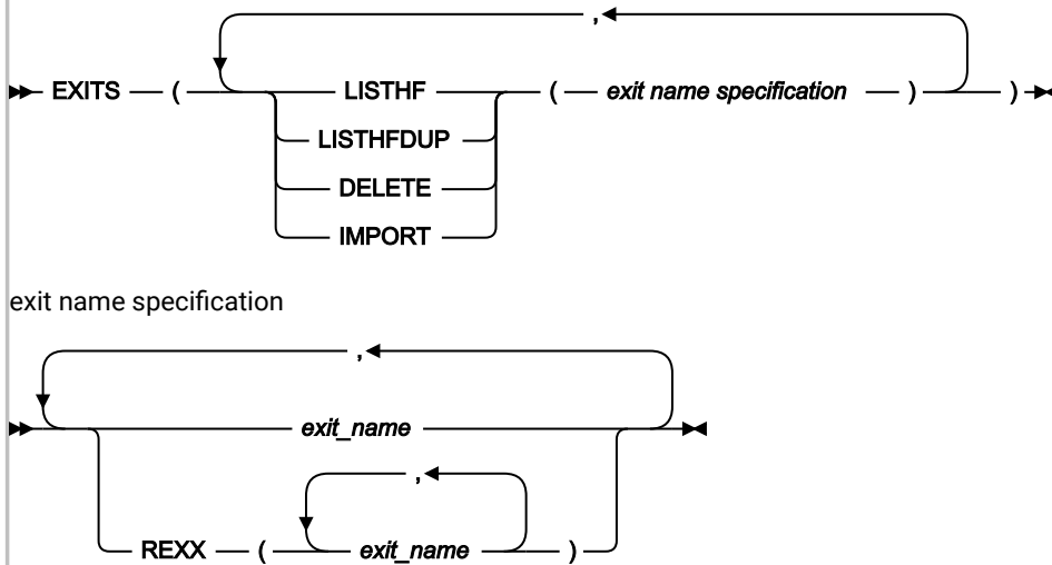
Figure 219. Syntax
