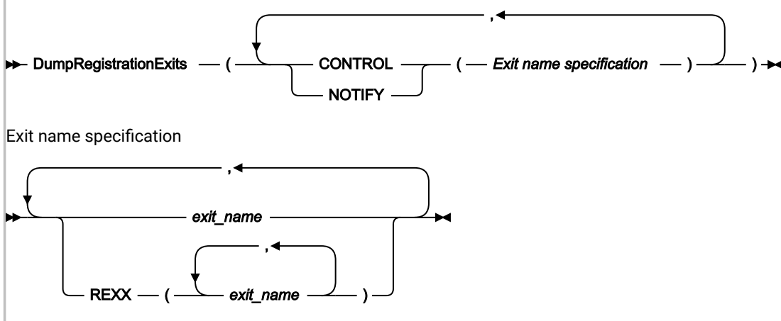
Figure 297. Syntax
