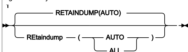
Figure 331. Syntax
