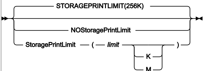
Figure 335. Syntax
