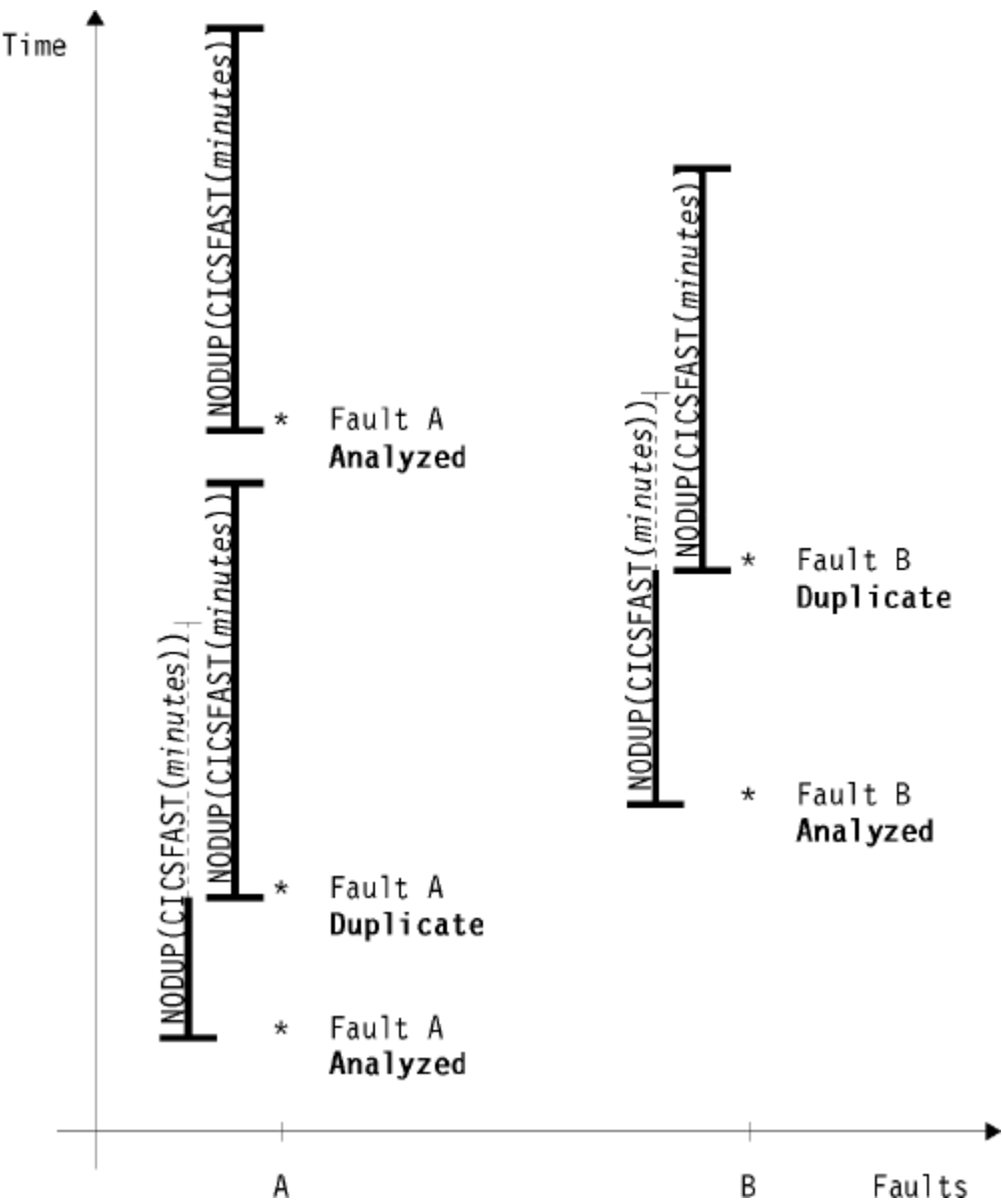
Figure 322. NoDup(CICSFAST) illustration
