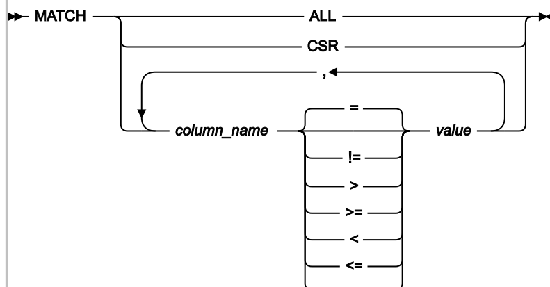
Figure 21. Syntax
