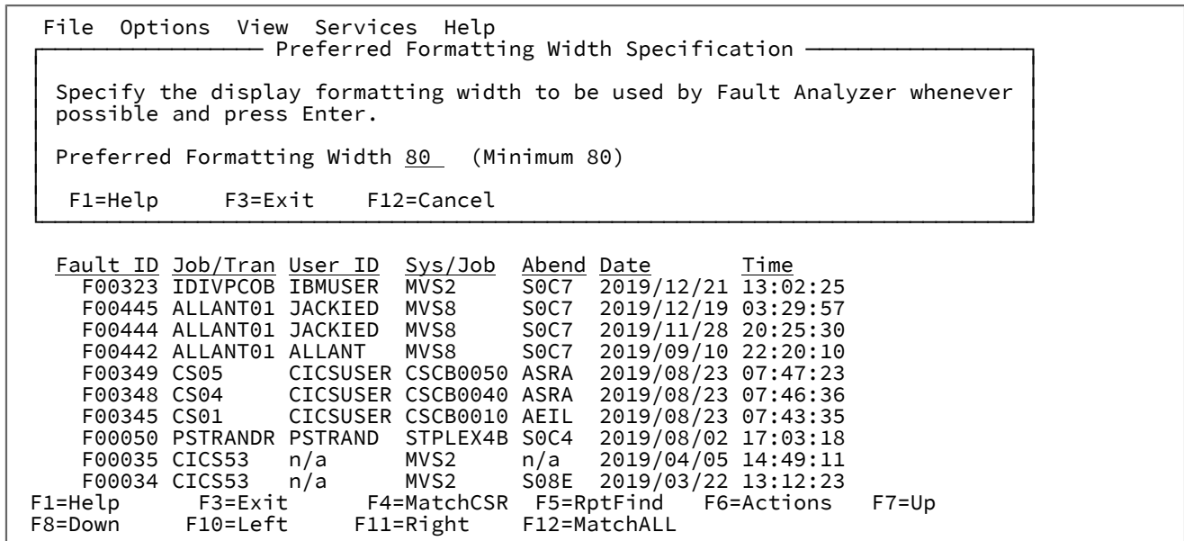
Figure 66. Sample Preferred Formatting Width display
