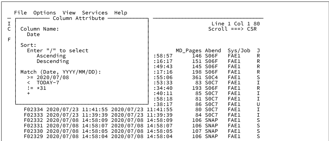
Figure 19. Sample Column Attributes display specifying multiple matching criteria
