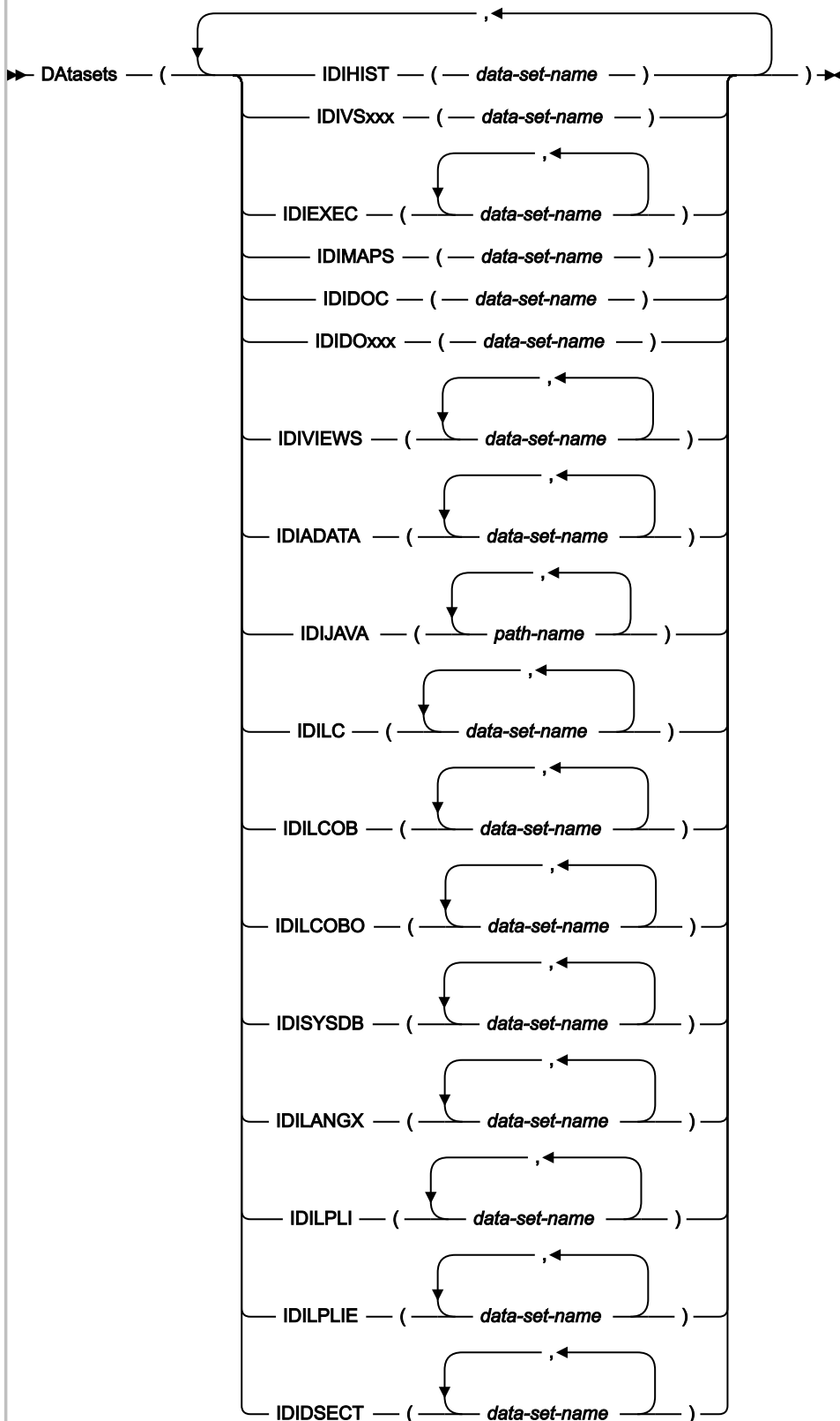
Figure 290. Syntax
