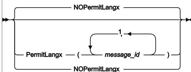
Figure 324. Syntax
