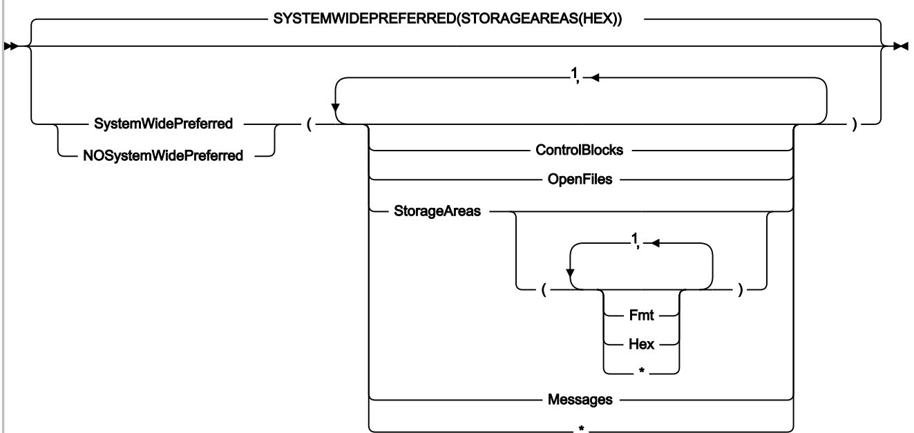
Figure 336. Syntax
