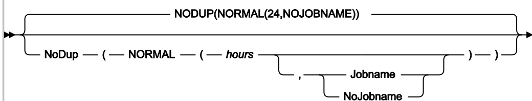
Figure 321. Syntax
