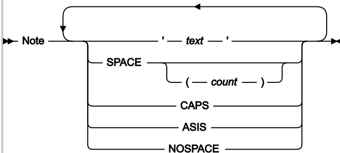
Figure 265. Syntax
