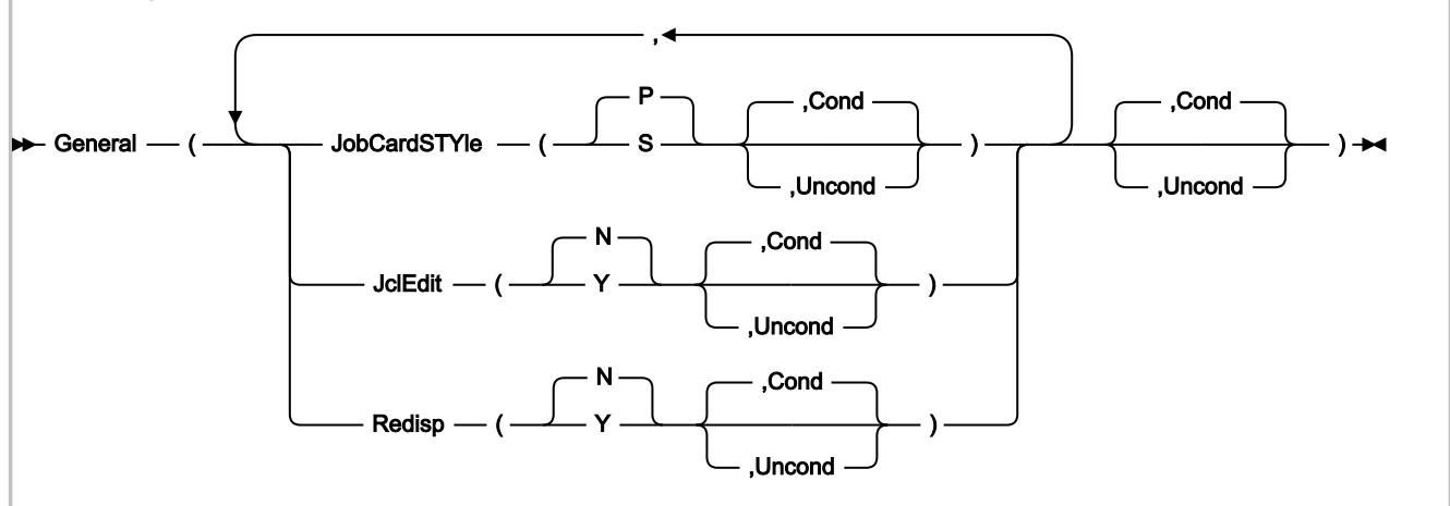
Figure 62. Syntax
