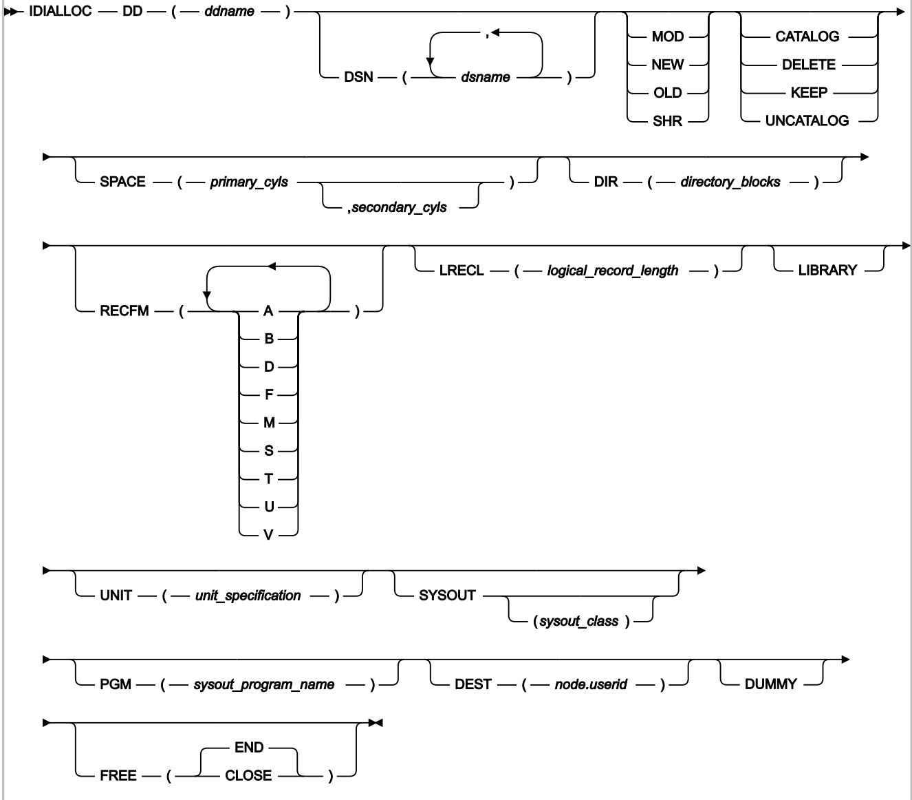
Figure 241. Syntax
