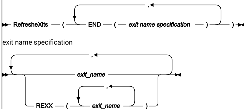
Figure 328. Syntax
