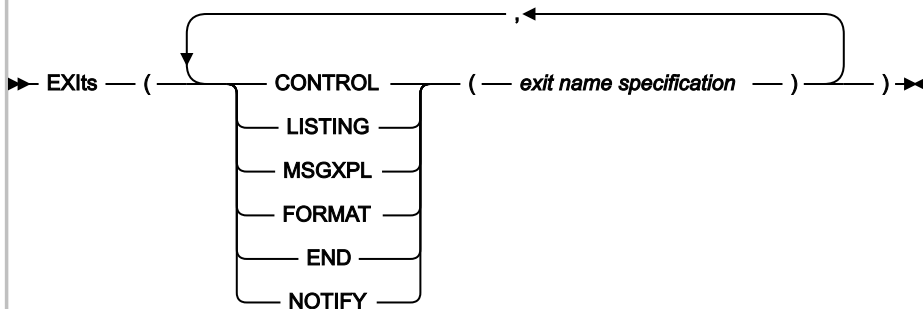
Figure 299. Syntax
