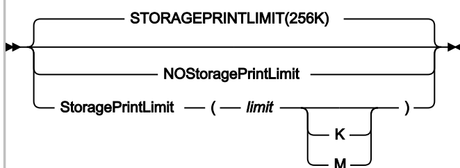
Figure 334. Syntax
