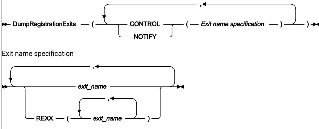
Figure 295. Syntax
