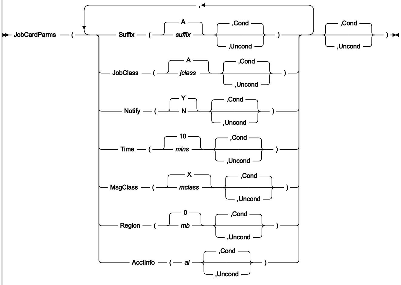
Figure 303. Syntax
