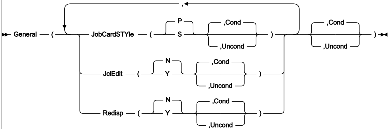
Figure 302. Syntax
