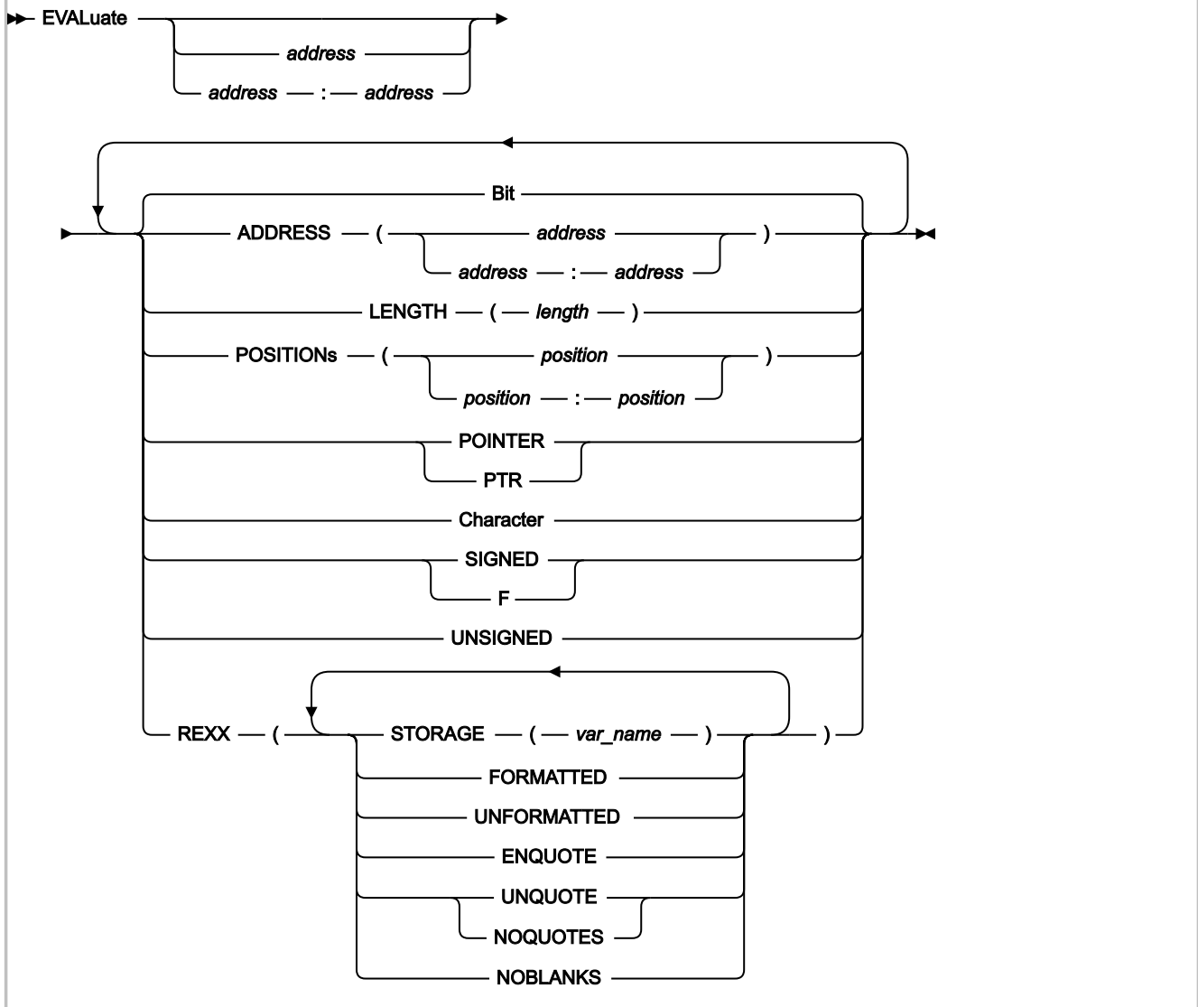
Figure 239. Syntax
