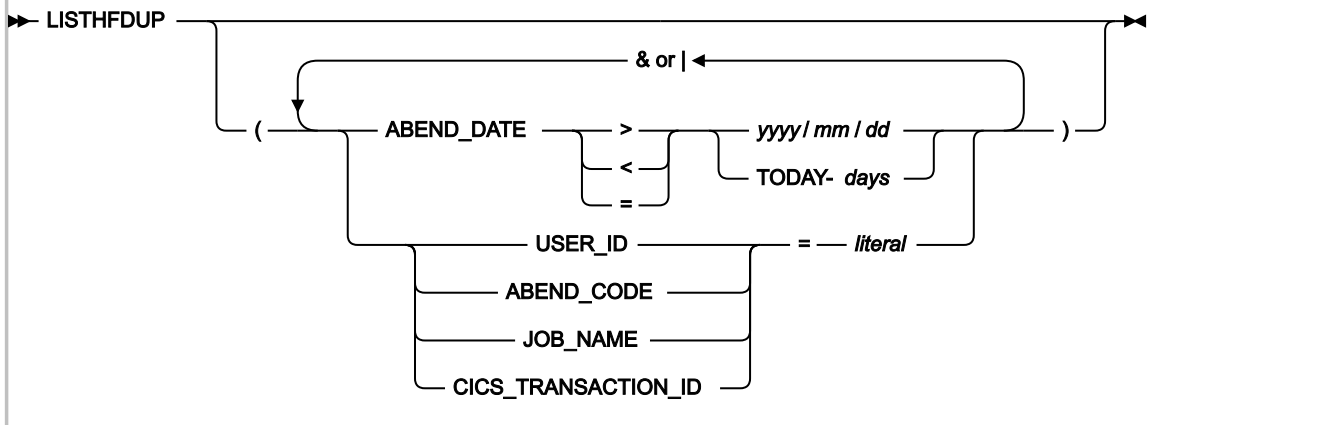
Figure 210. Syntax
