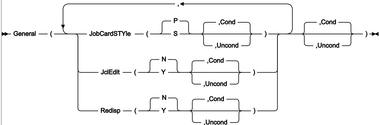
Figure 62. Syntax
