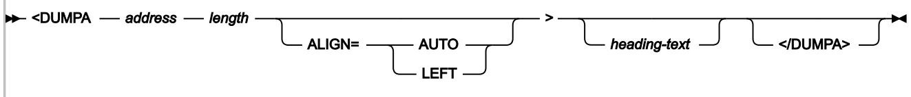
Figure 276. Syntax
