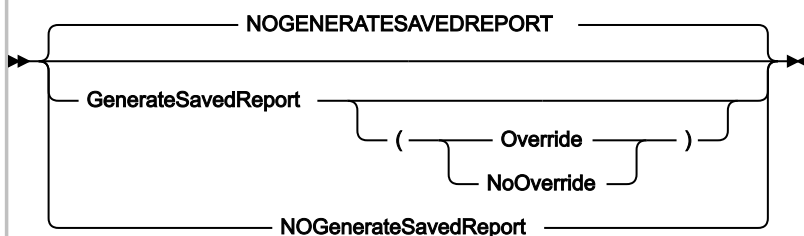
Figure 310. Syntax
