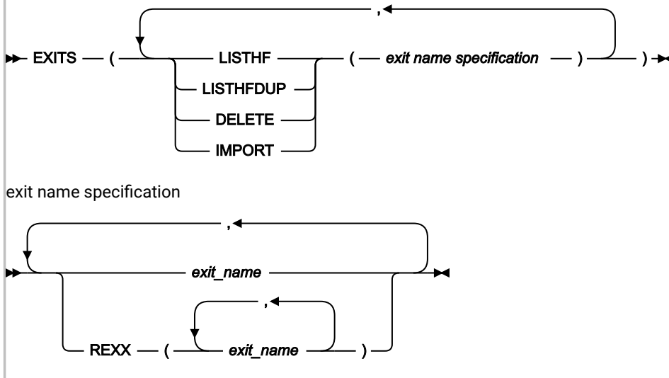
Figure 217. Syntax
