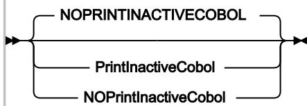
Figure 326. Syntax
