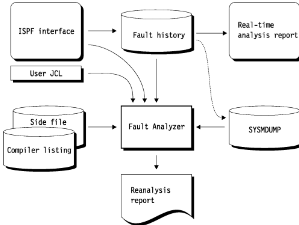
Figure 5. Reanalysis
