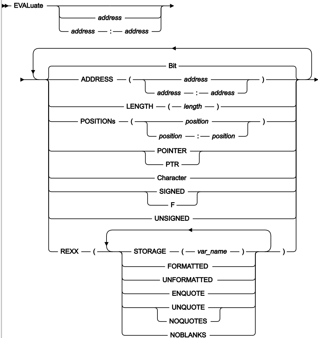
Figure 239. Syntax
