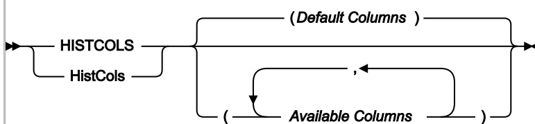
Figure 306. Syntax
