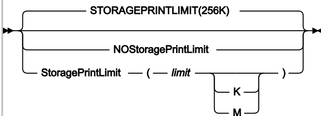
Figure 334. Syntax
