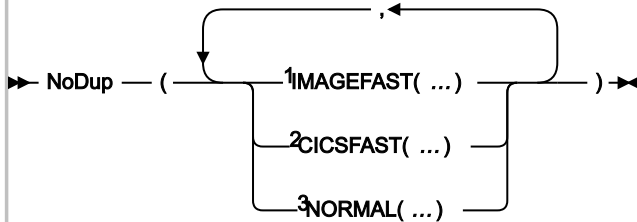
Figure 317. Syntax
