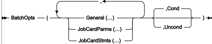
Figure 301. Syntax
