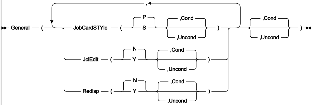
Figure 62. Syntax
