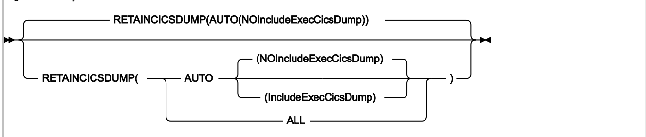
Figure 329. Syntax
