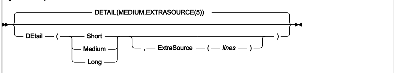
Figure 293. Syntax
