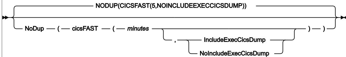
Figure 319. Syntax
